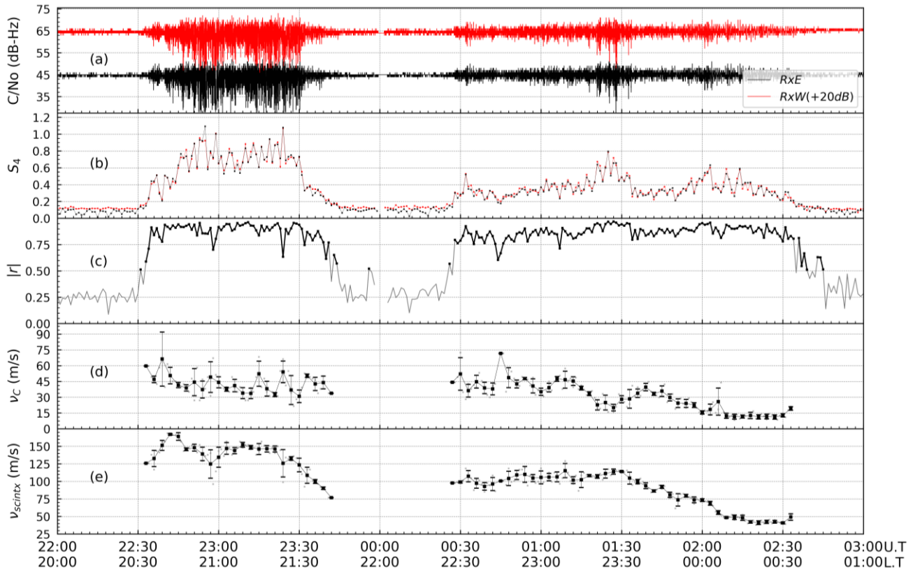
255 Figure 3 - Example of measurements and analyses made with closely spaced ScintPi 3.0 monitors at UFCG for the same night of Fig. 2 (October 4-5, 2022). (a) Signal strengths ( C/No ) in dB-Hz from L1 from PRN136. (b) Severity of scintillation, i.e., S_4 index. (c) Maximum value from the normalized cross correlation function, highlighted in black any value greater than 0.5. (d) Estimated mean characteristic velocities, (e) Estimated mean true scintillation pattern velocities. Error bars in panels (d) and (e) represent standard deviation around the mean of the values used in 3-minute bins.
