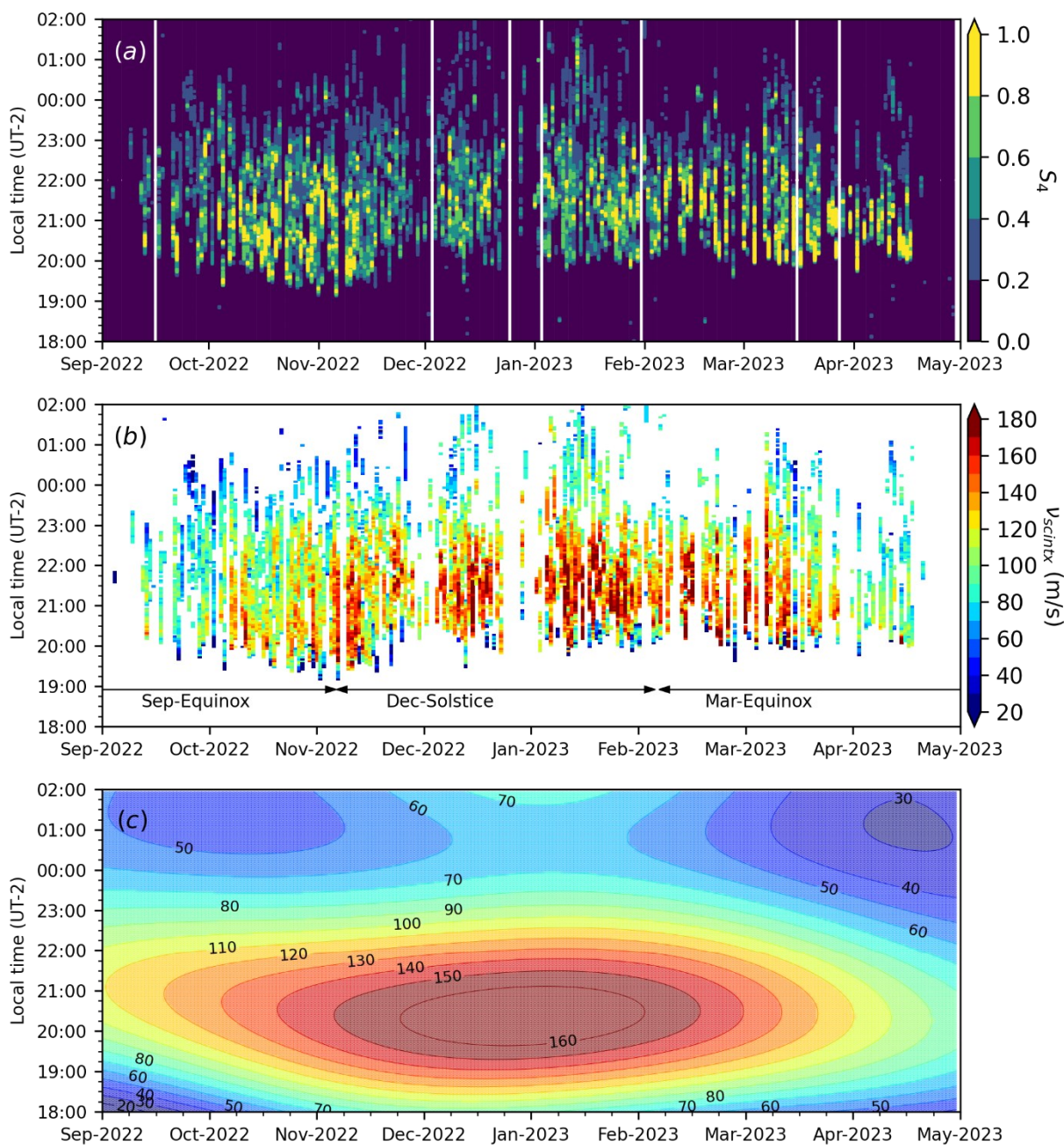
300 Figure 4 - Panel (a) shows the average S_4 index measurements as a function of local time ( LT = UT - 2 ) and date for 242 nights between September 1, 2022, and April 30, 2023. The average is for the two S_4 values computed by the spaced monitors. White lines indicate lack of data caused by power outages at the observation sites. Panel (b) shows zonal irregularity drifts. Different seasons determined as \pm 45 days around equinox and solstice days are also indicated. Panel (c) shows climatological zonal wind velocities ( U_z ) from the Horizontal Wind Model 14 (HWM14) for a height of 450 km over UFCG, its values magnitude values are indicated by labels of the contour lines.
