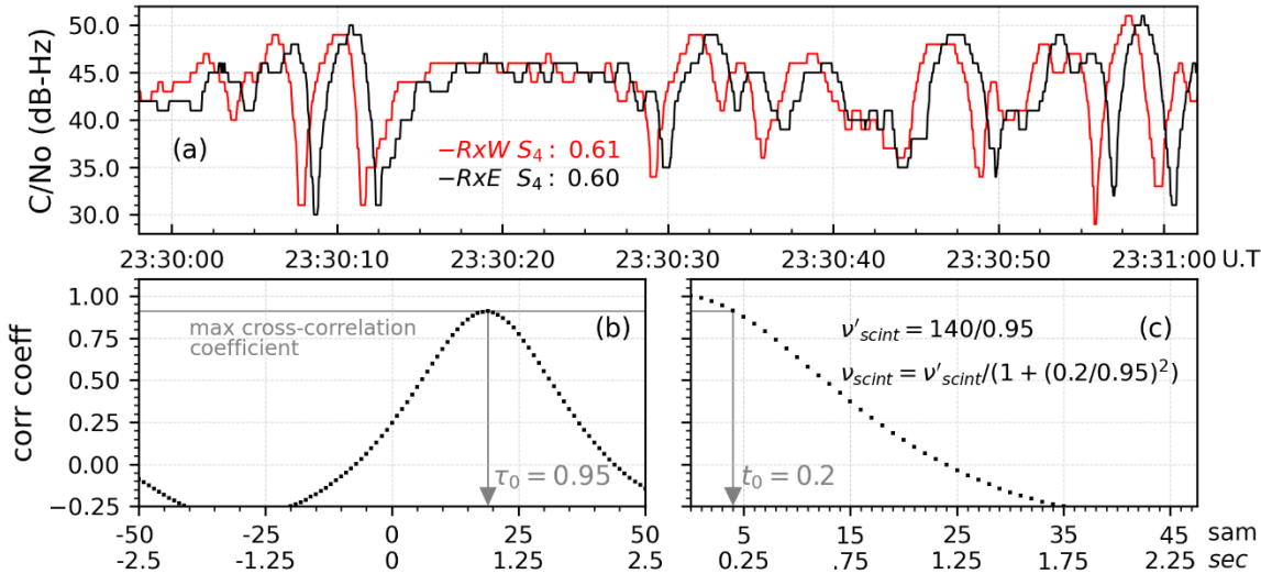
185 Figure 2 – Illustration of calculation used to derive the characteristic time ( t_0 ) and the time lag of maximum correlation ( \tau_0 ). Panel (a) shows an example of 60-second signal strength measurements made with closely spaced ScintPi 3.0 monitors on October 4, 2022. Panel (b) shows the cross-correlation function between power series from the two receivers, and panel (c) shows the autocorrelation for the west receiver. The maximum cross-correlation coefficient is used to estimate the characteristic time associated with the signal decorrelation. The horizontal axis in panels (b) and (c) show both sample number (samp) and time in seconds.
