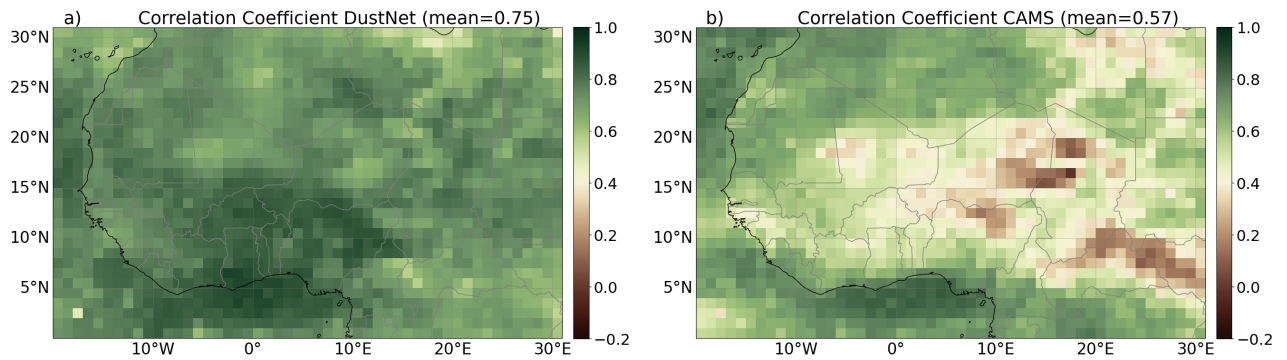
Figure 4. Daily correlation coefficients between MODIS AOD observations and model predictions are shown for a) DustNet and b) CAMS. The maximum correlation for DustNet is 0.82, with a minimum of 0.16, while the maximum correlation for CAMS is 0.75, with a minimum of -0.04. Values with weaker correlations ( \leq 0.4 ) are represented in white to brown shades, whereas stronger correlations ( >0.4 ) are depicted in green. The predominance of green shades, particularly over the Sahara region, highlights the advantage of DustNet predictions over CAMS
