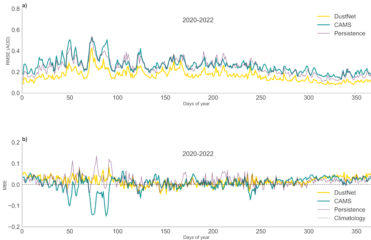
Figure B2. The top panel a) presents the study area mean RMSE calculated from daily AOD values predicted by DustNet (yellow), CAMS (cyan) and corresponding persistence (plum) are shown. At all time-steps the DustNet model predictions show smaller (better) errors than those produced by CAMS and persistence. The lower panel b) shows the temporal mean bias errors (MBE) from the DustNet predictions (yellow), CAMS (cyan) and persistence (plum). Here, the DustNet bias fluctuates close to zero more often than the bias produced by CAMS and persistence.
