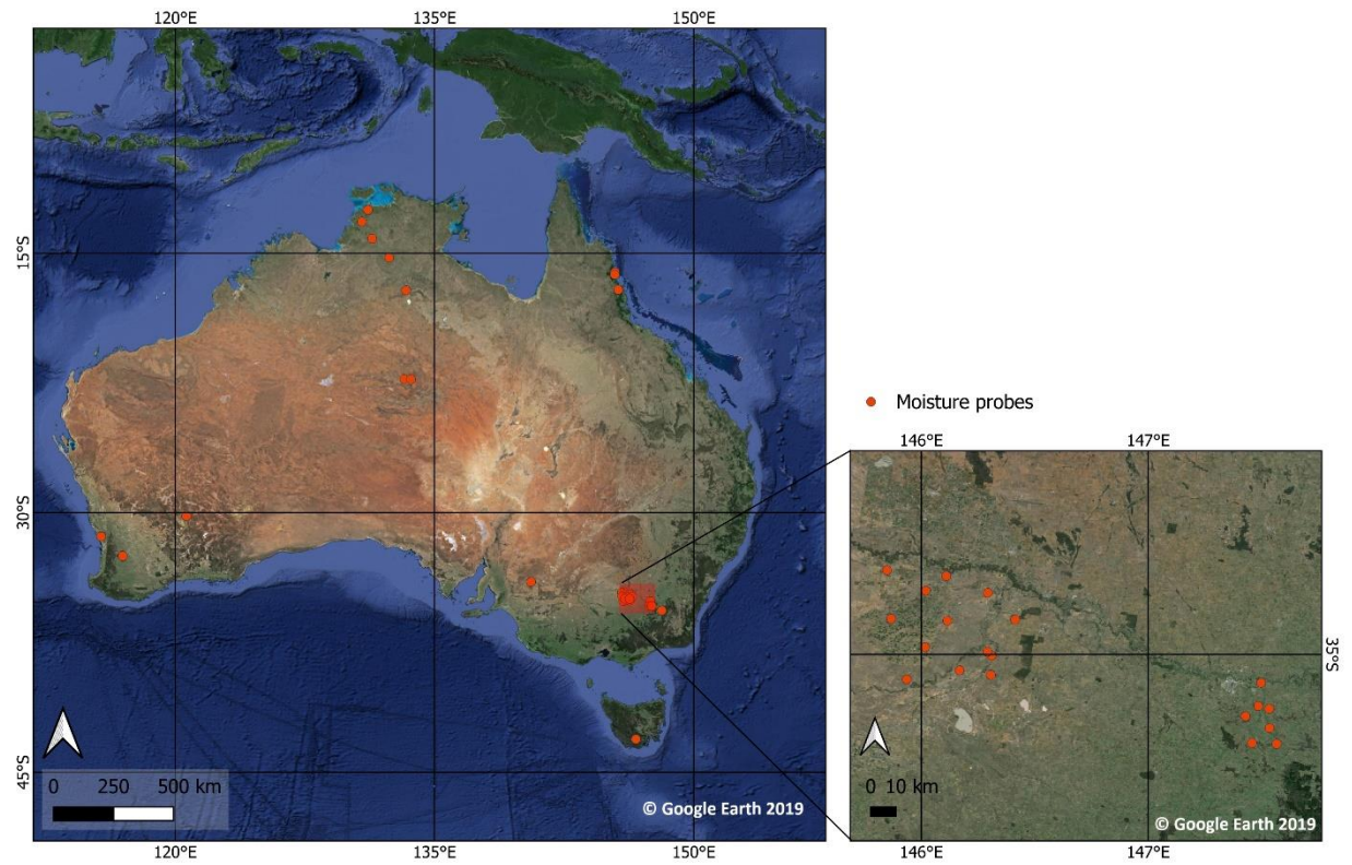
Figure S1: Location of soil moisture monitoring stations in Australia.
