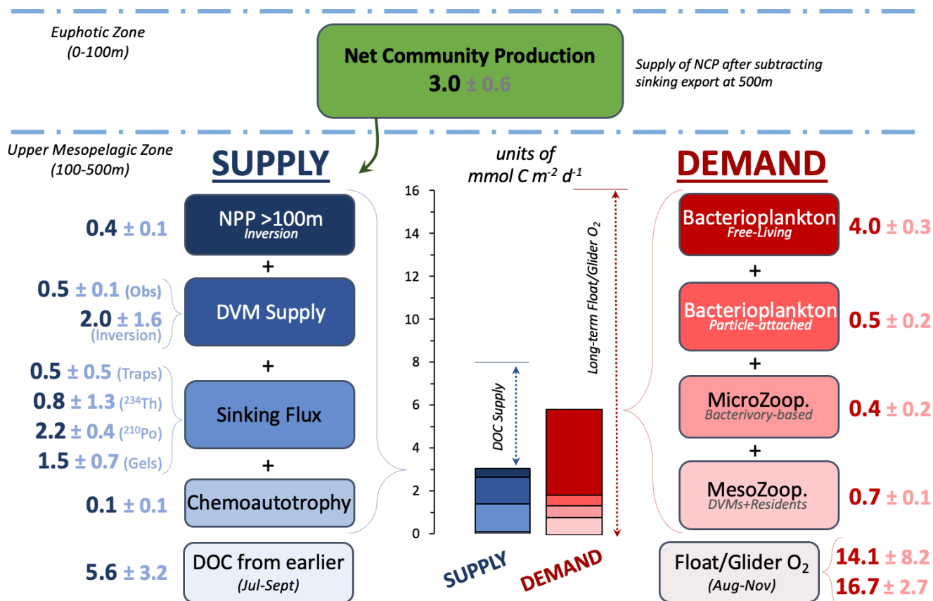
Figure 4: Comparison of organic C supply and demand estimates for the upper mesopelagic zone (MZ; 100 to 500 m) and stacked bar plot of combined supply and demand. Terms with multiple measurement methods (i.e., zooplankton diel vertical migration (DVM) supply, sinking flux attenuation, and float/glider respiration) were averaged for further carbon budget analysis. Cruise period-based net community production (NCP) is estimated from high-resolution glider \text{O}_2 observations and represents the difference after subtracting the mean sinking particle flux at 500 m ( 0.8 \text{ mmol C m}^{-2} \text{d}^{-1} ). The dotted line above the supply stacked bar represents an additional supply term based on dissolved organic carbon (DOC) removal trends from July to September 2018 and the dotted line next to the demand stacked bar represents long-term respiration as a potential upper bound of respiration based on float and glider \text{O}_2 trends collected from August to November 2018.
