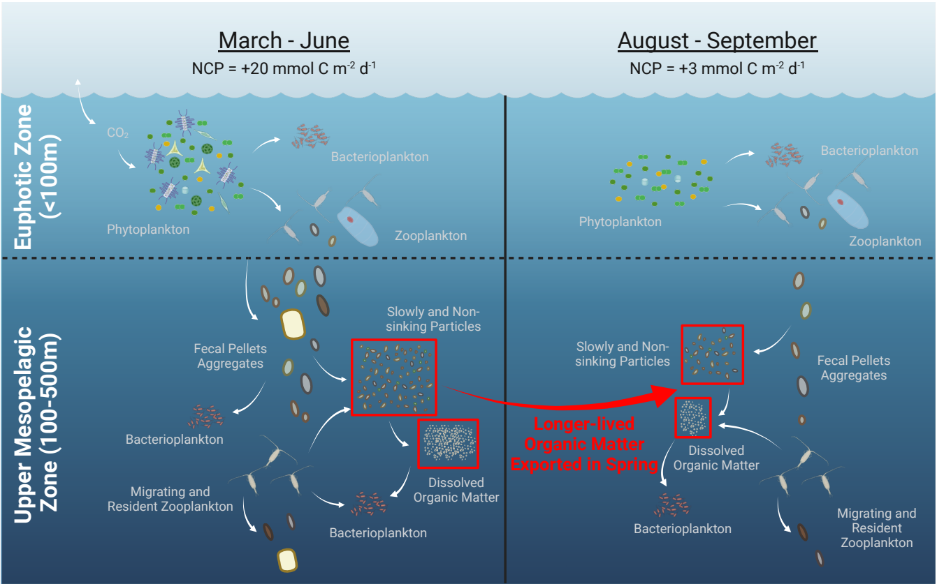
465 Figure 6: High net community production (NCP) in spring at Ocean Station Papa may have led to accumulating longer-lived, slowly- and non-sinking organic matter in the upper mesopelagic zone. Potential pathways for generating this accumulated organic matter could include particle disaggregation, solubilization, or release from vertically migrating zooplankton. This accumulated non-sinking organic matter may have contributed to the excess carbon demand in August 2018 (large red arrow) required for respiration compared with ship-based supply estimates. Created with BioRender https://BioRender.com/g5wmqh8 . 470
