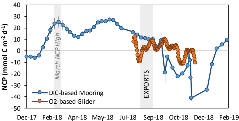
290 Figure 3: Depth-integrated (0-100 m) net community production (NCP) based on surface Ocean Station Papa (OSP) mooring measurements of dissolved inorganic carbon (December 2017 to February 2019) in blue and based on oxygen-sensor mounted to
