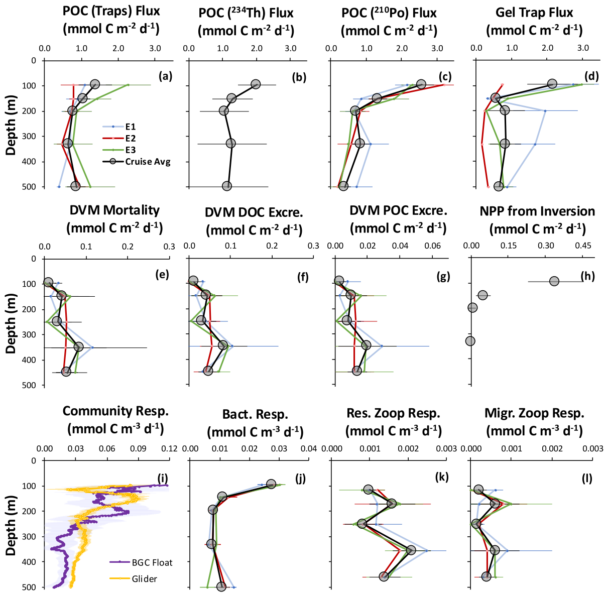
Figure 2: Epoch and cruise-mean profiles for carbon supply (subplots a to h) and demand (subplots i to l) estimates. Subplots a to d and i to j represent discrete sample collections, whereas subplots e to h and k to l represent samples collected across depth intervals. Subplots e to h are presented as depth-integrated units for comparison with passive supply subplots a to d. Net primary production (NPP) from inversion (subplot h) represents supply estimated from the inversion of size-fractionated [POC] data (Amaral et al., 2022), and only those data for the MZ are shown. Subplots i to l are shown in volumetric units. Community respiration from the glider and biogeochemical (BGC) float (subplot i) was estimated from long-term (>90 days) changes in [\text{O}_2] and converted to carbon
