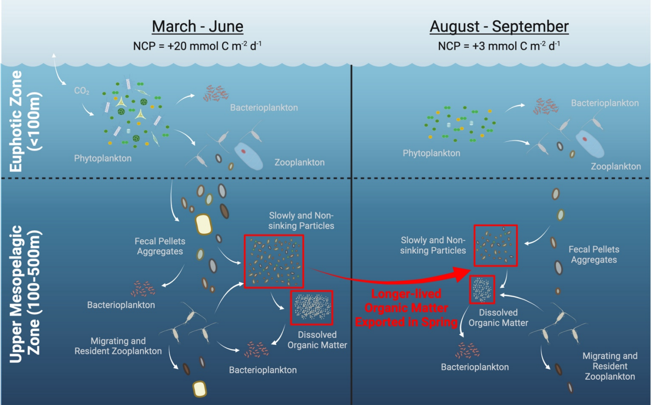
Figure 6: High net community production (NCP) in spring at Ocean Station Papa may have led to accumulating longer-lived, slowly- and non-sinking organic matter in the upper mesopelagic zone. Potential pathways for generating this accumulated organic matter could include particle disaggregation, solubilization, or release from vertically migrating zooplankton. This accumulated non-sinking organic matter may have contributed to the excess carbon demand in August 2018 (large red arrow) required for respiration compared with ship-based supply estimates. Created with BioRender.com.
