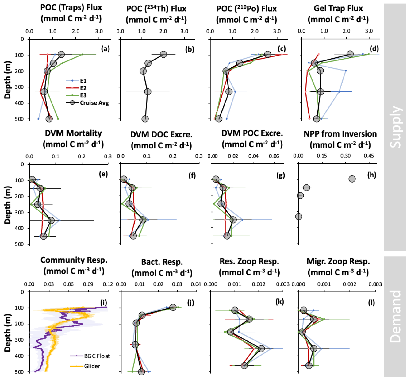
Figure 2: Epoch and cruise-mean profiles for carbon supply (subplots a to h) and demand (subplots i to l) estimates. Subplots a to d and i to j represent discrete sample collections, whereas subplots e to h and k to l represent samples collected across depth intervals.
