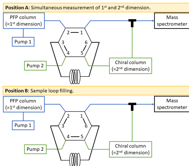
130 Figure 1: Instrumental setup of the heartcut-2D-LC method. In the first dimension, separation is performed using a PFP column; in the second dimension, the target enantiomers are separated on a chiral column. In position A, the sample loop is rinsed with solvent from pump 2. The heartcut is performed by switching to position B, whereby the target analyte from the first dimension is rinsed into the sample loop and then transferred to the chiral column by switching to A again. Both dimensions are combined via a T-piece and fed together into the mass spectrometer.
