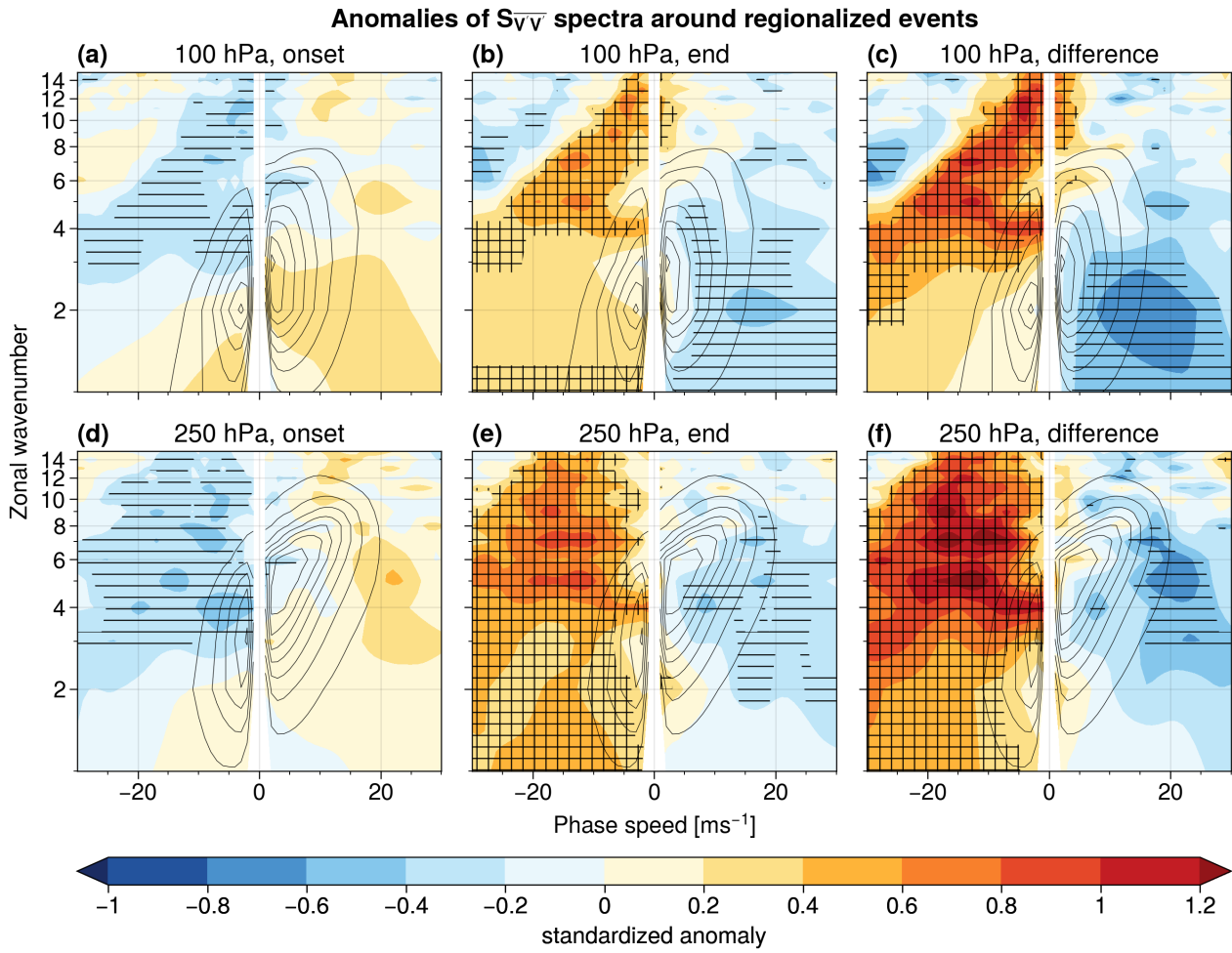
Figure A9. As Fig. 5, but for regionalized events (as defined in Sect. 2.2).
