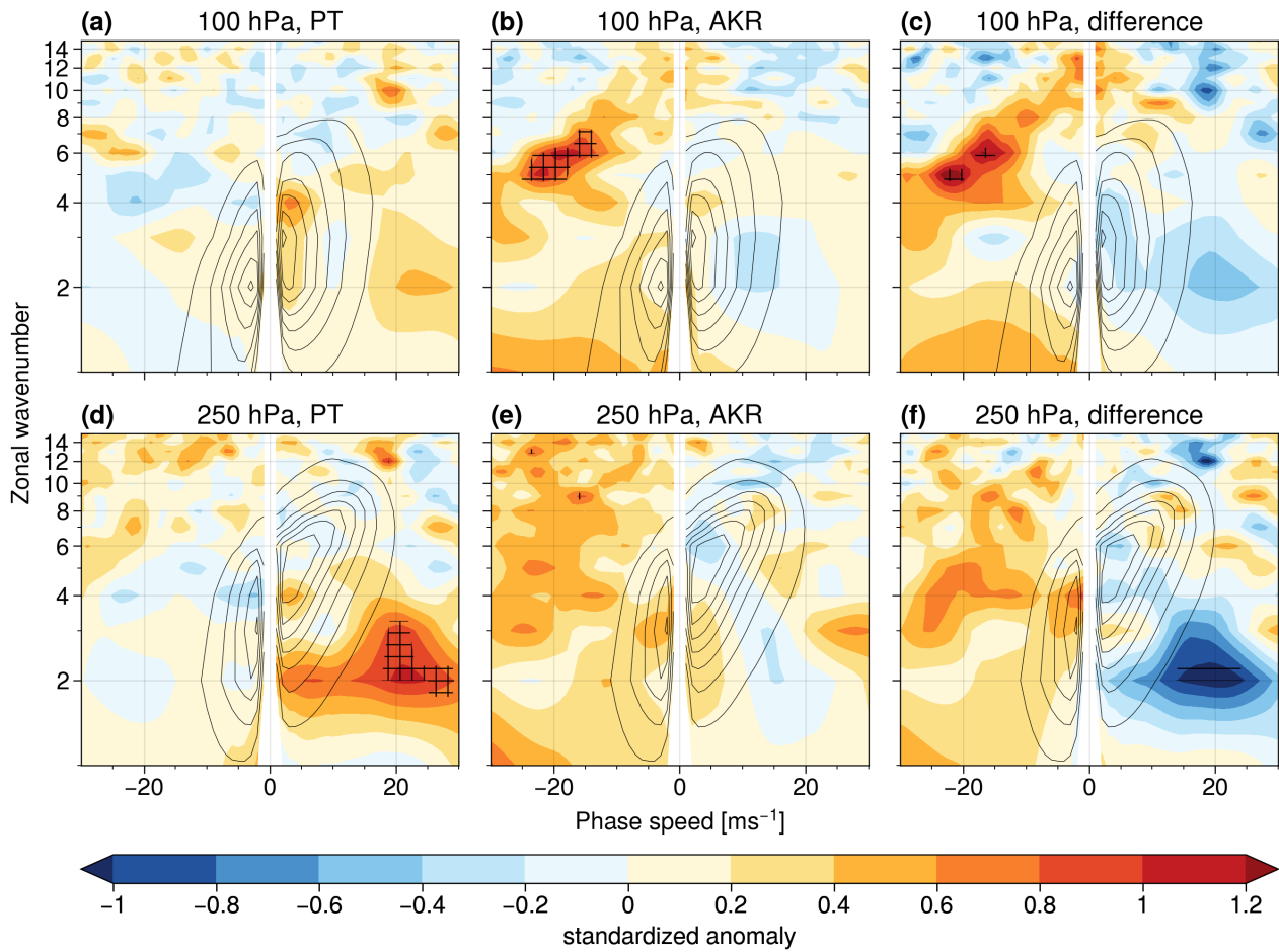
Figure A15. As Fig. 5, but for (a, d) PT regimes, (b, e) AKR regimes and (c, f) difference between PT and AKR regimes occurring during reflection events.
