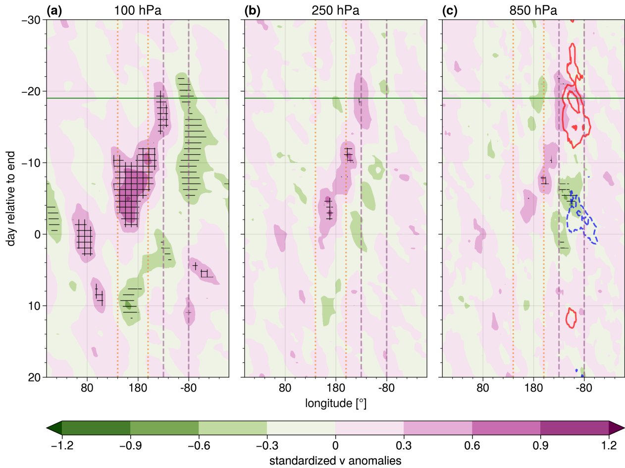
Figure A4. As Fig. 2, but for meridional wind speed at (a) 100 hPa, (b) 250 hPa and (c) 850 hPa.
