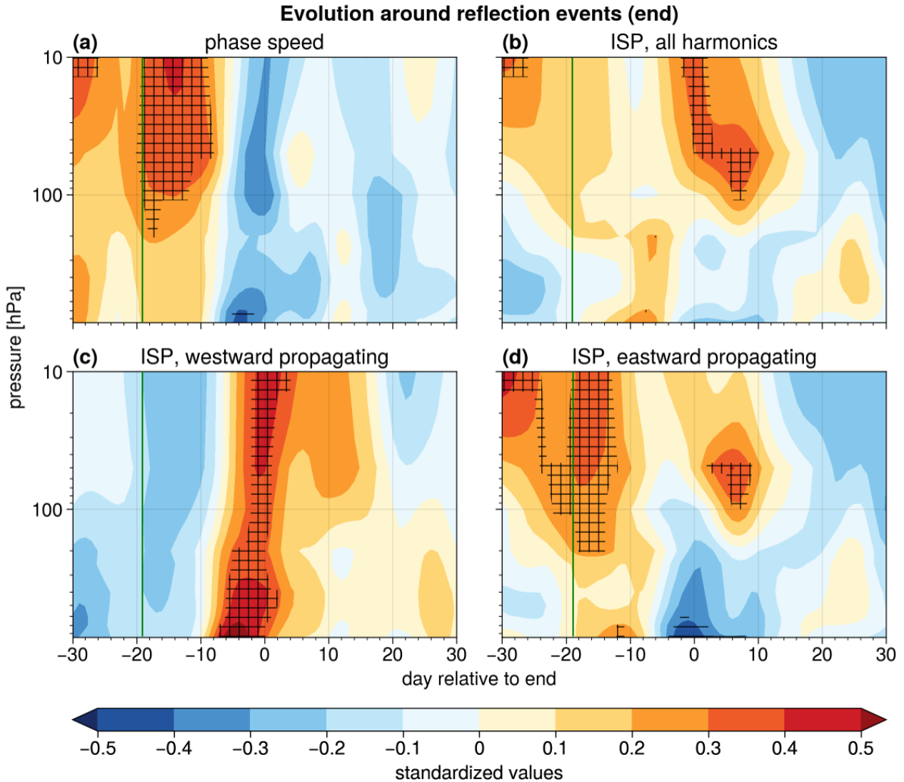
Figure 6. Vertical cross-section of standardized anomalies of (a) phase speed, (b) ISP, (c) ISP_{west} and (d) ISP_{east} derived from spectral power S_{\sqrt{V}}^2 between 850 hPa and 10 hPa centred around the end date of reflection events. Horizontal hatching marks statistically significant negative anomalies, cross-hatching statistically significant positive anomalies. The continuous vertical green line shows the median onset time of reflection events.
