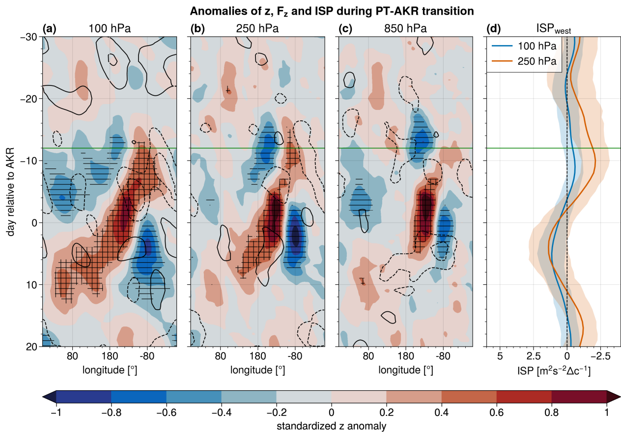
Figure 7. As in Fig. 3, but centred around the central date of AKR during PT-AKR transitions (See Sect. 2.2).
