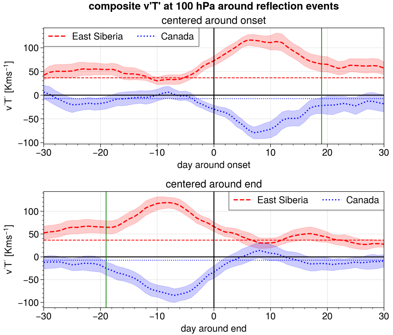
Figure A5. Meridional eddy heat flux \bar{v'T'} at 100 hPa over East Siberia (red, dashed) and Canada (blue, dotted), (a) centred around the onset date, (b) centred around the end date of reflection events. The thin horizontal lines show the DJFM mean in the respective region, shading indicates the 95% confidence interval on the mean, assessed with bootstrapping. The vertical green line in (a) shows the median end, and in (b) the median onset of reflection events.
