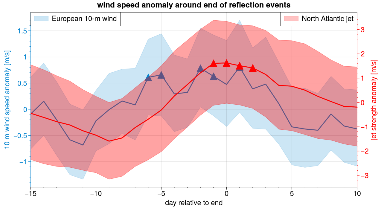
Figure A17. Anomaly of cosine-latitude weighted mean of 10-m wind speed over land grid points of Northern Europe (blue curve; 50\text{--}60^\circ\text{N} , 11^\circ\text{W}\text{--}20^\circ\text{E} ; blue box in Fig. 9 a) and anomaly of the jet strength (red curve). The jet strength is computed similarly to Woollings et al. (2010), but adapted to our study: The the zonal average of the 250 hPa zonal wind over the North Atlantic ( 15\text{--}75^\circ\text{N} , 70\text{--}0^\circ\text{W} 15\text{--}75^\circ\text{N} , 70\text{--}0^\circ\text{W} ; red box in Fig. 9 c) is smoothed with a centred 10-day running mean at each latitude. Subsequently the maximum wind speed is identified to define the jet strength on a given day which is then deseasonalized following See Sect. 2.1 . Shading indicates the 95% confidence interval of the mean and triangles highlight dates where the composite anomaly is above the 95th percentile of a resampled distribution of 10 000 means of 45 randomly selected days from the climatology.
