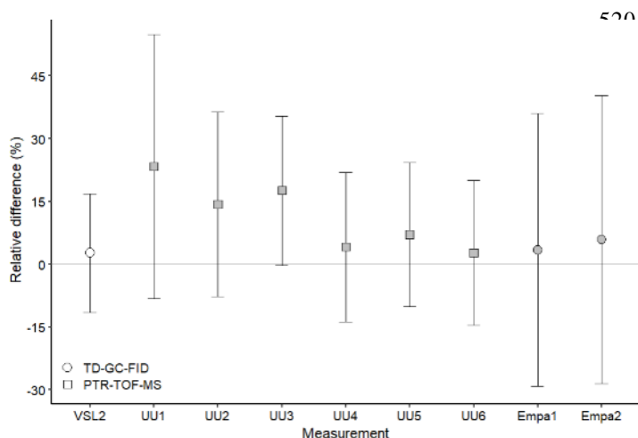
535 Figure 7: Assessment of the SI-traceable working standards based on the dilution of reference gas mixtures with dry nitrogen for acetaldehyde at amount fractions < 5 nmol mol -1 (grey symbols) and between 10-17 nmol mol -1 (white symbols). Error bars indicate the expanded uncertainty (coverage factor k = 2 ) of the relative difference between in-house and dilution working standards. Measurement labels show the participant and the number of SI-traceable working standards generated by dilution. Measurements were performed in August 2022 (VSL2), September 2022 (UU1-UU6) and November 2022 (Empa1, Empa2).
