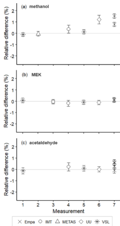
655 Figure 10: Assessment of the SI-traceable working standards based on certified spiked whole air samples in 10 L Experis® aluminium cylinders for (a) methanol, (b) methyl ethyl ketone (MEK) and (c) acetaldehyde. Error bars indicate the expanded uncertainty (coverage factor k = 2 ) of the relative difference between the measured and the certified amount fraction values of the working standards. Measurements were performed in Jul. 2021 (1), Feb. 2022 (2), Mar. 2022 (3), Jun. 2022 (4), Aug. 2022 (5), Sep. 2022 (6) and Nov. 2022 (7).
