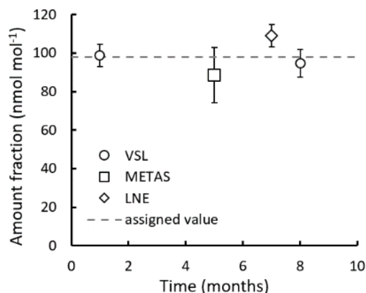
875 Figure B1: Interlaboratory comparison results for methanol. Reported values were the average of 5 measurements, except for month 1 results, which were the average of 3 measurements. Error bars show the expanded uncertainty of the measurements (coverage factor k = 2 ). The dashed line indicates the gravimetric amount fraction of the compound.
