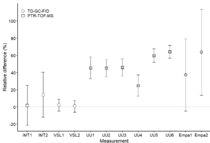
Figure 6: Assessment of the SI-traceable working standards based on the dilution of reference gas mixtures with dry nitrogen for methanol at amount fractions < 5 \text{ nmol mol}^{-1} (grey symbols) and between 10\text{--}17 \text{ nmol mol}^{-1} (white symbols). Error bars indicate the expanded uncertainty (coverage factor k = 2 ) of the relative difference between in-house and dilution working standards. Measurement labels show the participant and the number of SI-traceable working standards generated by dilution. Measurements
