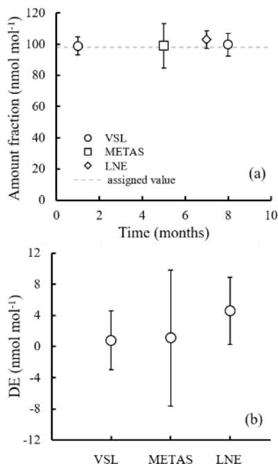
535 Figure 14: Interlaboratory comparison results for (a) acetone and (b) its degree of equivalence (DE; i.e., the deviation of each laboratory from the reference value). For VSL, only the first measurement period was considered (month 1) to estimate the DE. The measured amount fractions reported by the laboratories were the average of 5 measurements, except for month 1 results, which were the average of 3 measurements. Error bars show the expanded uncertainty of the measurements (coverage factor k = 2 ). The dashed line indicates the gravimetric amount fraction of the compound.
