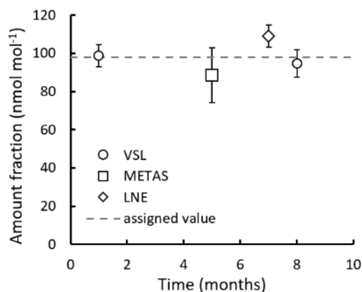
985 Figure B1: Interlaboratory comparison results for methanol. Reported values were the average of 5 measurements, except for month 1 results, which were the average of 3 measurements. Error bars show the expanded uncertainty of the measurements (coverage factor k = 2 ). The dashed line indicates the gravimetric amount fraction of the compound.
