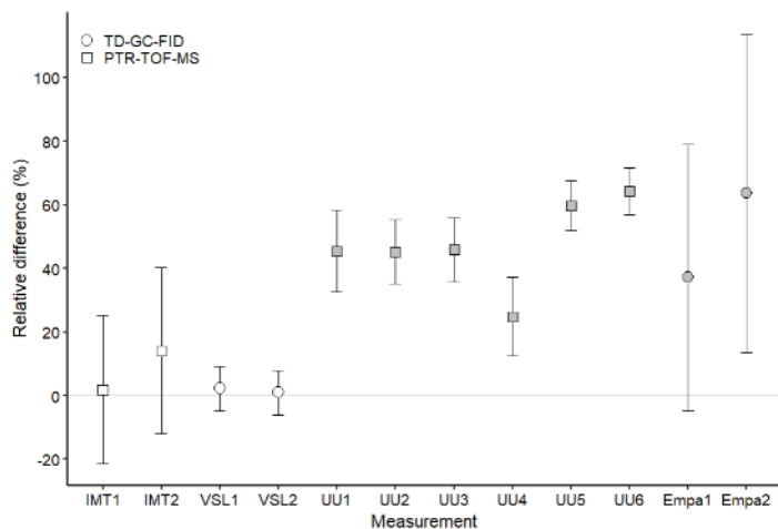
615 Figure 36: Assessment of the SI-traceable working standards based on the dilution of reference gas mixtures with dry nitrogen for methanol at amount fractions < 5 \text{ nmol mol}^{-1} (grey symbols) and between 10\text{--}17 \text{ nmol mol}^{-1} (white symbols). Error bars indicate the expanded uncertainty (coverage factor k = 2 ) of the relative difference between in-house and dilution working standards. Measurement labels show the participant and the number of SI-traceable working standards generated by dilution. Measurements
