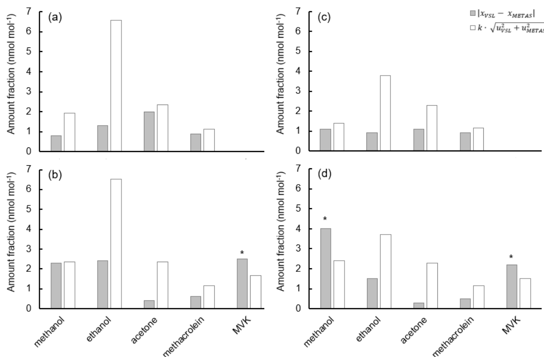
1065 Figure C1: Representation of the consistency of the amount fraction values assigned to the 10 L Experis cylinders according the criterion described in Eq. (4). METAS measurements (vessel 001C and 002A) performed in February 2022 were compared to the VSL measurements carried out in July 2021 on vessel 001A (a) and 002A (c) and in September 2022 on vessel 001A (b) and 002A (d). The asterisks show those measurements for which the absolute difference of the measured amount fractions ( x_{VSL} - x_{METAS} ) was greater than twice (coverage factor k = 2 ) the square root of the sum of squares of the measurement standard uncertainties ( u_{VSL}, u_{METAS} ).
