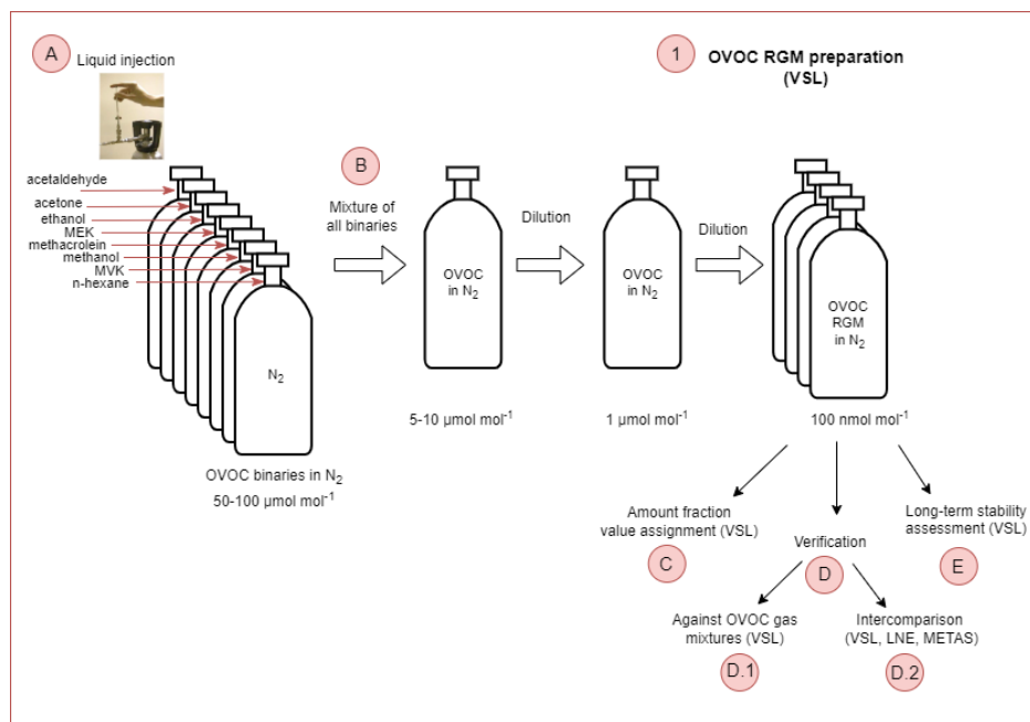
165 Figure 2: Schematic diagram illustrating the steps needed to prepare the reference gas mixtures (RGMs) of the selected oxygenated volatile organic compounds (OVOCs).
