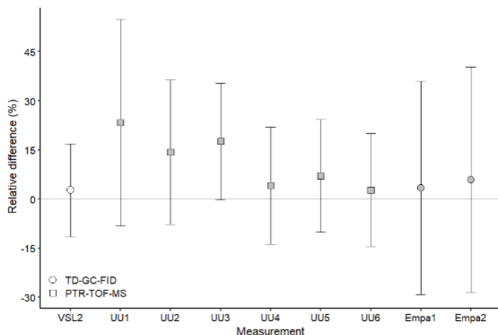
630 Figure 47: Assessment of the SI-traceable working standards based on the dilution of reference gas mixtures with dry nitrogen for acetaldehyde at amount fractions < 5 \text{ nmol mol}^{-1} (grey symbols) and between 10\text{-}17 \text{ nmol mol}^{-1} (white symbols). Error bars indicate the expanded uncertainty (coverage factor k = 2 ) of the relative difference between in-house and dilution working standards. Measurement labels show the participant and the number of SI-traceable working standards generated by dilution. Measurements were performed in August 2022 (VSL2), September 2022 (UU1-UU6) and November 2022 (Empa1, Empa2).
