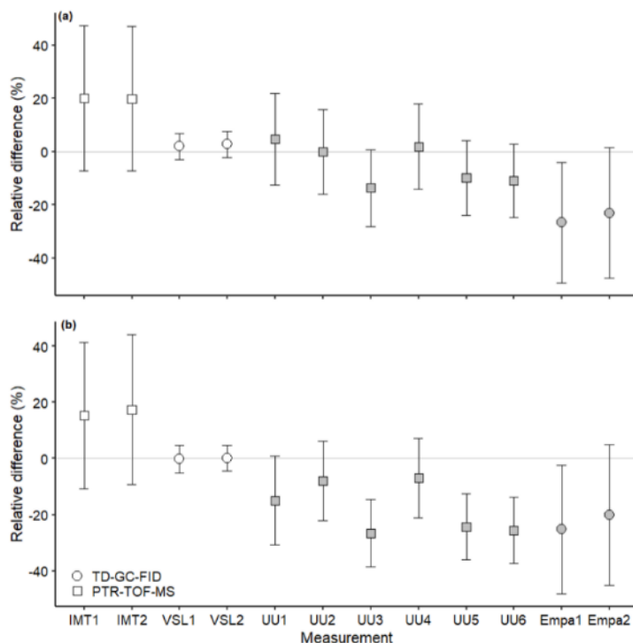
600 Figure 25: Assessment of the SI-traceable working standards based on the dilution of reference gas mixtures with dry nitrogen for (a) acetone and (b) MEK at amount fractions < 5 \text{ nmol mol}^{-1} (grey symbols) and between 10\text{--}17 \text{ nmol mol}^{-1} (white symbols). Error bars indicate the expanded uncertainty (coverage factor k = 2 ) of the relative difference between in-house and dilution working standards. Measurement labels show the participant and the number of SI-traceable working standards generated by dilution. Measurements were performed in July 2022 (IMT1, IMT2), August 2022 (VSL1, VSL2), September 2022 (UU1-UU6) and November 2022 (Empa1, Empa2).
