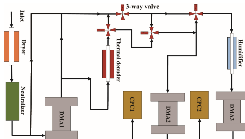
Figure 1. The schematic diagram of the VH-TDMA.
