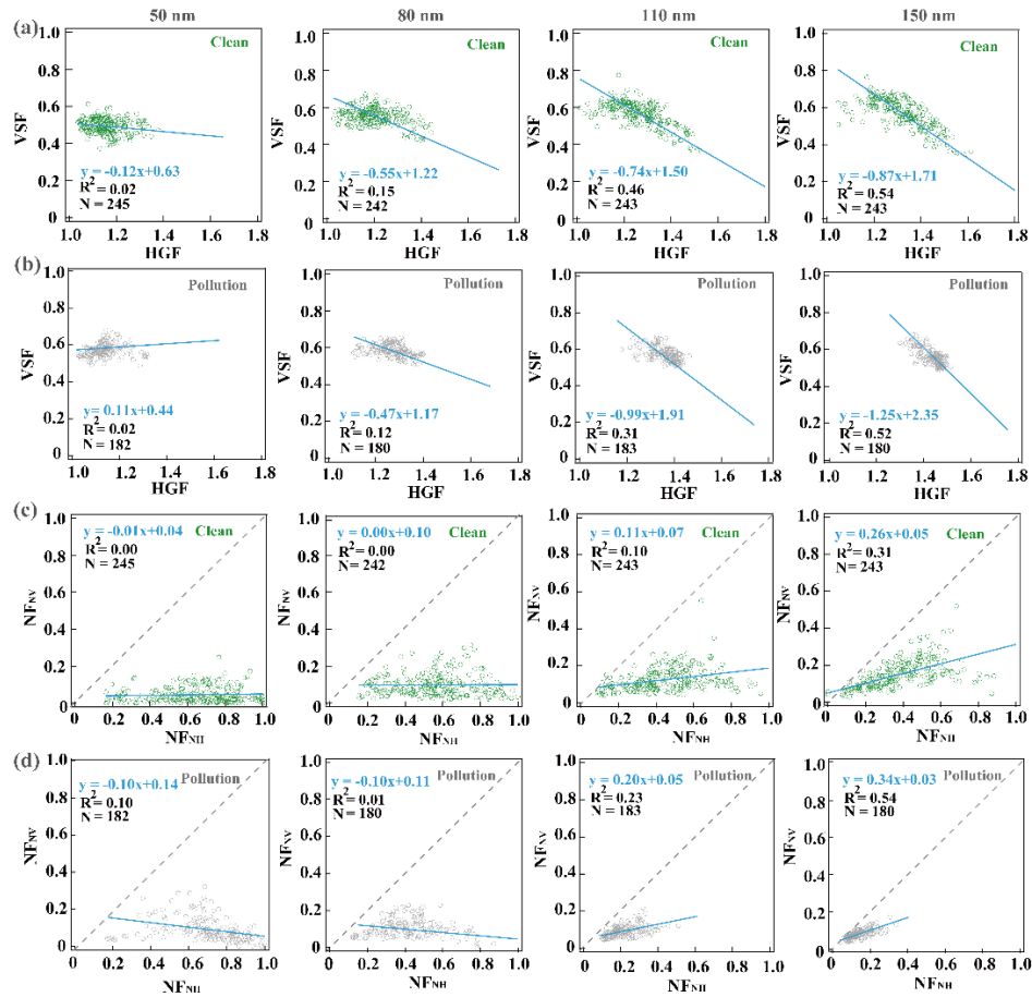
Figure 7. Relationship between the hygroscopic growth factors (HGFs) and the volatility shrink factors (VSFs) during the clean and pollution periods for different dry particle diameters (a, b); relationship between the NF NH and the NF NV during the clean and pollution periods (c, d) for different dry particle diameters.
