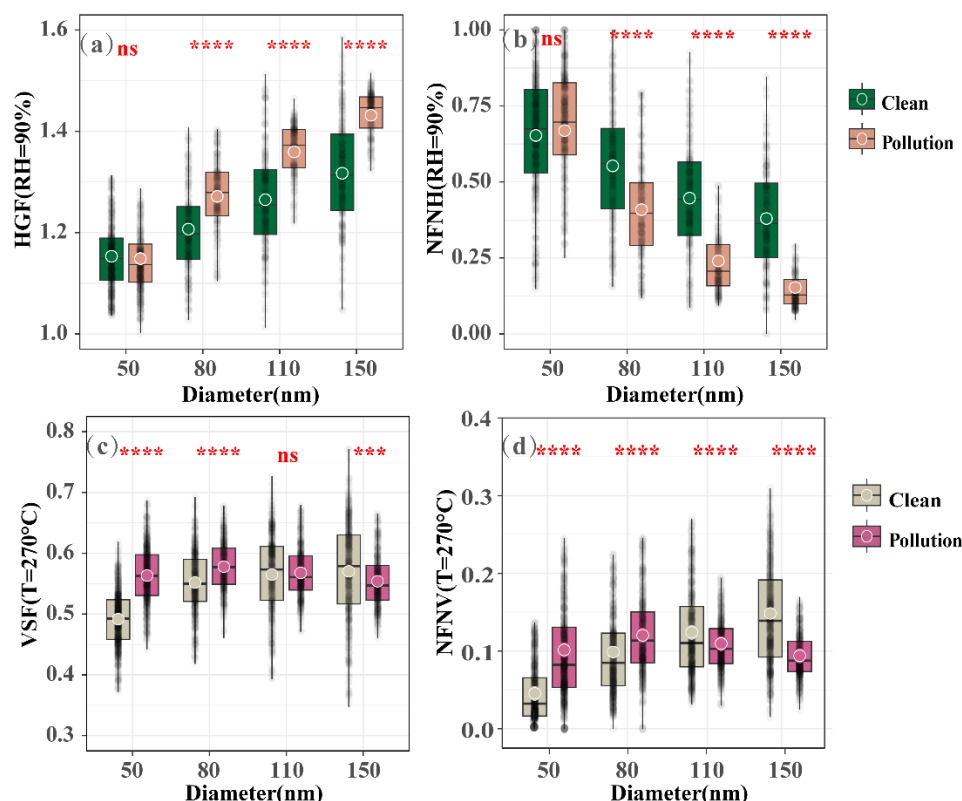
Figure 6. Boxplot of (a) size-resolved hygroscopic growth factor (HGF) and (b) the number fraction of nearly hydrophobic mode particles (NF NH ) during the clean and pollution periods. (c) (d) same as (a) (b) but for volatile shrink factor (VSF) and number fraction of non-volatile mode particles (NF NV ), respectively. The two borders of box indicate the 25th and 75th percentiles, the line in box represents the median, whiskers indicate the 5th and 95th percentiles, and the circle in each box indicates the mean. Ns means the observed difference is not statistically significant, **** means P value \leq 0.0001 .
