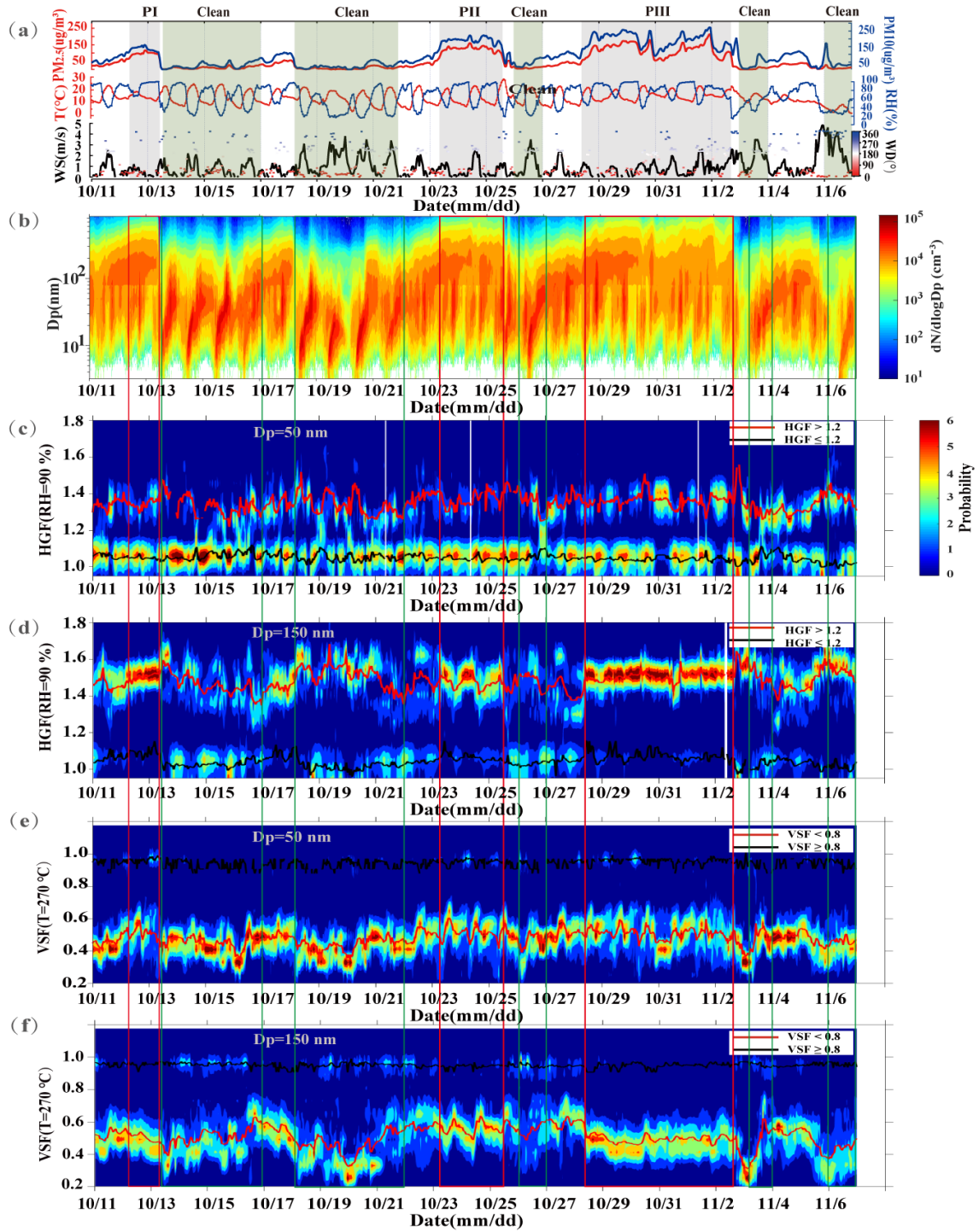
Figure 2. Time series of PM_{2.5} and PM_{10} mass concentrations and meteorological parameters (a), PNSD from TSMPS (b), hygroscopic growth factor probability density function (HGF-PDF) for 50 nm (c) and 150 nm (d) particles at RH = 90\% , and volatile shrink factor probability density function (VSF-PDF) for 50 nm (e) and 150 nm (f) particles at T = 270^{\circ}C . In the HGF-PDFs, the blackline represents the mean HGF of the nearly hydrophobic mode ( HGF_{NH} ), and the red line represents the mean HGF of the more hygroscopic mode ( HGF_{MH} ). In the VSF-PDFs, the blackline represents the mean VSF of the non-volatility mode ( VSF_{NV} ), and the red line represents the mean VSF of the very volatility mode ( VSF_{VV} ).
