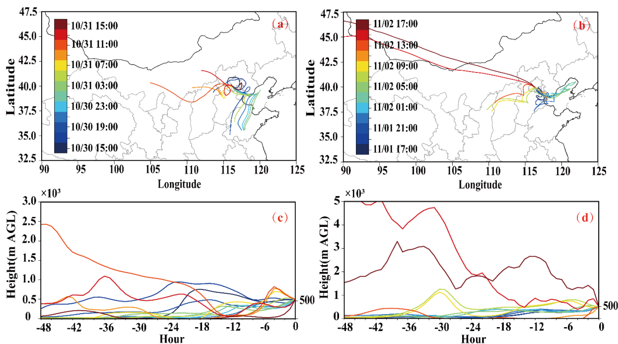
Figure 10. The 48-h back trajectories arriving at the height of 500 m AGL at the CAMS site were calculated every two hours from 30 October, 15:00 to 31 October, 15:00 including event I (a), and from 1 November, 17:00 to 2 November, 17:00 including event II (b). (c) and (d) show the air mass heights of the backward trajectories corresponding to (a) and (b), respectively. The color scale represents the time of air mass backward trajectory arrived at the sampling site. 625
