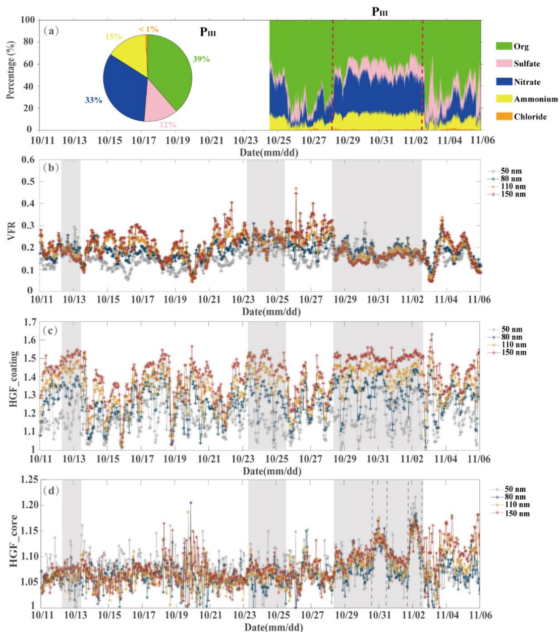
Figure 8. Time series of the main mass fraction of chemical components in PM 1 during the sampling period based on the available AMS data (a), The volume fraction of non-volatile core (VFR) (b), calculated HGF coating (c) and measured HGF core (d) for particles from 50 nm to 150 nm during the sampling period. The shadows represent the pollution period and the dashed lines represent the period during which the hygroscopicity of non-volatile core was relatively high.
