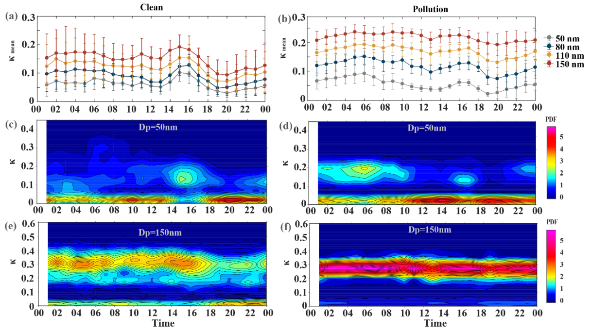
Figure 4. Diurnal variation of mean \kappa for different diameters and the error bars represent the standard deviations (a, b); \kappa -PDF for particles with D_p = 50 nm (c, d) and \kappa -PDF for particles with D_p = 150 nm (e, f) during the clean and pollution periods, respectively.
