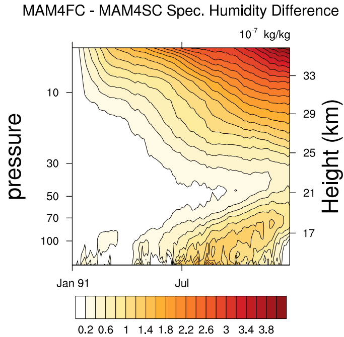
Figure S3: Differences in specific humidity between MAM4FC and MAM4SC. The vertical axis represents altitude, while the horizontal axis represents time. Values are averaged over all longitudes and 30S-30N latitudes.
