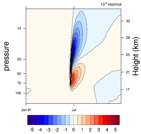
MAM5FC - MAM5SC SO 2 Conc. Difference
