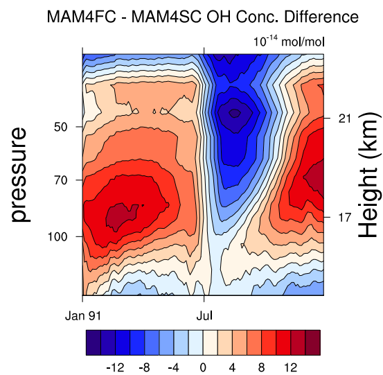
Figure S1: Differences in SO 2 concentrations and OH concentrations between MAM4FC and MAM4SC. The vertical axis represents altitude, while the horizontal axis represents time. Values are averaged over all longitudes and 30S-30N latitudes.
