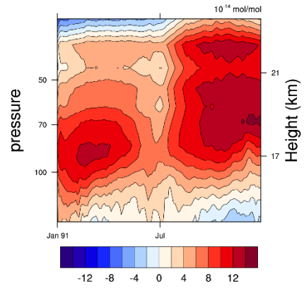
MAM5FC - MAM5SC OH Conc. Difference
