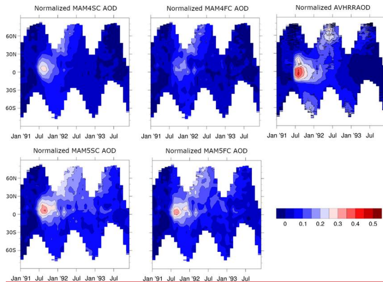
Figure 98: Latitude vs. time plots of model simulated AOD and AVHRR observed AOD. Both were normalized to 1989 AOD output or observations respectively, to eliminate contributions from the troposphere and background stratospheric AOD. Model output was masked to correspond to areas that AVHRR had observation data for. Results were averaged across longitude.
