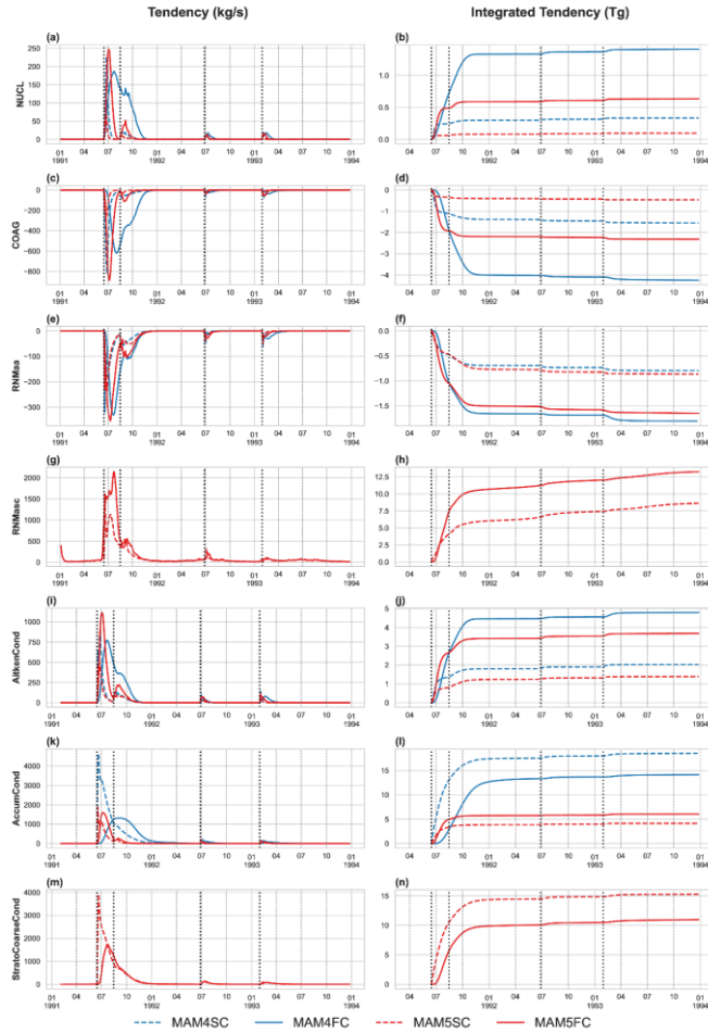
Figure 67: The relevant tendencies for each mode in each experiment in the stratosphere between 80°S and 80°N. See Figure 1(a) for description of processes. Positive values represent gained mass from the associated microphysical process from the perspective of the aerosol mode in question. NUCL represents the aerosol mass gain for Aitken mode due to nucleation (i.e., aerosol formation), COAG represents Aitken mode mass loss due to coagulation into the accumulation mode, RNMa represents Aitken mode mass loss due to renaming into the accumulation mode, RNMaSC represents the gain in mass for stratospheric coarse mode in MAM5-PSA due to renaming from the accumulation mode. The left column plots represents represent the tendency values over time, while the right column represents the cumulative mass change due to the associated microphysical process (i.e. tendency integrated over time). The bottom three rows represent the condensation tendencies for each mode, with the positive value representing mass transition from gaseous phase to the aerosol. The vertical lines represent the Pinatubo, Cerro Hudson, Spurr and Lascar eruptions respectively.
