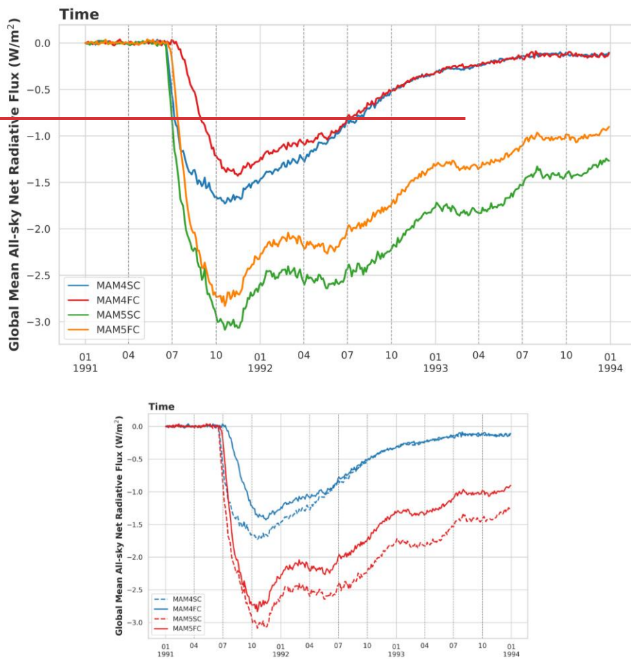
Figure 11: Global mean net radiative flux in the four experiments, where negative values represent a net upward flux. ▲
