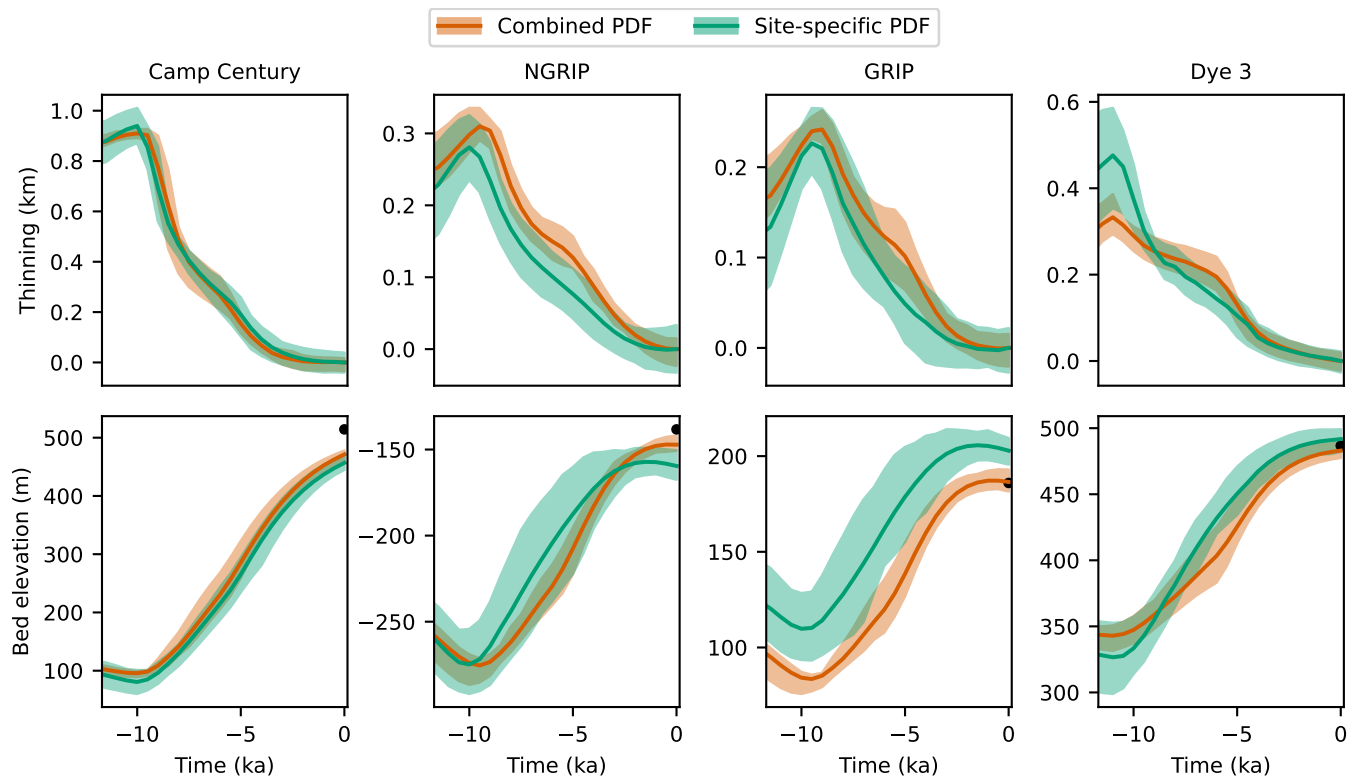
Figure A7. Modeled bedrock elevation and thinning over the past 11.7 ka at the ice-core ice-core sites Camp Century, NGRIP, GRIP, and Dye 3. The red envelopes represent the ensemble-estimated mean and standard deviation, while the green envelopes show the site-specific estimate. The black dots indicate the observed present-day bedrock elevation from Morlighem et al. (2017).
