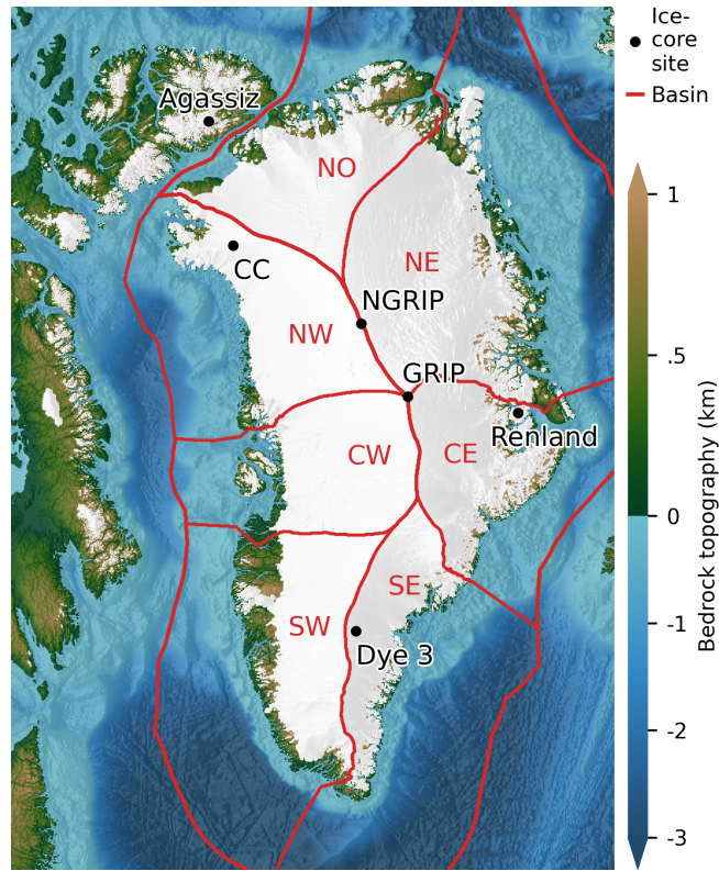
Figure 1. Model domain showing the present-day bedrock topography elevation from Morlighem (2022), Jakobsson et al. (2020), and GEBCO Bathymetric Compilation Group (2023) and with the present-day ice cover from Morlighem (2022) and RGI Consortium (2023) shown in white. The ice-core ice-core sites discussed in the text (CC, NGRIP, GRIP, Dye 3, Renland, and Agassiz) are shown on top together with the glacier catchment basins (NW, CW, SW, SE, CE, NE, NO) from Mouginot and Rignot (2019) and extended out to the Exclusive Economic Zone of Greenland (Flanders Marine Institute (VLIZ), Belgium, 2023) and constitute our extended continental shelf (ECS) domain, see text.
