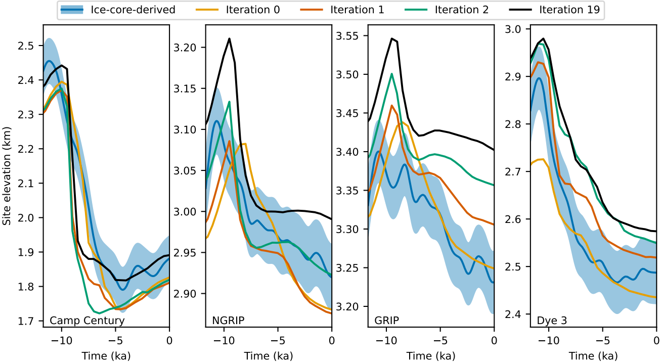
Figure A6. Observed and modeled surface elevation over the past 11.7 ka at the ice-core ice-core sites Camp Century, NGRIP, GRIP, and Dye 3. The blue lines represent ice-core-derived surface elevations from Vinther et al. (2009), with the blue envelopes indicating one standard deviation. The orange, red, green, and black lines correspond to the modeled surface elevations for the 0th, 1st, 2nd, and 19th iterations of the bedrock adjustment, respectively.
