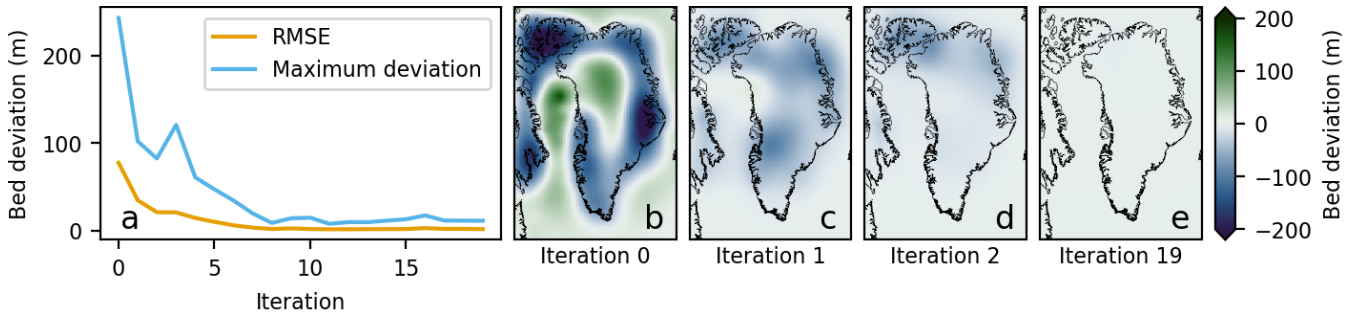
Figure 3. Iterative bedrock adjustment. (a) The modeled present-day bedrock elevation deviation compared to (Morlighem, 2022; Jakobsson et al., 2020; GEBCO Bathymetric Compilation Group, 2023) Morlighem (2022), Jakobsson et al. (2020), and GEBCO Bathymetric Compilation Group (2023). (b–e) shows the zeroth to the third, first, second, and 19th iteration of the modeled present-day bedrock elevation deviation from observed.
