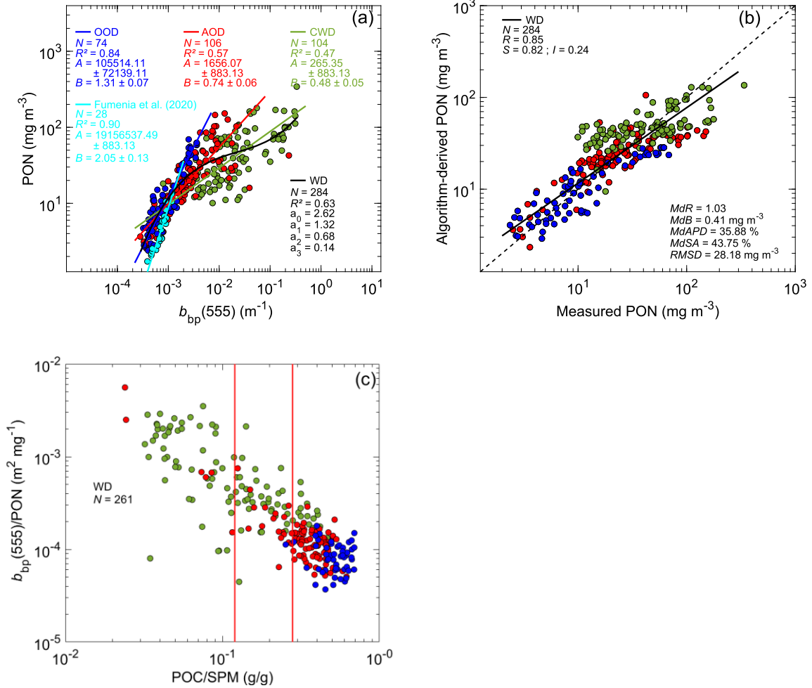
Figure 7. (a) Relationships between PON and b_{\text{bp}}(555) for different datasets as indicated with black, dark blue, red, and green colors corresponding to the whole dataset (WD), open-ocean dataset (OOD), Arctic Ocean dataset (AOD), and coastal-water dataset (CWD), respectively. The solid dark blue, red, and green lines represent the best fit power functions obtained from Model-II linear regression on log 10 -transformed data. The solid black line represents the best fit 3 rd -degree polynomial function. For comparison, data in light blue from Fumenia et al. (2020) are shown after conversion of measured b_{\text{bp}}(700) to b_{\text{bp}}(555) using a \lambda^{-1} spectral dependency. The standard deviation of the best fit coefficients, A and B , is indicated. (b) Comparison of algorithm-derived and measured PON where the algorithm is the black line in panel (a) for the whole dataset WD. The black solid line is the best-fit function obtained from Model-II linear regression on log 10 -transformed data. The dashed line represents the 1:1 line. (c) Scatter plot of b_{\text{bp}}(555)/\text{PON} vs. POC/SPM. The red vertical lines refer to the threshold values of POC/SPM of 0.12 and 0.28 which delimit the mineral-dominated from mixed particulate assemblages and mixed from organic-dominated particulate assemblages, respectively (Stramski et al., 2023). Panels (a) and (b) of the figure include the statistical indicators (see Sect. 2.4 for details).
