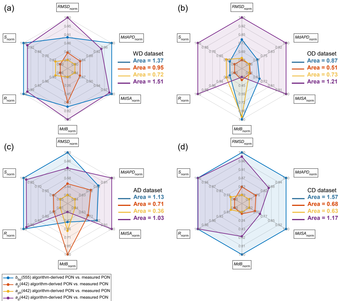
Figure 11. Radar plots summarizing the performance of the IOP-based algorithms for deriving PON. The IOPs( \lambda ) considered are the b_{bp}(555) (blue line), a_p(442) (red line), a_{ph}(442) (yellow line), and a_d(442) (purple line). The smallest area of the polygon associated with each algorithm represented in the radar plot corresponds to the best performance. The coefficient of correlation, R , Slope, S , Root Mean Square Deviation, RMSD , Median Bias, MdB , Median Absolute Percentage Difference, MdAPD , and Median Symmetric Accuracy, MdSA , subject to appropriate normalization (see Sect. 2.4) are indicated (a) for the WD, (b) OOD, (c) AOD, and (d) CWD datasets.
