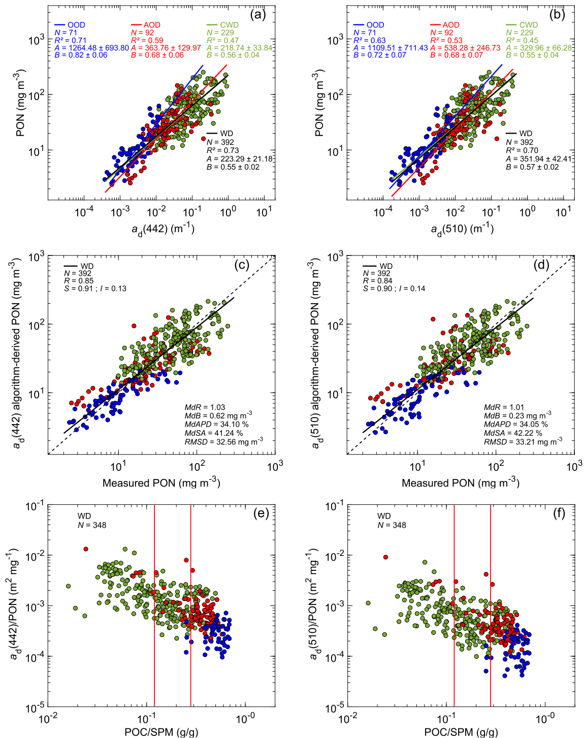
Figure 10. Same as Figure 8 but for the non-algal particulate absorption coefficients a_d(442) and a_d(510) .
