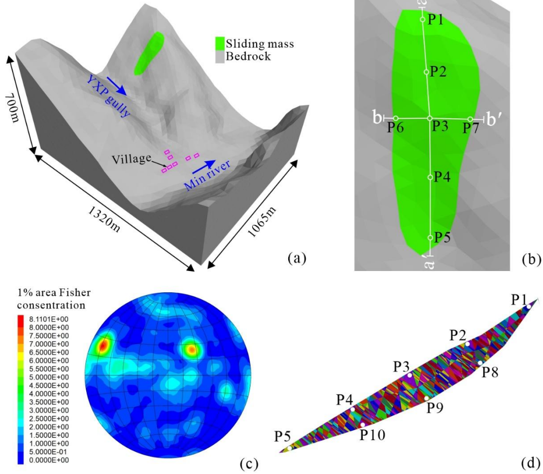
Figure 6: The three-dimensional model of YXP rockslide (a) and monitoring points in source area (b). Fisher distribution of in-site measured rock fractures (c) and sliding mass cut by DFN (d).
