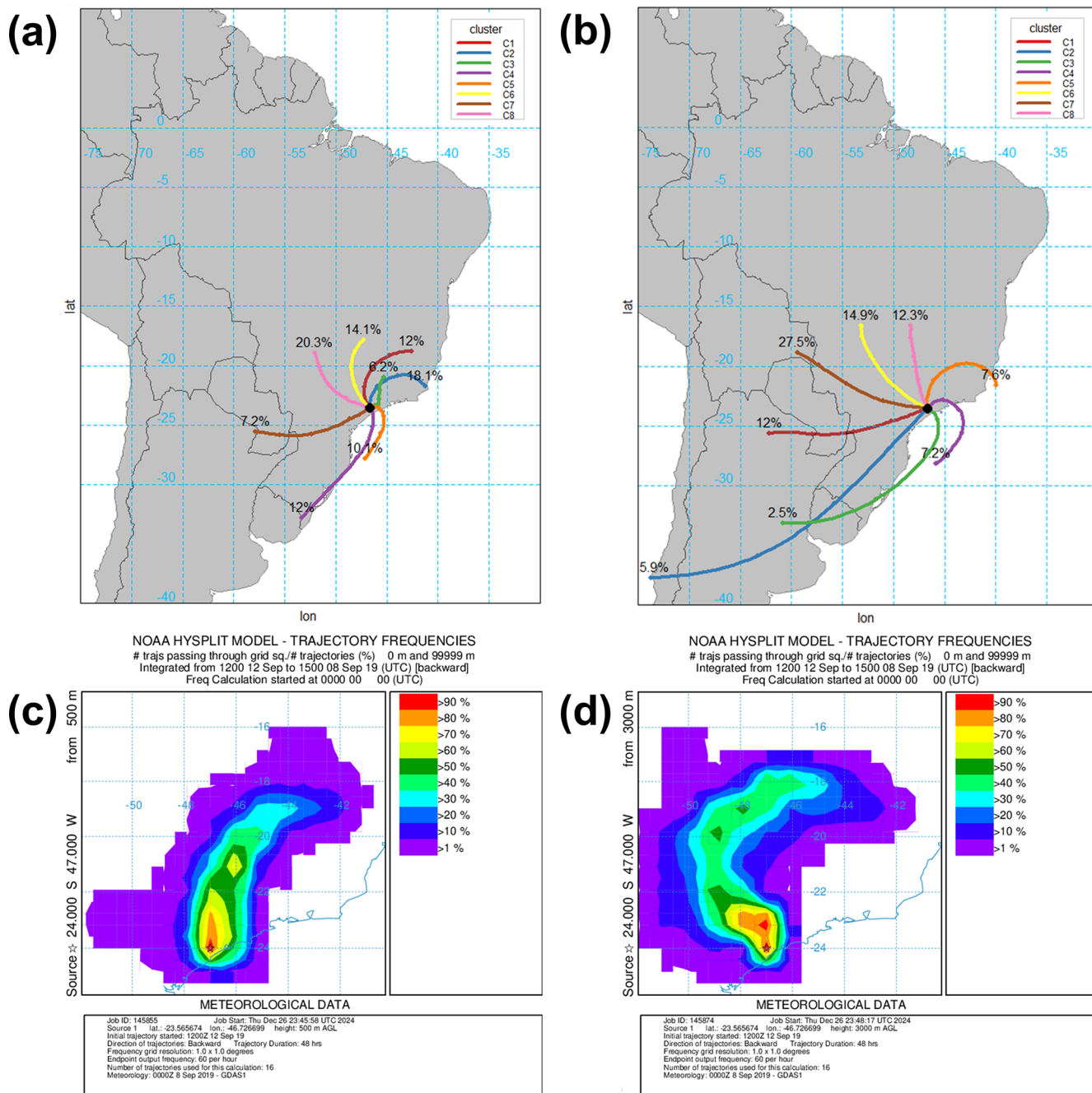
Figure 3. Backward trajectory clusters for the sampling period, arriving at (a) 500 m and (b) 3000 m, and trajectory frequencies for 10 and 11 September 2019, arriving at (c) 500 m and (d) 3000 m. TS6
