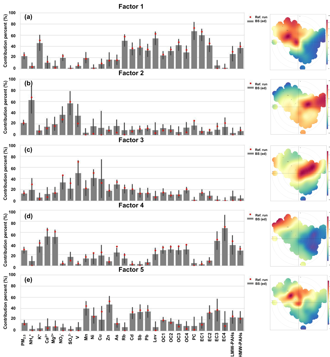
Figure 6. Profiles identified with the PMF receptor model and polar plots. (a) Factor 1: biomass burning (BB). (b) Factor 2: secondary formation (SF). (c) Factor 3: industrial (IN). (d) Factor 4: vehicular + road dust (VE1). (e) Factor 5: local vehicular (VE2). Model reference runs (Ref. run) are marked in red, and bootstrap runs (BS) and standard deviation (SD) are marked in gray.
