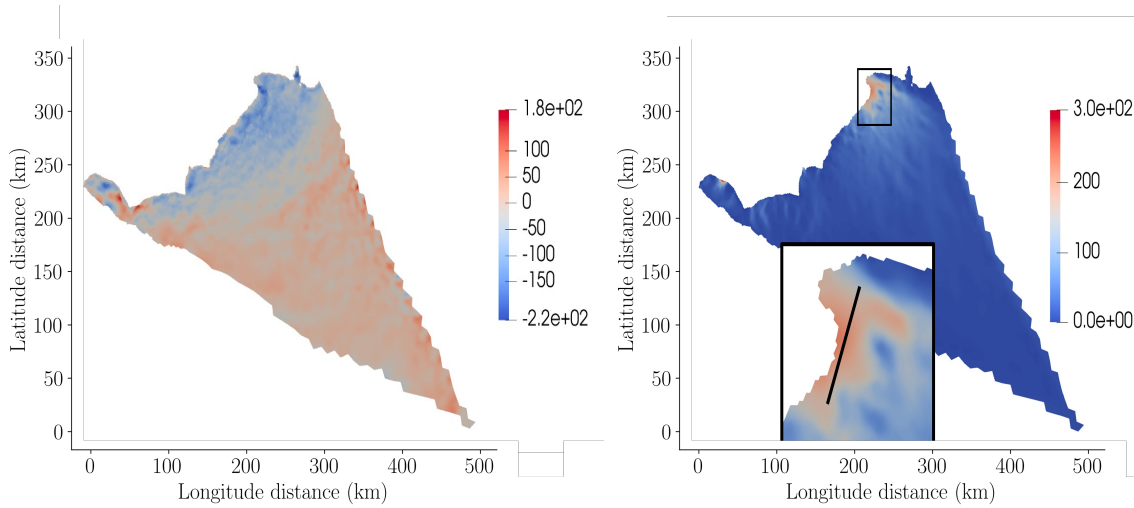
Figure 7. (Left) The difference between the final and initial ice thickness in meters and (Right) the surface velocity of Humboldt Glacier. The left box is a zoomed in picture of the top right tip of the glacier. The black line in the inset was used to plot cross-sections of the thickness and friction profiles at 2100 in a region with high velocities (see Figure 14). Both the left and right figures were generated using the highest-fidelity model \text{MOLHO}_{1\text{km},9\text{days}}^* evaluated at one random realization of the posterior of the basal friction field.
