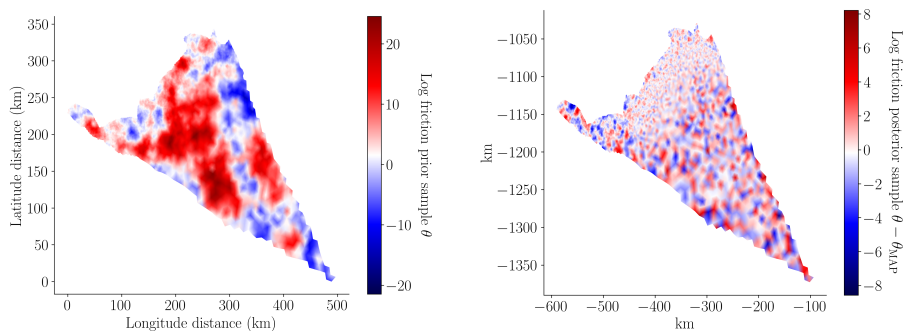
Figure 6. (Left) A random sample from the prior distribution of the log-friction p(\theta) \sim \mathcal{N}(0, \Sigma_{\text{prior}}) , where \Sigma_{\text{prior}} is defined in Eq. (9). (Right) A random sample from the Laplace approximation of the posterior p(\theta | \mathcal{M}, \mathbf{y}) \sim \mathcal{N}(\theta_{\text{MAP}}, \Sigma_{\text{post}}) , defined in Eq. (14).
