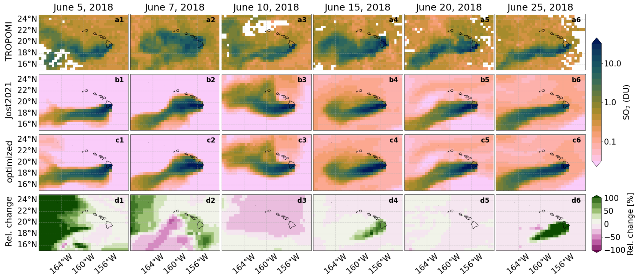
Figure 9. Observed (top) and simulated \text{SO}_2 columns resulting from the degassing of the Kilauea volcano at selected days in June 2018 at a model resolution of T255. a* , a) Observations from TROPOMI, regridded to T255 resolution. b* , b) Simulation with emission rates derived by Jost (2021, scaled by a factor of 4.3 – see text for details). c* , c) Simulation with optimized emission rates, based on a comparison between model and observations (refer to the text for more details). d* , d) Relative change from the simulation with derived emission rates by Jost (2021) to the optimized simulation.
