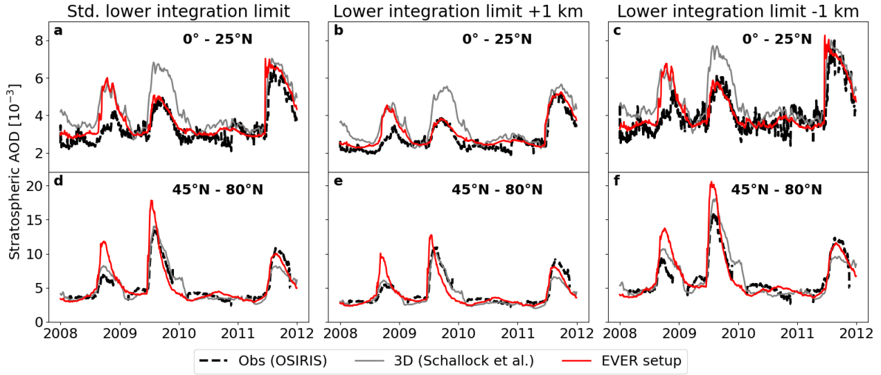
Figure A2. Sensitivity of the evaluation result to the lower integration limit (applied to observations and simulations) for the derivation of sAOD. a,d a,d ) Lower integration limit as applied in the manuscript (16 km from 0-25°N and 12 km from 45-80°N). Variations of plus 1 km ( b,e,b,e ) and minus 1 km ( c,f,c,f ) show similar agreement at different absolute values. The most significant differences are observed for the Sarychev volcano, that shows strongly decreased simulated sAOD at increased lower integration limit at higher latitudes ( ee ).
