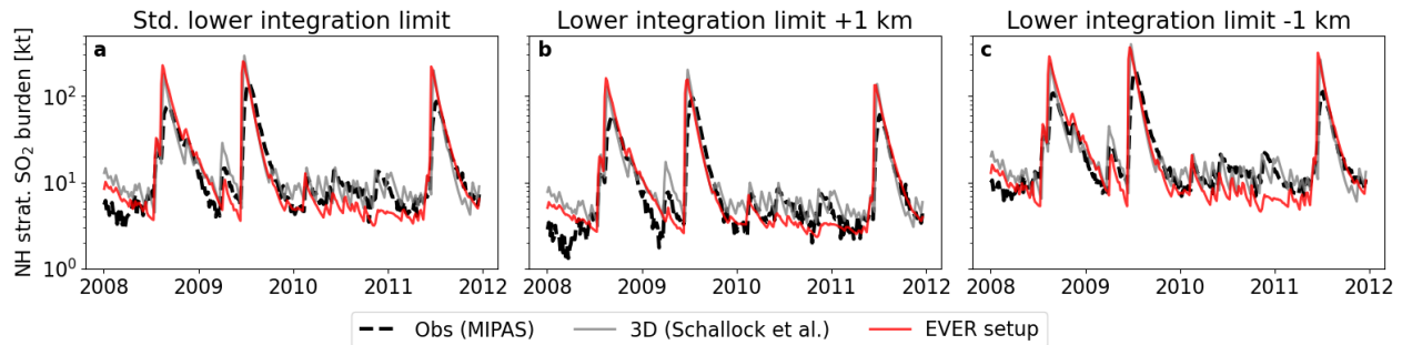
Figure A1. Sensitivity of the evaluation results to the lower integration limit (applied to observations and simulations) for the derivation of the stratospheric SO 2 burden. a ; a ) Lower integration limit as applied in the manuscript (16 km from 0-30°N, 14 km from 30-60°N and 12 km from 60-90°N). Variations of plus 1 km ( b ) and minus 1 km ( c ) show similar agreement at different absolute values. Slight differences can be seen at background levels with increased agreement in 2010 for the increased lower integration limit ( b ).
