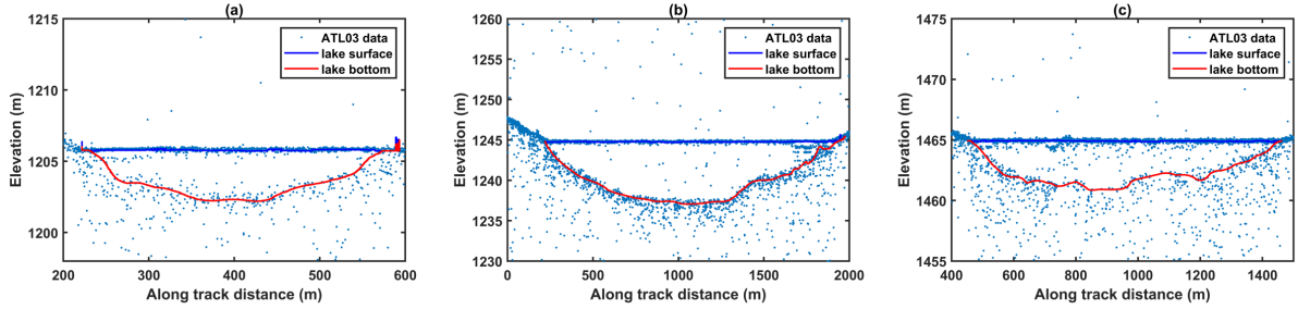
Figure 5. Three examples of lake surface and bottom detection results based on ICESat-2 ATL03 data. The locations of lakes (a), (b), and (c) are shown in Fig. 1.
