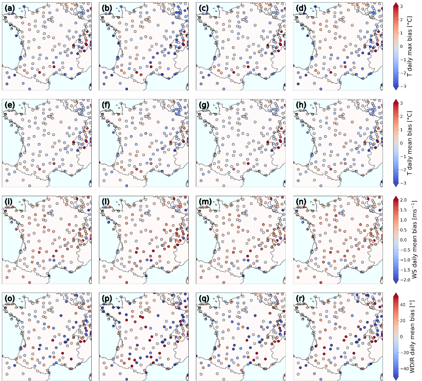
1060 Figure 4: Daily bias obtained by comparing model output to observations from the MIDAS database, respectively for (left column) the full period, (middle left column) the first heatwave, (middle right column) the clean period and (right column) the second heatwave for the (a)–(d) max temperature, (e)–(h) mean temperature, (i)–(n) wind speed and (o)–(r) wind direction.
