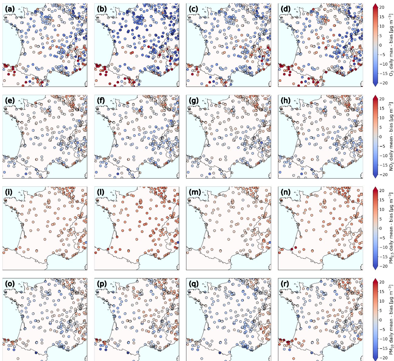
1080 Figure 6: Daily biases obtained by comparing model output to the EEA observations respectively for the full period (left column), the first heatwave (middle left column), the clean period (middle right column) and the second heatwave (right column) for the (a)–(d) O 3 daily max, (e)–(h) NO 2 mean, (i)–(n) PM 2.5 mean and (o)–(r) PM 10 mean.
