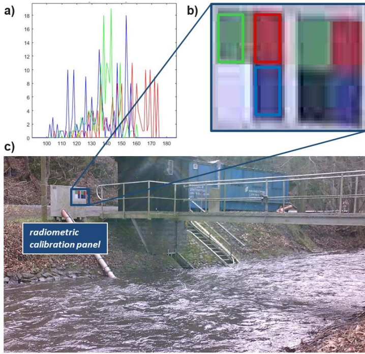
200 Figure 9: Example of radiometric calibration procedure applied to a TC image, using the reference mean RGB values (a) of the radiometric calibration panel (b) installed within the camera field of view (c).
