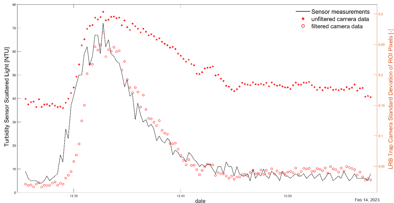
Figure 20: Comparison of turbidimeter measurements (line in black) and the standard deviation of ROI pixels intensity in LRB trap camera red band filtered (“o” symbols in red) and unfiltered (“*” symbols in red) data, during the short-term experiment of February 2023.
