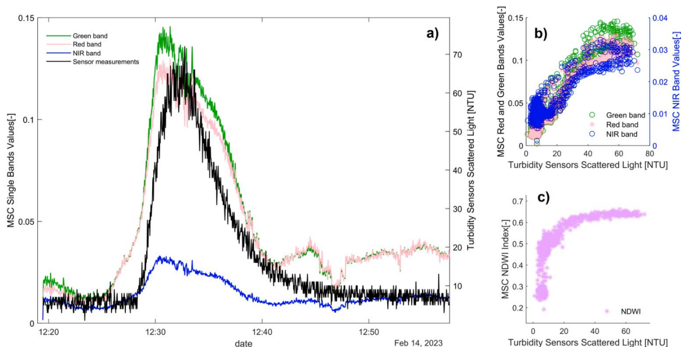
245 Figure 11: a) Comparison between turbidimeter measurements and data from the multispectral camera (MSC) installed on the bridge; b) Scatter plot of the MSC single bands values and on-site measurements; c) Scatter plot of the MSC NDWI values and on-site measurements. The colour schemes used in this figure are accessible to persons with colour vision deficiencies.
