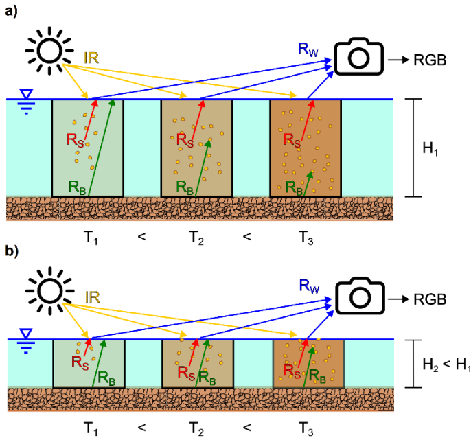
75 Figure 1: Light behaviour within shallow (b) and non-shallow water (a): The solar irradiance (IR) passes through the water, whose reflectance ( R_W ) is influenced by the background ( R_B ) and suspended particles ( R_S ) presence, by varying the water level ( H ). Finally, the total water reflectance ( R_W ) signal is caught by the digital camera that produces an image with different pixel intensities of red, green and blue values (RGB).
