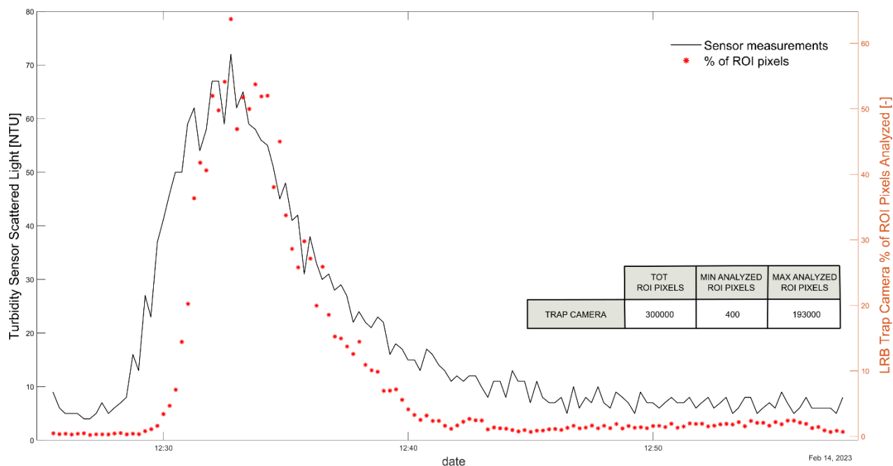
Figure 19: Comparison of turbidimeter measurements (line in black) and number of analyzed ROI pixels in LRB trap camera data (“*” symbols in red) during the short-term experiment of February 2023.
