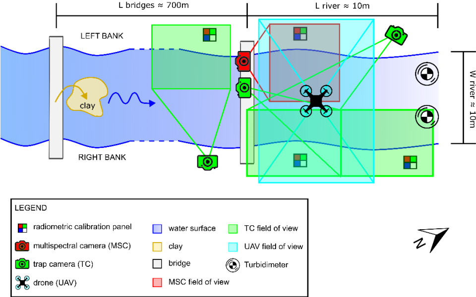
Figure 4: Plan of the monitored river section during the field experiment, showing the generated synthetic turbidity events, using kaolin clay tracer.
