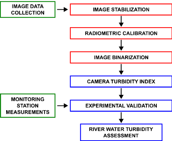
Figure 7: Image processing procedure workflow.
