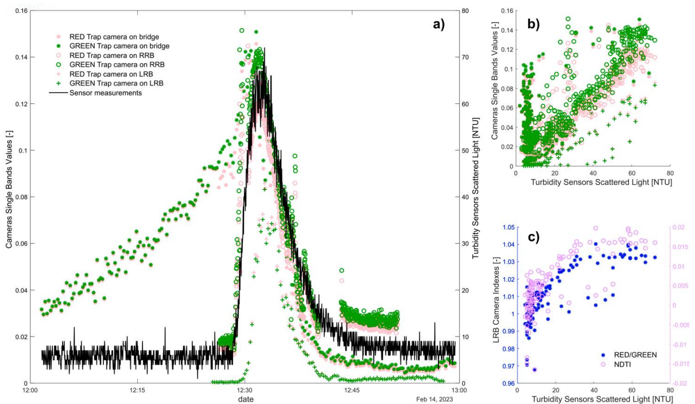
Figure 12: Comparison between turbidimeter measurements, red and green band values from all the trap cameras installed on site; b) Scatter plot of all the cameras green band signal and red band signal ; c) Scatter plot of the NDTI and Red/Green indexes from the trap camera installed on the left riverbank (LRB). The colour schemes used in this figure are accessible to persons with colour vision deficiencies.
