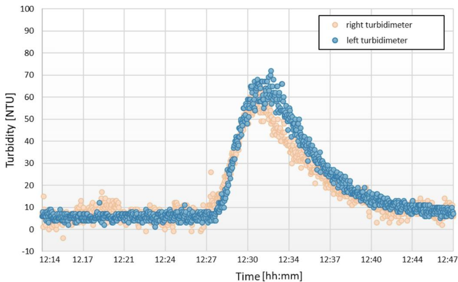
155 Figure 5: Optical measurements of turbidity, using two turbidimeters installed on the right and the left riverbed sides during the experiment. The colour schemes used in this figure are accessible to persons with colour vision deficiencies.
