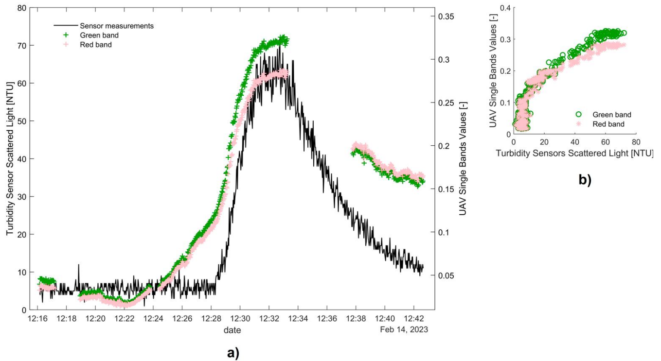
Figure 13: a) Comparison between turbidimeter measurements and data from the UAV camera; b) Scatter plot of the variables. The colour schemes used in this figure are accessible to persons with colour vision deficiencies.
