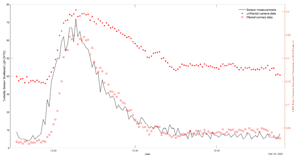
Figure 20: Comparison of turbidimeter measurements (line in black) and the standard deviation of ROI pixels intensity in LRB trap camera red band filtered (“o”symbols in red) and unfiltered (“*”symbols in red) data, during the short-term experiment of February 2023.
