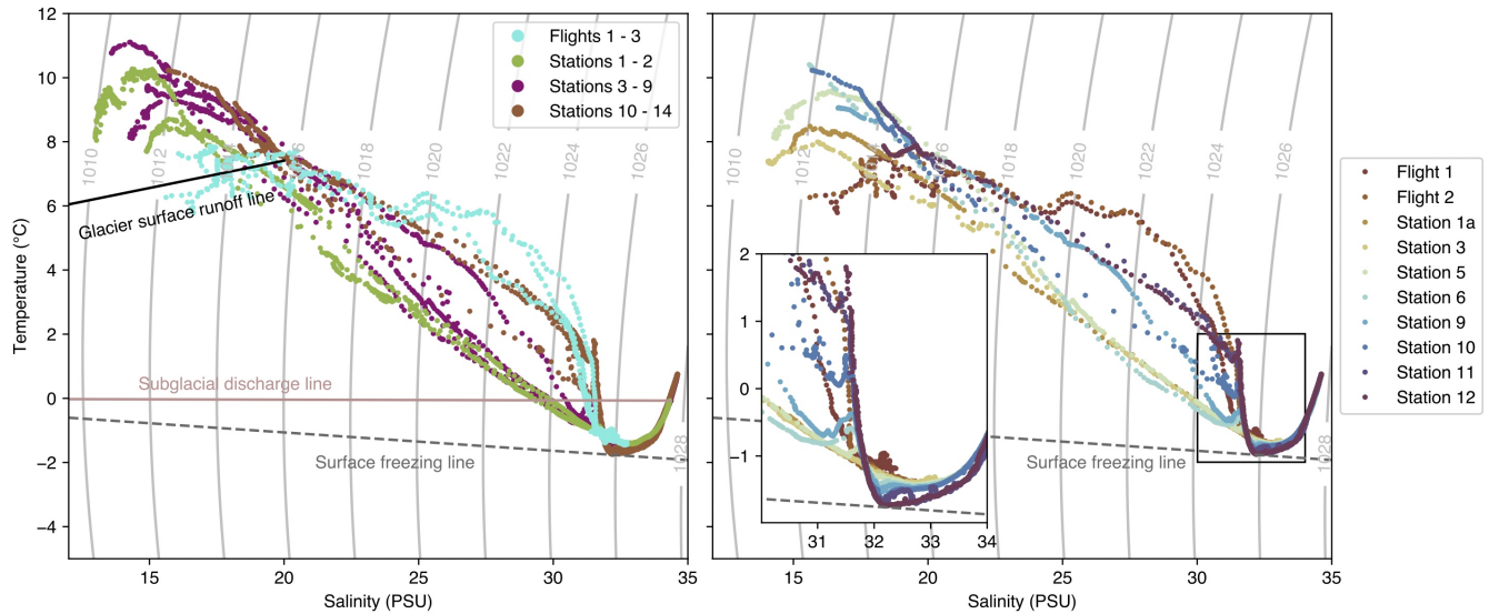
Figure 3. Temperature-salinity values of the profiles measured at all the stations grouped (a) and selected stations (b). Both plots include density lines ( \text{kg/m}^3 ) and the surface freezing line. The cluster plot includes a glacier surface runoff line connecting the surface waters with the glacial surface runoff and a subglacial discharge line connecting deep waters with subglacial discharge.
