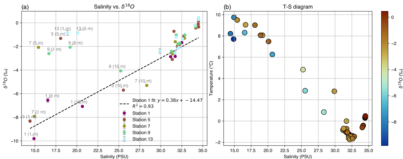
Figure 6. (a) The relationship between salinity and \delta^{18}\text{O} , with data points color-coded based on station and labels indicating station numbers and depts for points with salinity below 29. A dashed black line indicates the linear fit for station 1, with the corresponding equation and R^2 value shown in the legend. (b) T-S diagram with \delta^{18}\text{O} indicated with a color gradient. AC
