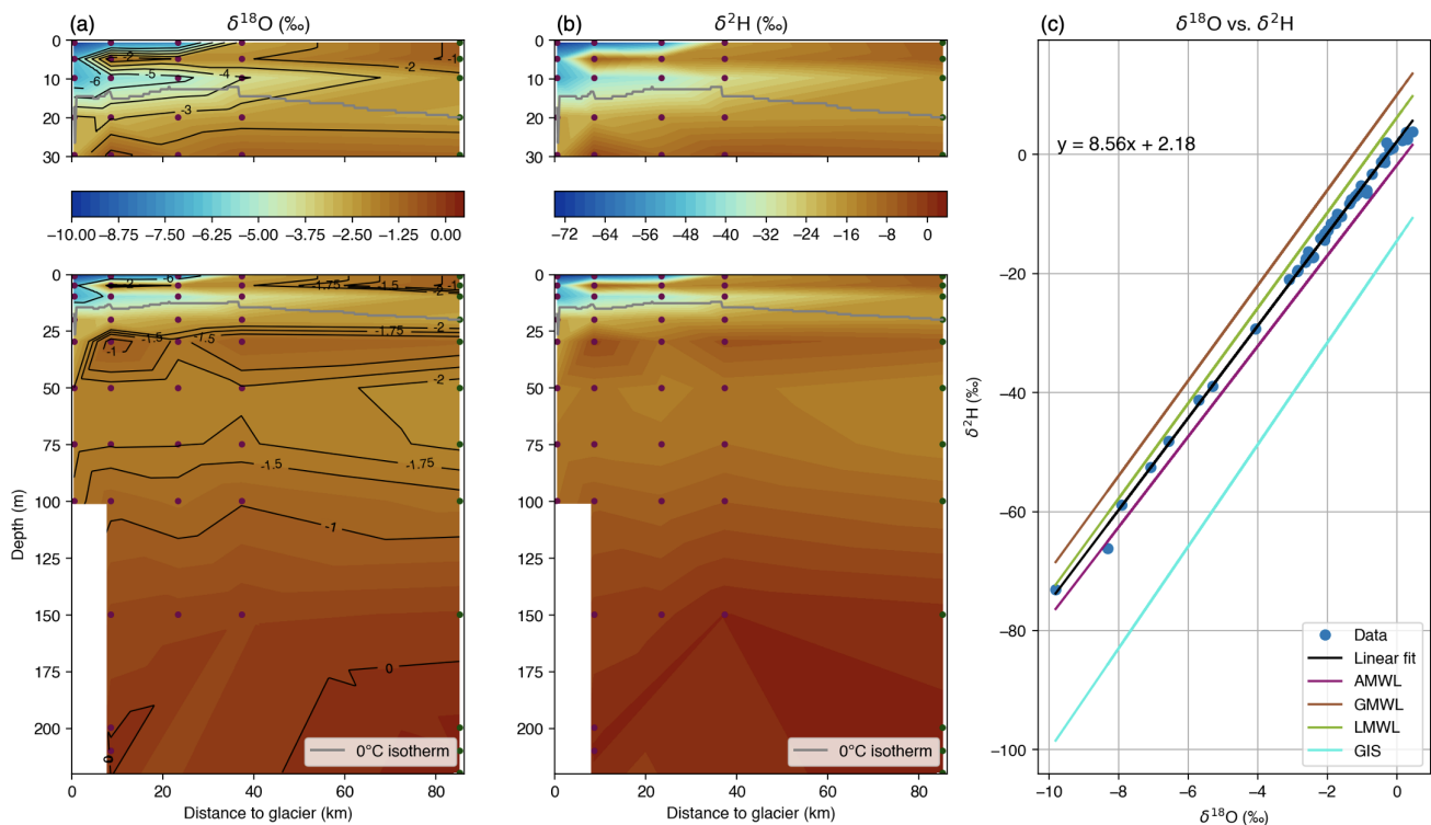
Figure 5. Sections of \delta^{18}\text{O} (a) AC and \delta^2\text{H} (b) AC extending from 0.5 to 87 km from the glacier terminus, and a plot with the \delta^{18}\text{O} values plotted against the \delta^2\text{H} values (c) AC . All the values are represented in units of ‰. In sections (a) and (b), the dark purple and dark green dots represent the measurement data collected on August 14th and August 15th, respectively. Additionally, a 0 °C isotherm is plotted to highlight the freshwater freezing point. Contours with varying intervals have been added to (a). the contour plots, the black dots represent the profile transects rev2 on which the sections rev2 profiles rev2 are based, and the grey line the 0 °C isotherm. Two contours have also been added to the \delta^{18}\text{O} profile. AC In the rightmost plot, a black solid line represents the linear fit of the data points, plotted alongside the AMWL, the GMWL, the LMWL (Willcox et al. (2023)) and the GIS line (Rysgaard et al. (2024)).
