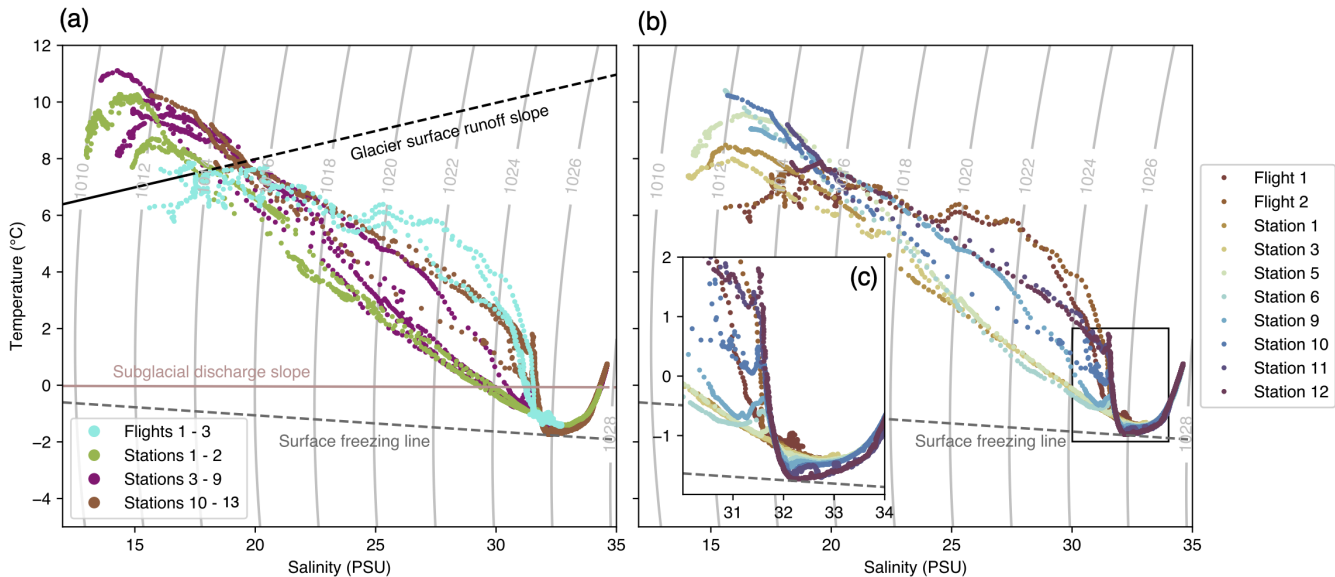
Figure 3. Temperature-salinity values of the profiletransects rev2 measured at all the stations grouped (a)elustered (left) rev1 and selected stations (b)(right) rev1 . Both plots include density lines (kg/m³) and the surface freezing line. The cluster plot includes a glacier surface rev2 runoff slope connecting the surface waters with the glacial surface rev2 runoff and a subglacial discharge slopemixing-line rev2 connecting deep waters with subglacial discharge.
