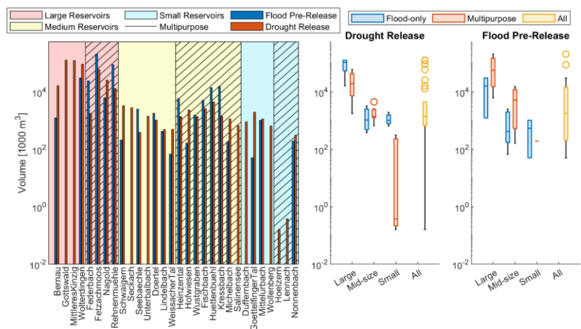
555 Figure 14. Comparisons of total releases for drought protection and pre-releases for flood protection in the optimized combined operation model over the simulation period. Reservoirs with no flood pre-release volumes were omitted from the respective plots.
