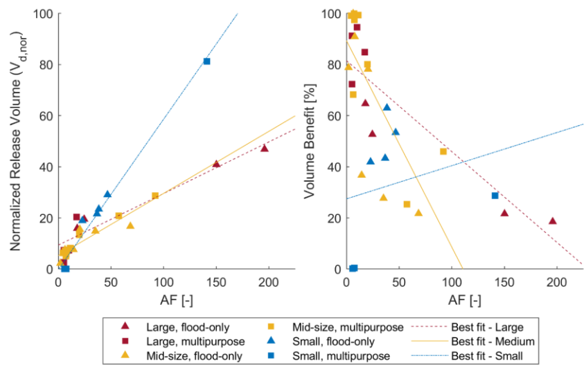
560 Figure 15. The relation between AF (relative water availability) and normalized release volume ( V_{d,nor} ; left) and volume benefit (B; right).
