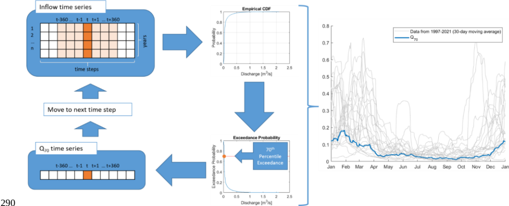
Figure 3. Example calculation of the Q_{70} time series.
