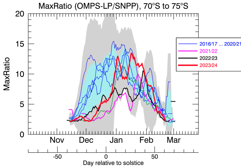
Figure 4. The maximum radiance ratio between the measured and background limb radiance from OMPS-LP for each of the SH NLC seasons. The thick lines indicate zonally and daily mean maximum radiance ratios between 70 °S to 75°S for 2021/22 (magenta), 2022/2023 (black) and 2023/24 (red). All seasons before are displayed as thin blue lines. The blue (grey) shaded region contains the averaged maximum radiance ratio for the years 2016/17 to 2020/21 \pm one (three) standard deviations from this period. All occurrence frequencies are smoothed over 5 days and the day of solstice is December 21.
