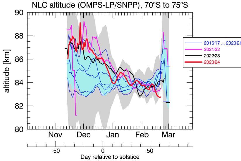
Figure 5. Altitude of the NLCs determined from OMPS-LP measurements. The thick lines indicate zonally and daily mean maximum radiance ratios between 70 °S to 75°S for 2021/22 (magenta), 2022/23 (black) and 2023/24 (red). All seasons before are displayed as thin blue lines. Blue (grey) areas indicate the mean NLC altitude from 2016/17 to 2020/21 \pm one (three) standard deviation. All data is smoothed over 5 days.
