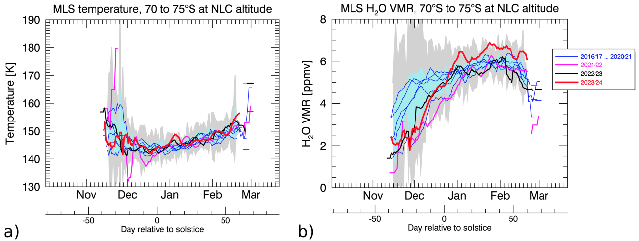
Figure 3. a) MLS temperature between 70°S - 75°S at NLC altitude determined from OMPS-LP measurements. The thick lines show the SH seasons 2021/22 (magenta), 2022/23 (black) and 2023/24 (red), respectively. All seasons before are displayed as thin blue lines. Blue (grey) areas indicate the averaged temperature from 2016/17 to 2020/21 \pm one (three) standard deviations. b) The same for MLS water vapour mixing ratios. All data is smoothed over 5 days.
