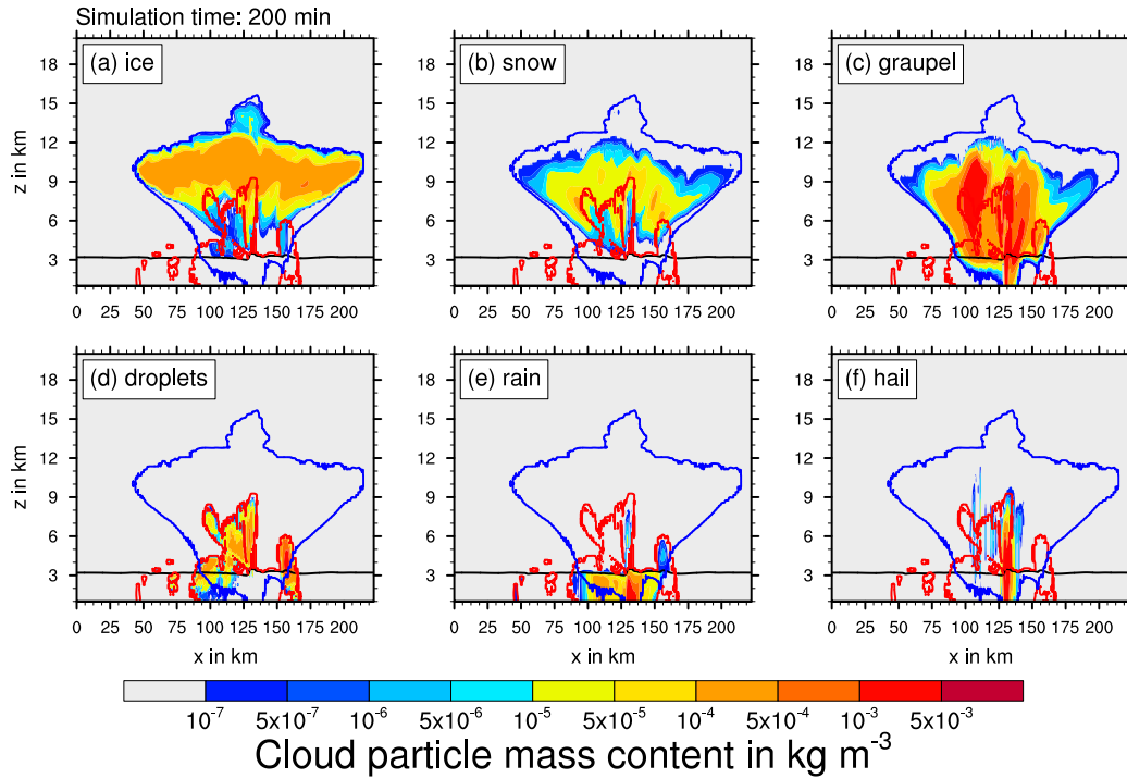
Figure 5. Vertical slice through domain center at 200 min simulation time. Mass content of (a) total ice, (b) snow, (c) graupel, (d) cloud droplets, (e) raindrops and (f) hail. The black line indicates the melting temperature level. The red and blue contour show the critical LWC and IWC value of 0.1 \text{ mg m}^{-3} , respectively.
