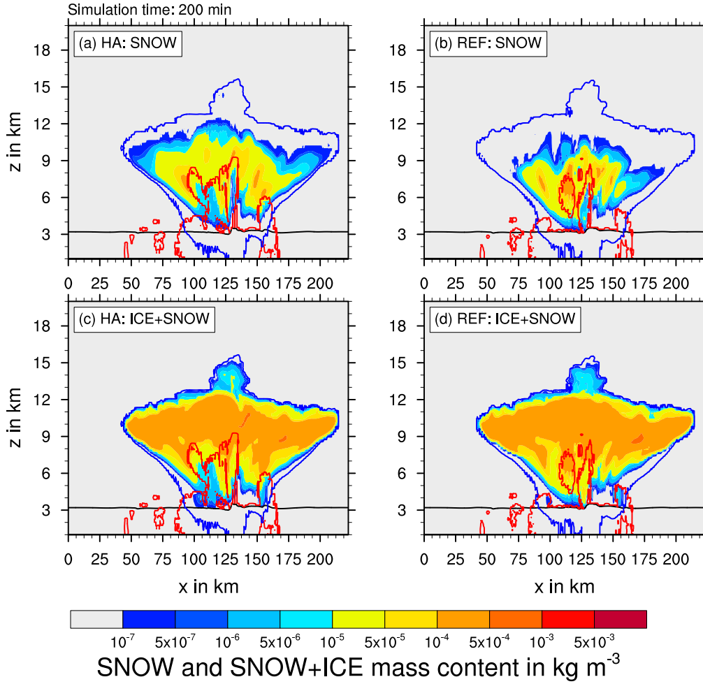
Figure 7. Vertical slice through domain center at 200 min simulation time. Mass content of snow for (a) ice modes scheme (HA) and (b) standard SB (REF) as well as the sum of all cloud ice and snow for (c) HA and (d) REF. The black line indicates the melting temperature level. The red and blue contour show the critical LWC and IWC value of 0.1 \text{ mg m}^{-3} , respectively.
