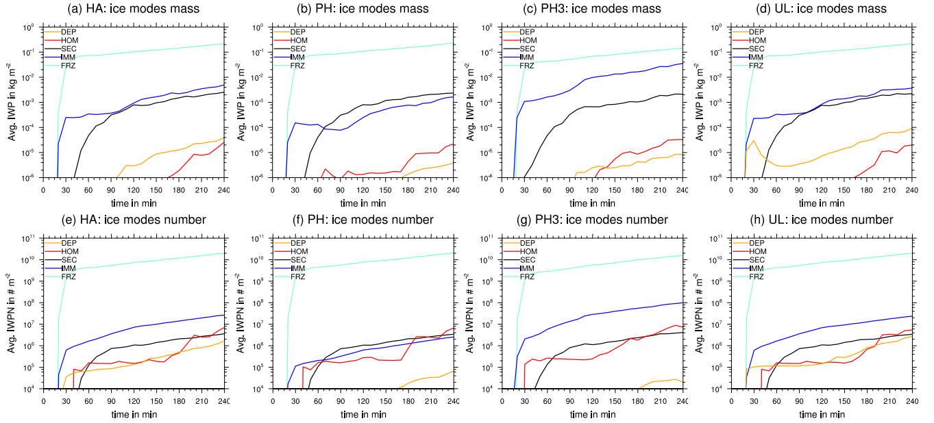
Figure 4. Temporal evolution of the horizontally averaged (ice) water path for each ice for heterogeneous ice nucleation scheme (a) HA, (b) PH, (c) PH3 and (d) UL. Average integrated number concentration for each ice mode for e) HA, (f) PH, (g) PH3 and (h) UL.
