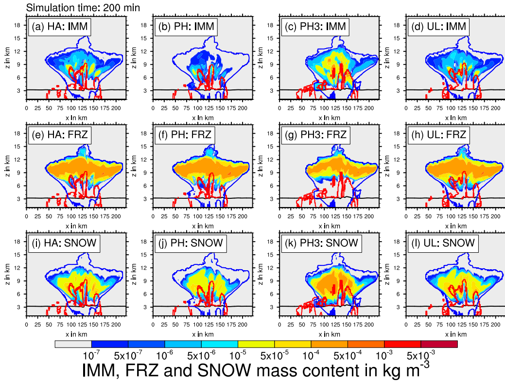
Figure 8. Vertical slice through domain center at 200min simulation time comparing mass content of IMM (a-d), FRZ (f-h) and snow (i-l) for the experiments HA (a,e,i), PH (b,f,j), PH3 (c,g,k) and UL (d,h,l). The black line indicates the melting temperature level. The red and blue contour show the critical LWC and IWC value of 0.1 \text{ mg m}^{-3} , respectively.
