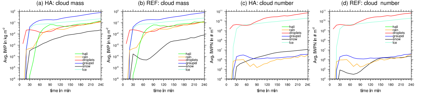
Figure 3. Temporal evolution of the horizontally averaged ice water path for each hydrometeor class for (a) ice modes (HA) and (b) reference SB simulation (REF). Temporal evolution of average integrated number concentration for (c) HA and (d) REF. ICE is the sum of all ice modes for HA.
