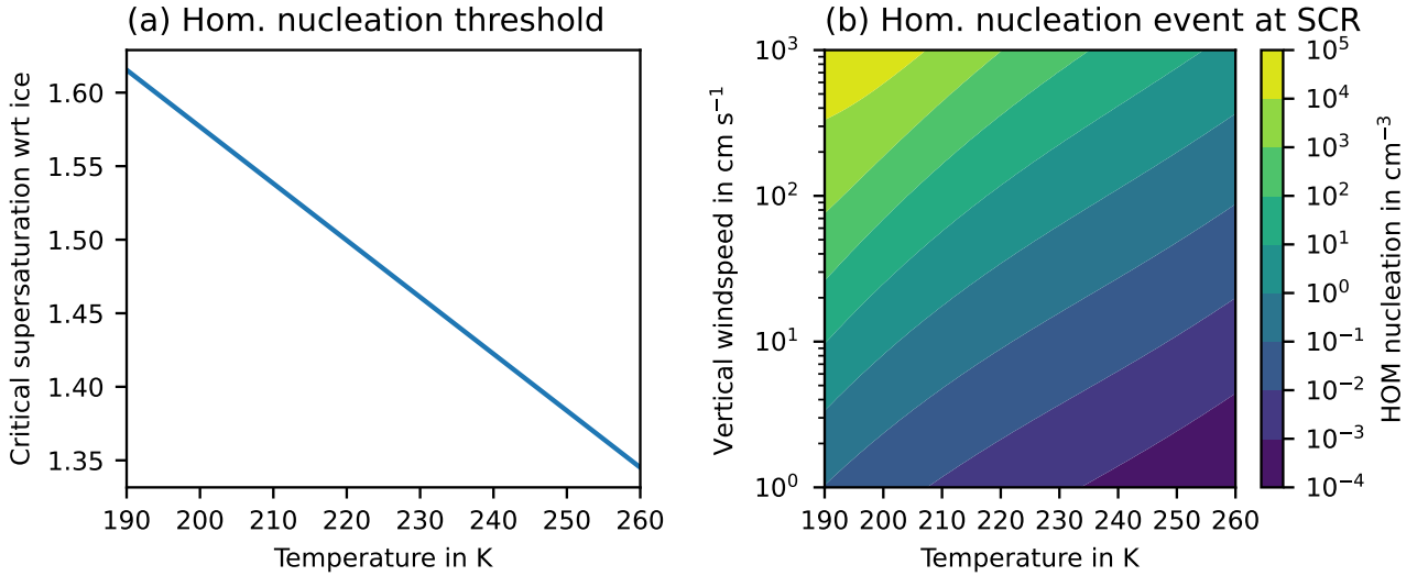
Figure 1. Homogeneous nucleation following Kärcher et al. (2006) for no pre-existing ice. (a) Critical supersaturation S_{cr} serves as a nucleation threshold and (b) number of ice crystals after a homogeneous nucleation event at S_{cr} .
