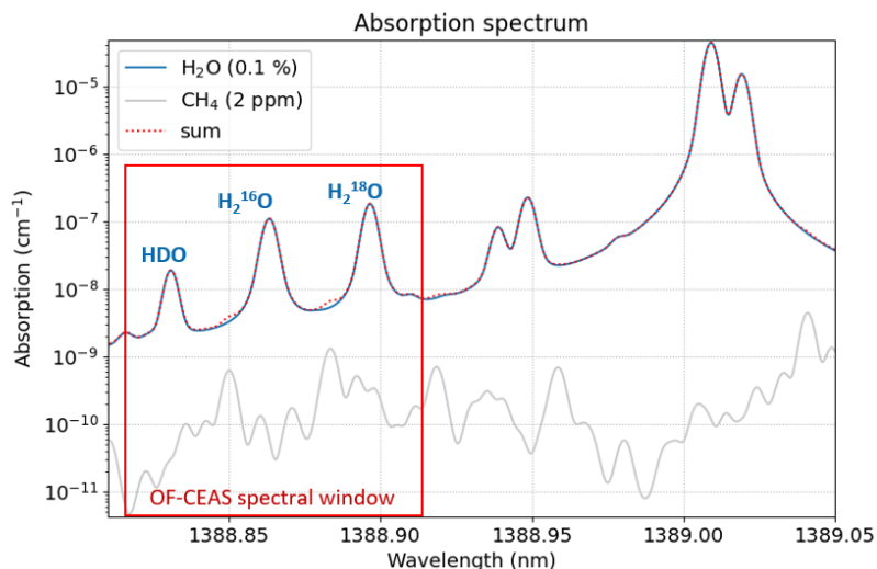
75 Figure 1 : Absorption spectrum of the three target isotopologues HDO, H 2 16 O and H 2 18 O retrieved from HITRAN database. The total absorption spectrum is plotted with the red dotted line, considering 0.1% of water vapour (blue line) and 2 ppm of methane (grey line). The red rectangle indicates the OF-CEAS spectral window by current tuning on a 1389 nm distributed feedback laser diode.
