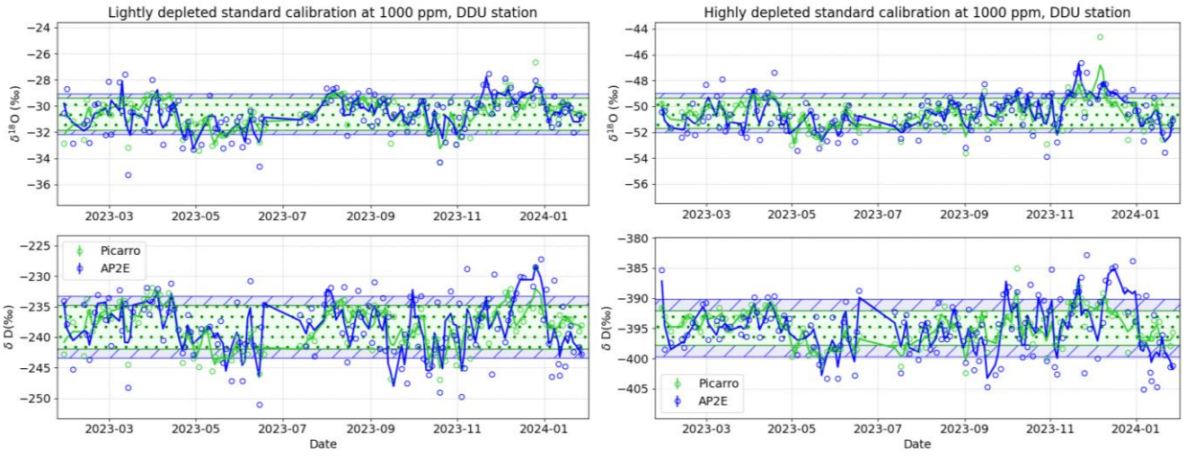
Figure 5 : \delta^{18}\text{O} and \delta\text{D} drift calibration of the AP2E OF-CEAS (blue circles) and Picarro CRDS (green circles) analysers for two in-house isotopic standards named AO1 (lightly depleted standard) and FP5 (highly depleted standard). Each calibration point represents the average of the final 5 to 10 minutes of humidity plateaus, with a humidity setpoint of 1000 ppm. The blue line (resp. green line) corresponds to the AP2E OF-CEAS (resp. Picarro CRDS) dataset smoothed over a 5-point window. The blue hatched (resp. green dotted) area corresponds to the standard deviation of the AP2E OF-CEAS (resp. Picarro CRDS) calibrations, with the corresponding values displayed in Table 1.
