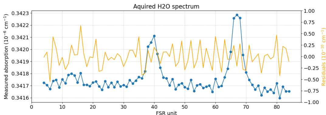
90 Figure 2 : Measured spectrum of the OF-CEAS analyser (blue dots) after a long drying period using a N 2 gas cylinder, resulting in a minimal water concentration of 3 ppm. The residuals after fitting are expressed in cm -1 (yellow line) and obtained from a 600 ms wavelength scan and a fit calculation time of less than 52 ms,
