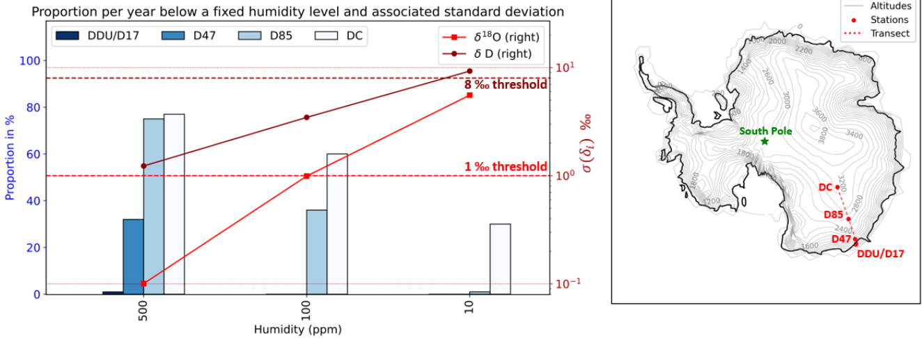
315 Figure 8 : On the left, histogram representing the year fraction (expressed in %) below a fixed humidity content for 4 sites situated along the transect. For each humidity, we plotted the associated standard deviation after 24 hours \sigma(\delta_i) as predicted by the Allan deviation study for \delta^{18}\text{O} and \delta\text{D} . The dotted horizontal lines represent the \delta^{18}\text{O} and \delta\text{D} upper thresholds for the standard deviation to confidently study the diurnal cycle. These thresholds are set at a value 10 times lower than the amplitude of the diurnal cycle, to ensure a correct signal resolution (see discussion in the text). On the right, map with the location of the 4 instrumented sites for the AWACA deployment.
