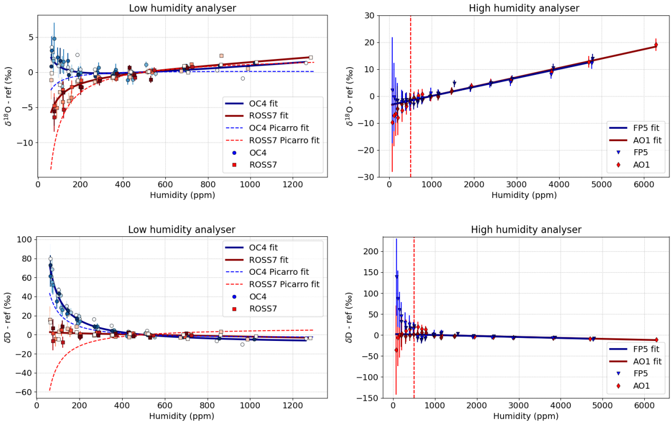
255 Figure 6 : Humidity dependency calibration of the low-humidity OF-CEAS analyser from 50 to 1300 ppm for \delta^{18}O (top left) and \delta D (bottom left) and of the high-humidity analyser from 50 to 6500 ppm for \delta^{18}O (top right) and \delta D (bottom right). The y-axis are shown with different scales. All curves are referenced to the isotopic composition measured at 500 ppm (left panel) and 1000 ppm (right panel), denoted “ref” on the y-axis. Shades of blue and red indicate various calibration sequences in time. Additional dashed curves correspond to the typical humidity dependency of a Picarro instrument measured in the lab, for comparison. The vertical 260 dashed line in the right panels corresponds to the humidity above which 99% of the humidity signal at DDU is observed.
