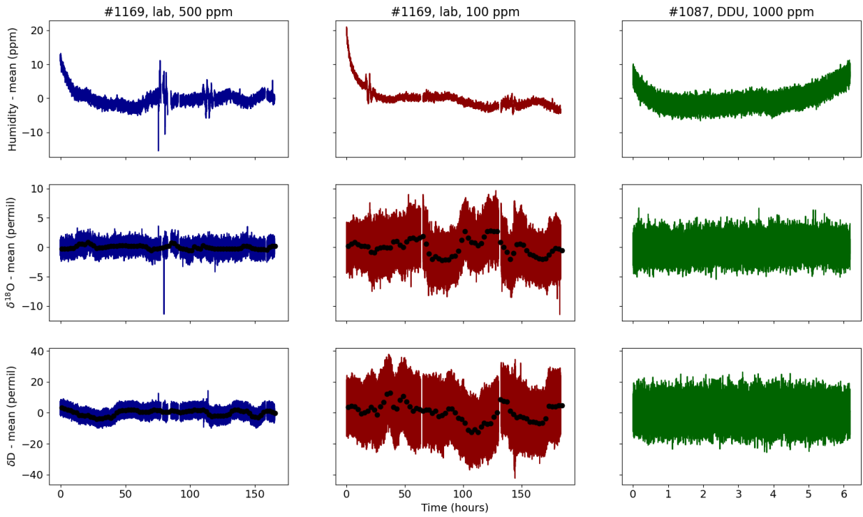
Figure 3 : From top to bottom, measured humidity, \delta^{18}\text{O} and \delta\text{D} used for the Allan deviation study, referenced to their mean value. The two first columns correspond to one-week calibrations in the lab with the low-humidity analyser at 500 ppm (first column, blue) and at 100 ppm (second column, red). The third column (green) corresponds to the data obtained at 1000 ppm from the high-humidity analyser in the field, over 6 hours. Coloured curves show the raw signal, and the black circles the signal averaged on a 8 000 s window.
