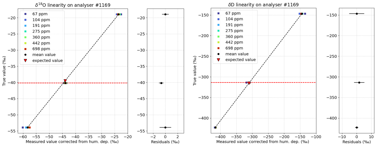
290 Figure 7: Correspondence between the true isotopic value and the measured, corrected value of \delta^{18}\text{O} and \delta\text{D} for 7 humidity steps ranging from 67 to 698 ppm with three VSMOW-SLAP calibrated standards OC4, TD3 and ROSS7 (coloured squares), with the corresponding average values calculated across the humidity range (black circles). The linear calibration slope (black dashed line) results from the average value of the OC4 and ROSS7 standards only, while the TD3 standard (true value indicated with the red dashed line) is used to quantify the instrument accuracy and precision. The red triangle indicates the expected value of the TD3 standard using the calibration slope.
