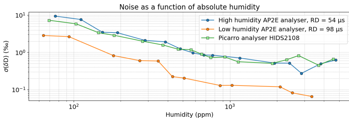
Figure 9 : Noise on \delta D with an averaging time of 2 min as a function of the humidity for the two OF-CEAS analysers from AP2E and the Picarro analyser currently installed at Dumont d'Urville station. The noise is obtained from short-term Allan deviations at \tau = 2 min calculated during each step of the humidity dependency calibration.
