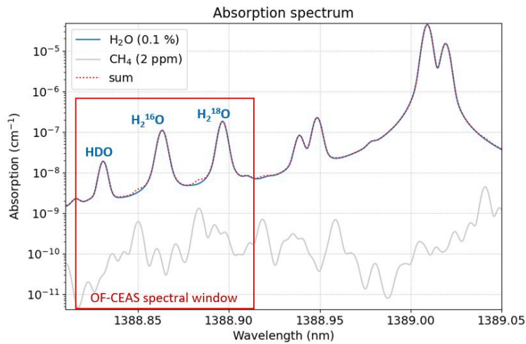
75 Figure 1 : Absorption spectrum of the three target isotopologues HDO, H 2 16 O and H 2 18 O retrieved from HITRAN database. The total absorption spectrum is plotted with the red dotted line, considering 0.1% of water vapour (blue line) and 2 ppm of methane (grey line). The red rectangle indicates the OF-CEAS spectral window by current tuning on a 1389 nm distributed feedback laser diode.
