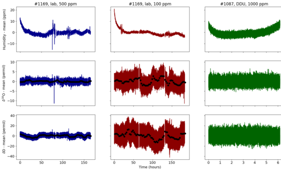
Figure 3 : From top to bottom, measured humidity, \delta^{18}O and \delta D used for the Allan deviation study, referenced to their mean value. The two first columns correspond to one-week calibrations in the lab with the low-humidity analyser at 500 ppm (first column, blue) and at 100 ppm (second column, red). The third column (green) corresponds to the data obtained at 1000 ppm from the high-humidity analyser in the field, over 6 hours. Coloured curves show the raw signal, and the black circles the signal averaged on a 8 000 s window.
