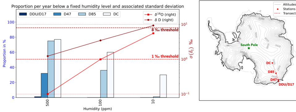
Figure 8 : On the left, histogram representing the year fraction (expressed in %) below a fixed humidity content for 4 sites situated along the transect. For each humidity, we plotted the associated standard deviation after 24 hours \sigma(\delta_i) as predicted by the Allan deviation study \sigma(\delta_i) after 24 hours for \delta^{18}\text{O} and \delta\text{D} . The dotted horizontal lines represent the \delta^{18}\text{O} and \delta\text{D} upper thresholds for the standard deviation to confidently study the diurnal cycle. These thresholds are set at a value 10 times lower than the amplitude of the diurnal cycle, to ensure a correct signal resolution (see discussion in the text). For diurnal cycle tracking, in red and dark red, respectively (see discussion in the text). On the right, map with the location of the 4 instrumented sites for the AWACA deployment.
