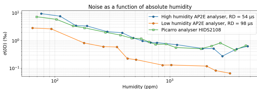
Figure 9 : Noise on \delta D with an averaging time of 2 min as a function of the humidity for the two OF-CEAS analysers from AP2E and the Picarro analyser currently installed at Dumont d'Urville station. The noise is obtained from short-term Allan deviations at \tau = 2 min calculated during each step of the humidity dependency calibration.
