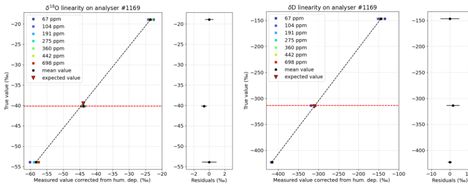
295 Figure 7: Correspondence between the true isotopic value and the measured, corrected value of \delta^{18}\text{O} and \delta\text{D} for 7 humidity steps ranging from 67 to 698 ppm with three VSMOW-SLAP calibrated standards OC4, TD3 and ROSS7 (coloured squares), with the corresponding average values calculated across the humidity range (black circles). The linear calibration slope (black dashed line) results from the average value of the OC4 and ROSS7 standards only, while the TD3 standard (true value indicated with the red dashed line) is used to quantify the instrument accuracy and precision. The red triangle indicates the expected value of the TD3 standard using the calibration slope.
