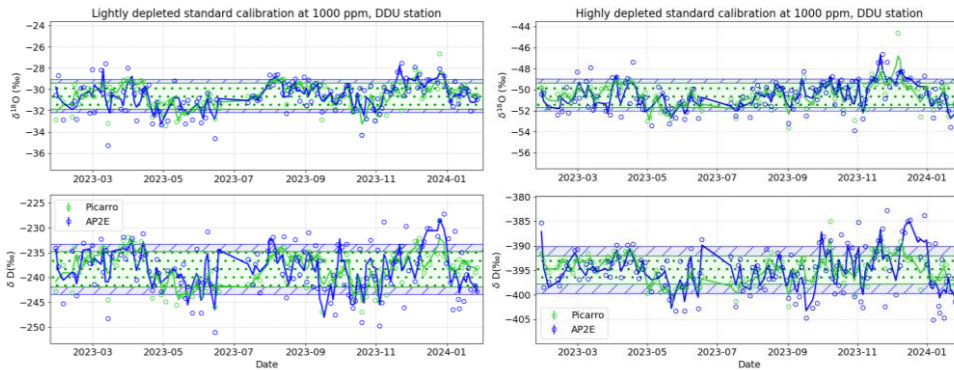
Figure 5: \delta^{18}\text{O} and \delta D drift calibration of the AP2E OF-CEAS (blue circles) and Picarro CRDS (green circles) laser spectrometers analysers for two in-house isotopic standards named AO1 (lightly depleted standard) and FP5 (highly depleted standard). Each calibration point represents the average of the final minimum 5 to 10 minutes of 1000 ppm-humidity plateaus, with a humidity setpoint of 1000 ppm. The blue line (resp. green line) corresponds to the AP2E OF-CEAS (resp. Picarro CRDS) dataset smoothed over a 5-point window. The blue hatched (resp. green dotted) area corresponds to the standard deviation of the AP2E OF-CEAS (resp. Picarro CRDS) calibrations, with the corresponding values displayed in Table 1, and the error bars correspond to the associated standard deviation.
