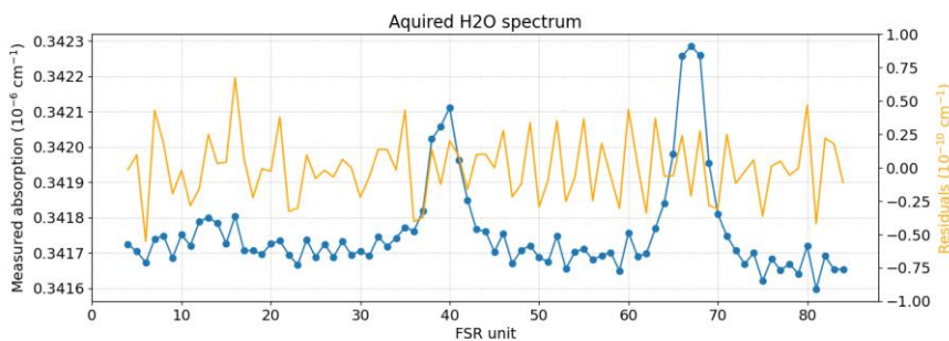
90 Figure 2 : Measured spectrum of the OF-CEAS analyser (blue dots) after a long drying period using a N 2 gas cylinder, resulting in a minimal water concentration of 3 ppm. The residuals after fitting are expressed in cm -1 (yellow line) and obtained from a 600 ms wavelength scan and a fit calculation time of less than 52 ms,
