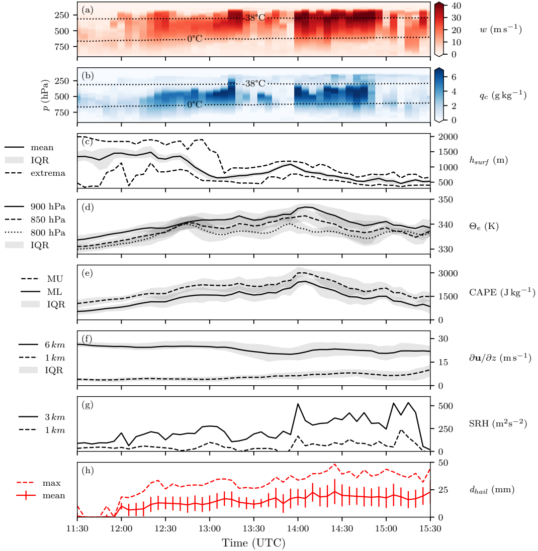
Figure 4. Temporal evolution of a selection of storm-centered variables (within the 50 \times 50 grid-point box) along the red storm track in Fig. 3. The horizontal maxima of the respective variables are shown as colored pixels for the 3D variables (a) vertical velocity w , and (b) cloud water content q_c , both within the storm mask. (c) shows the distribution of topographical height within the storm mask (IQR as shading), (d) and (e) show the mean values of \Theta_e and CAPE in the inflow region, respectively (respective IQR as shading). (f) shows the mean vertical 0 – 1 km and 0 – 6 km wind shear in the inflow region (respective IQR as shading). (g) shows the storm maximum 0 – 1 km and 0 – 3 km SRH evolution. (h) shows the maximum and mean hail diameter values within the storm mask as reported by HAILCAST, with the standard deviation indicated by error bars. Panels (a) and (b) also feature two dotted ambient isotherms. The inflow region encompasses a 20 \times 20 \text{ km}^2 square box, centered 20 km ahead of the storm. All values are from a selected storm of one ensemble member of the COSMO-1E simulation.
