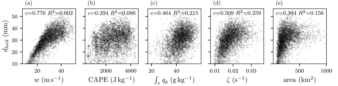
Figure 8. Scatter matrix with per time step storm-environmental parameters (considered in box with 50×50 gridpoints 50 × 50 grid-points ) from n = 100 storms with lifespans > 2.5 h that reach updraft velocities > 25 \text{ m s}^{-1} . All values but the area are the per-time step maxima found within the environmental box. Correlation and R^2 values are indicated in each permutation. COSMO-1E simulation, all 11 members.
