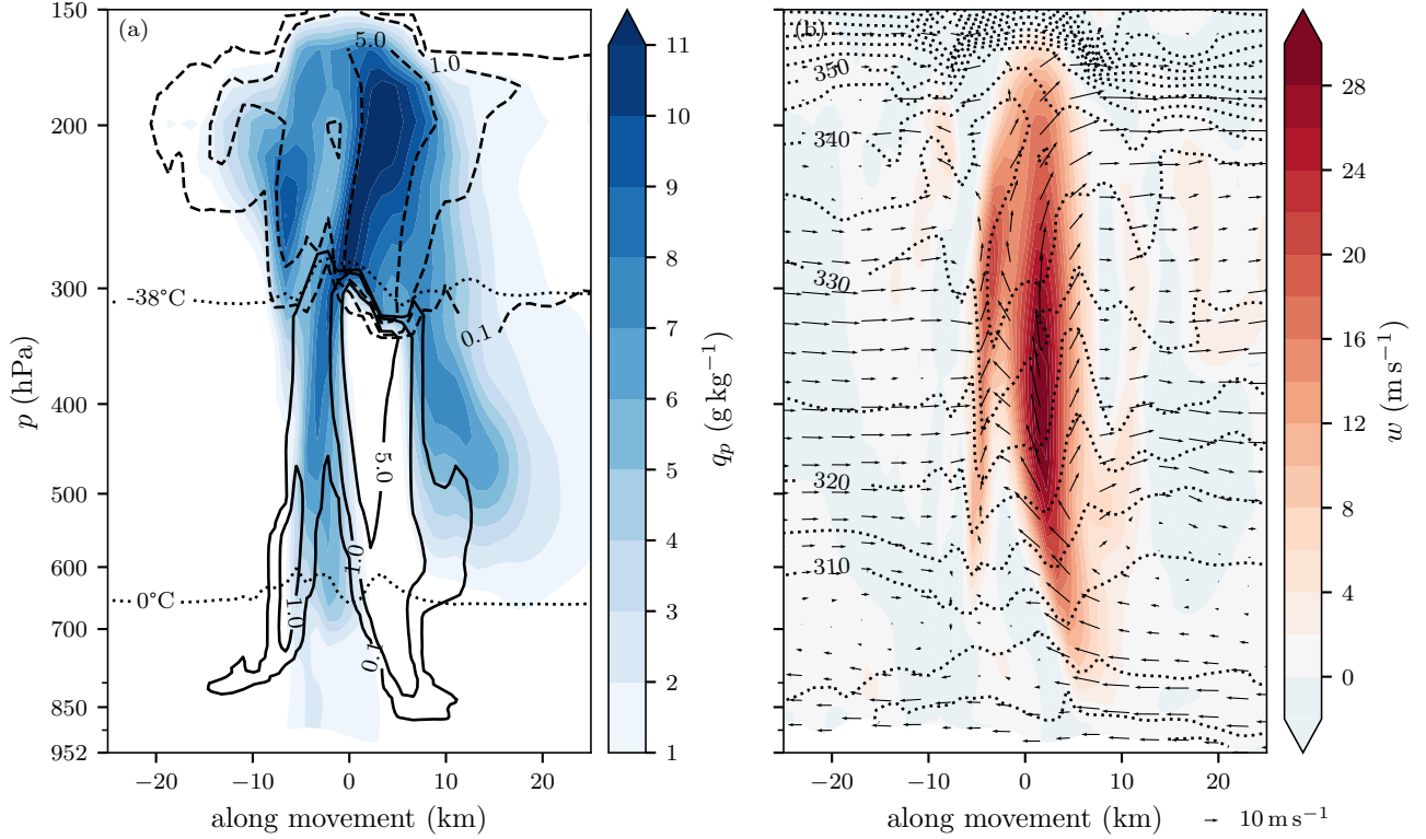
Figure B1. Same as Fig. 5, for the most intense time step of a selected storm in one member of the COSMO-IE simulation .
