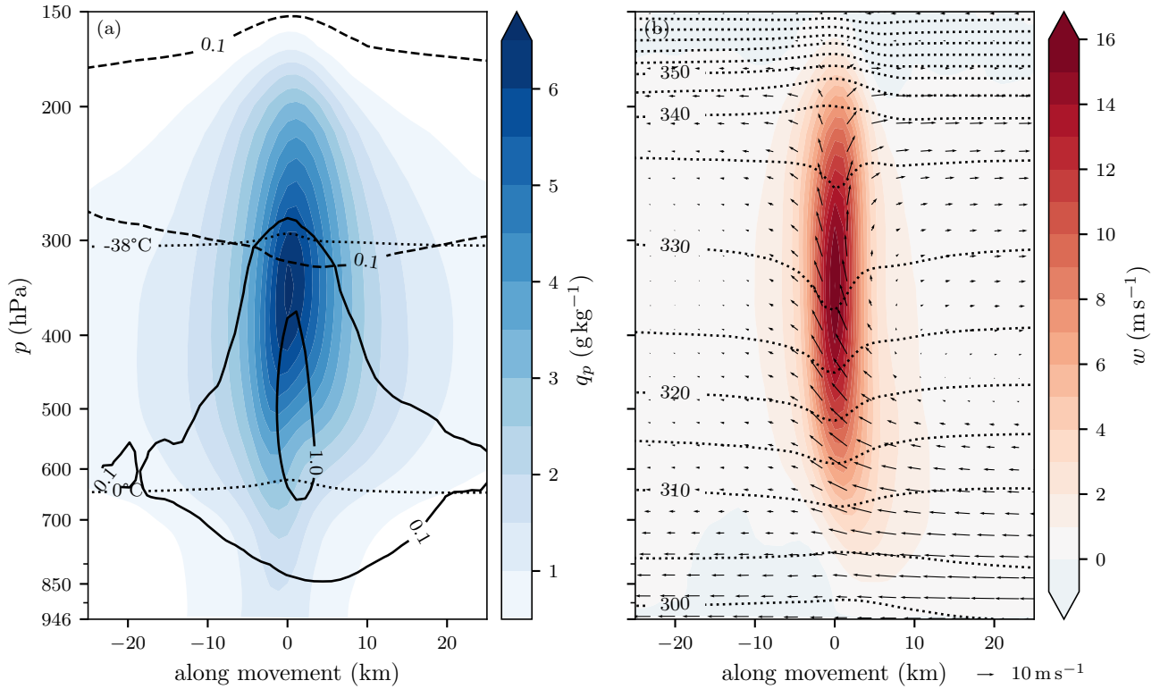
Figure 5. Vertical cross-section ( single plane through storm center ) along the propagation direction of the storm-centered composite of n = 100 storms with lifespans > 2.5 h at time steps with w > 25 \text{ ms}^{-1} , identified in all COSMO-1E ensemble members. The storm is moving to the right and the center (0 km) represents the storm track center. (a) Filled contours denote the total precipitating hydrometeor mixing ratio, solid and dashed contours represent cloud water and cloud ice mixing ratios ( \text{g kg}^{-1} ), respectively, while the 0^\circ\text{C} and -38^\circ\text{C} levels are shown as dotted lines. (b) Vertical wind field (in \text{ms}^{-1} , filled contours), isentropes (in K, dotted contours), and in-plane, storm-relative wind vectors, quivers. Refer to Fig. C1 for the ensemble spread.
