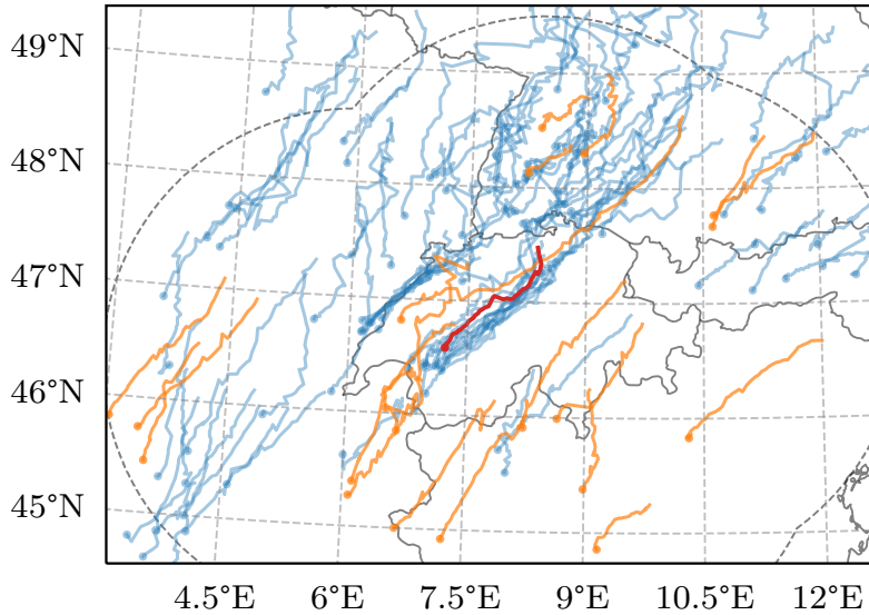
Figure 3. Overview of the 100 tracked storms with lifespans greater than 2.5 h that reach updraft velocities > 25 \text{ ms}^{-1} from all COSMO-IE members (blue). The start of storm tracks is marked with a dot, while the storm selected to be investigated in detail is highlighted in red. Orange tracks indicate the radar-observed tracks on the case study day with lifespans > 2.5 \text{ h} as classified by TRT ( Hering et al., 2004 ; Trefalt et al., 2023 ). The dashed line denotes the extent of the radar domain.
