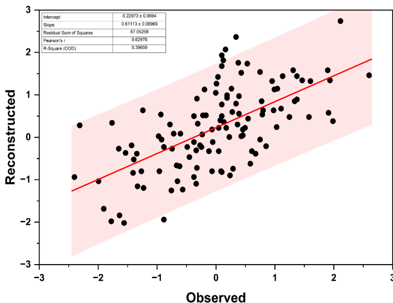
Figure 5. a) Calibration – validation model for the August SPEI9 reconstruction; in (a) the grey line indicates the observed data (CRU TS v. 4.04 dataset, Harris et al., 2020); the red line indicates the reconstructed August SPEI9 over the calibration period and the blue line indicates the reconstructed August SPEI9 over the validation period; and b) regression between the observed and reconstructed August SPEI9 over the period 1900 – 2020.
