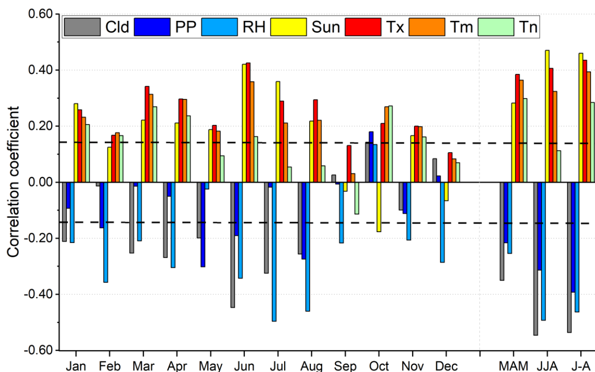
220 Figure 2. The correlation coefficients of \delta^{18}\text{O} chronology from Letea Forest with monthly climate data (cloud cover – Cld, precipitation – PP, relative humidity – RH, sunshine duration – Sun, maximum temperature – Tx, mean temperature – Tm, minimum temperature - Tn) from Sulina meteorological station. Correlation analyses were performed from January to December, but also for March, April, and May (MAM), June, July, and August (JJA), and from January to August (J-A). The black dotted lines represent the significance level at 0.05.
