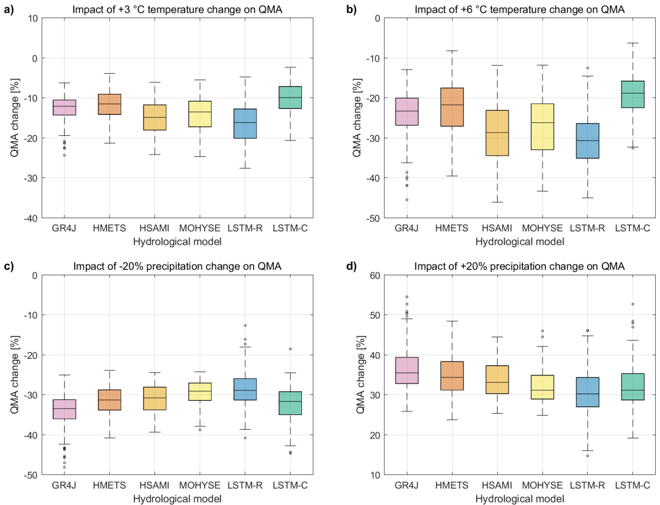
565 Figure 4: Projected mean annual streamflow (QMA) changes for the 4 sensitivity scenarios: temperature increase of +3 °C (a) and +6 °C (b) and precipitation relative change of -20% (c) and +20% (d).
