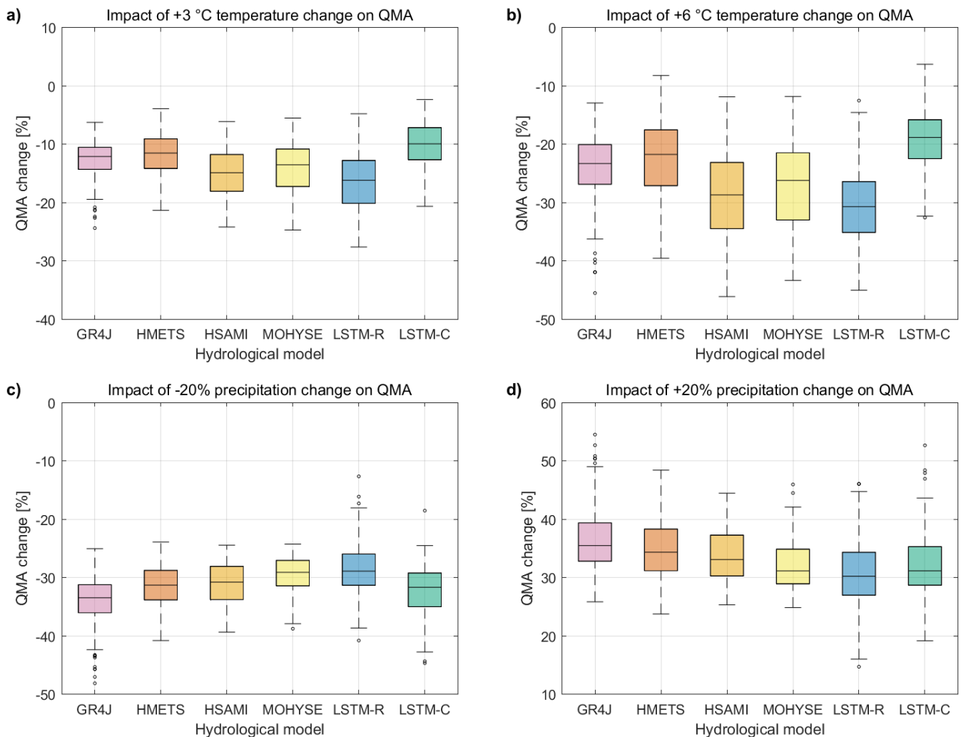
Figure 4: Projected mean annual streamflow (QMA) changes for the 4 sensitivity scenarios: temperature increase of +3 °C (a) and +6 °C (b) and precipitation relative change of -20% (c) and +20% (d).
