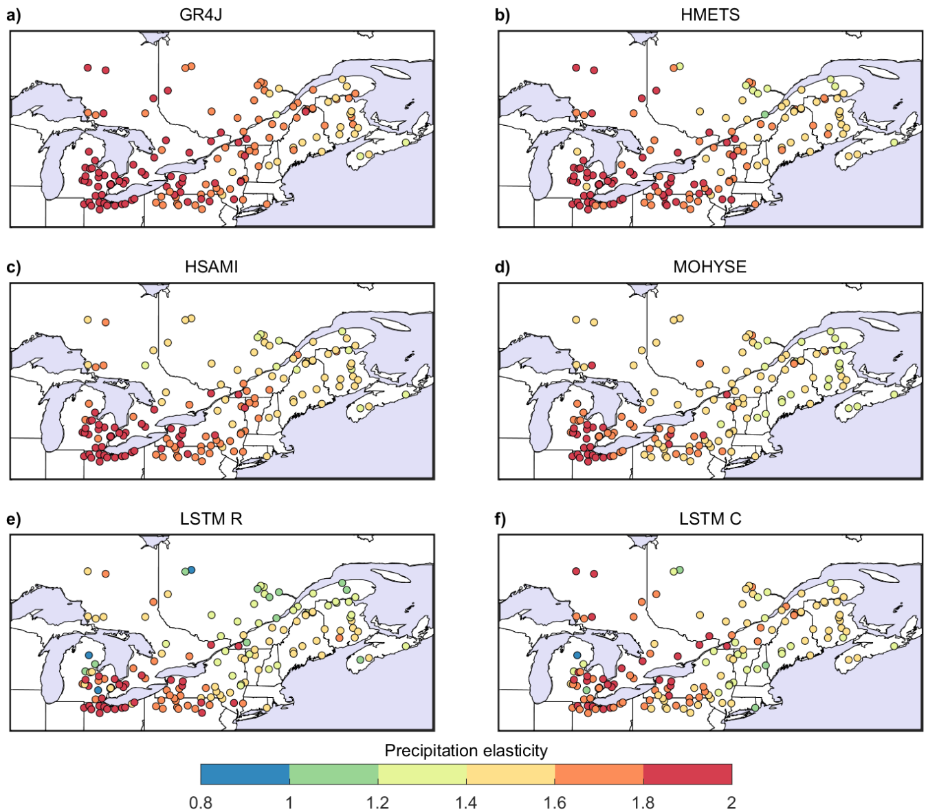
Figure 79: Rainfall elasticity for each of the 148 catchments as evaluated by the six hydrological models.
