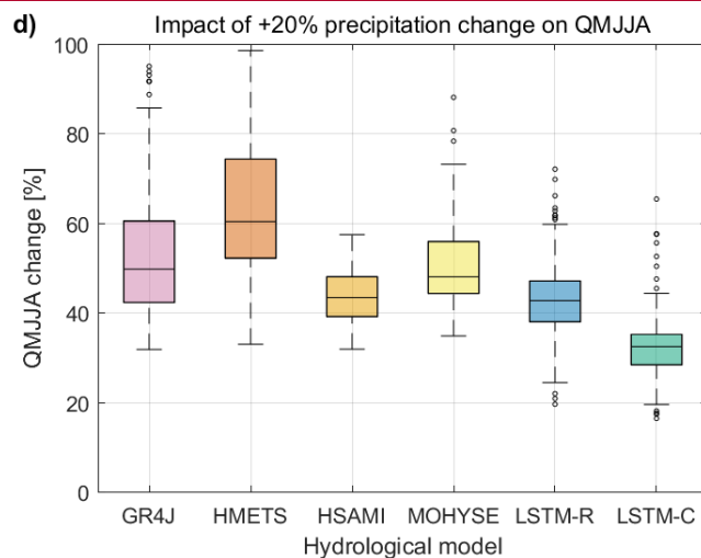
635 Figure 5: Same as Figure 4, but for projected mean summer (JJA) streamflow changes.
