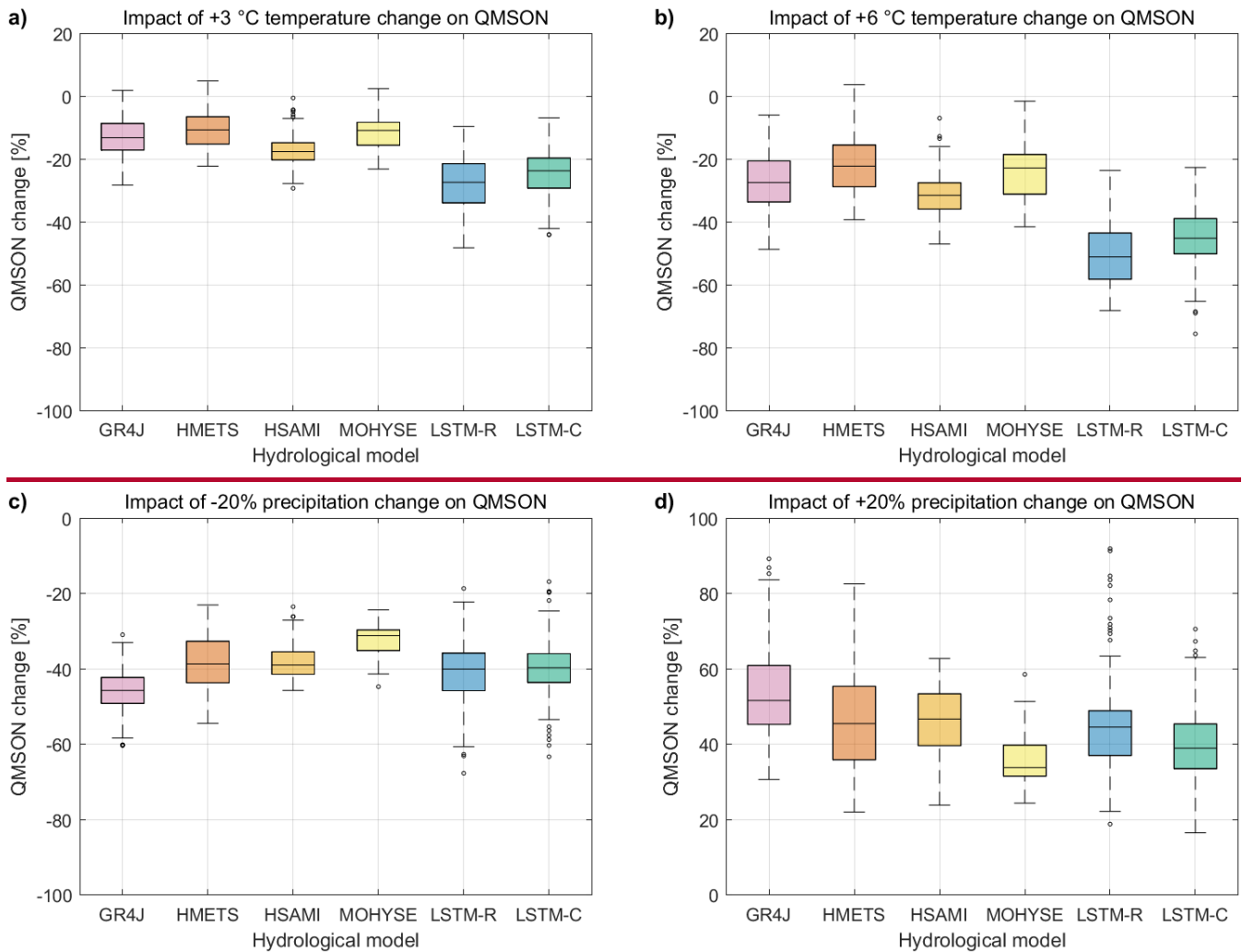
Figure 6: Same as Figure 4, but for projected mean fall (SON) streamflow changes.
