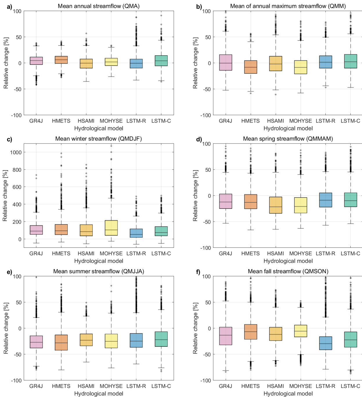
Figure 57: Boxplots of the range of expected change for all 6 streamflow metrics. The boxplots are aggregations of the 22 GCMs and 148 catchments. The boxplots are thus drawn from a distribution of 3,246 points (148 catchments \times 22 GCMs). Note that the y-axis range is different in panel c) than the others due to the much larger values for this period.
