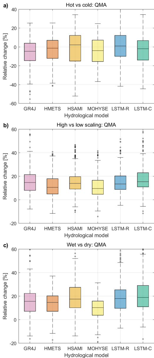
655 Figure 6: Boxplots of % change between two groups of three contrasted climate models. a): hot vs cold models, b): high vs low precipitation scaling models, c): wet vs dry models. The boxplots are drawn from a distribution of 444 points (148 catchments \times 3 climate models).
