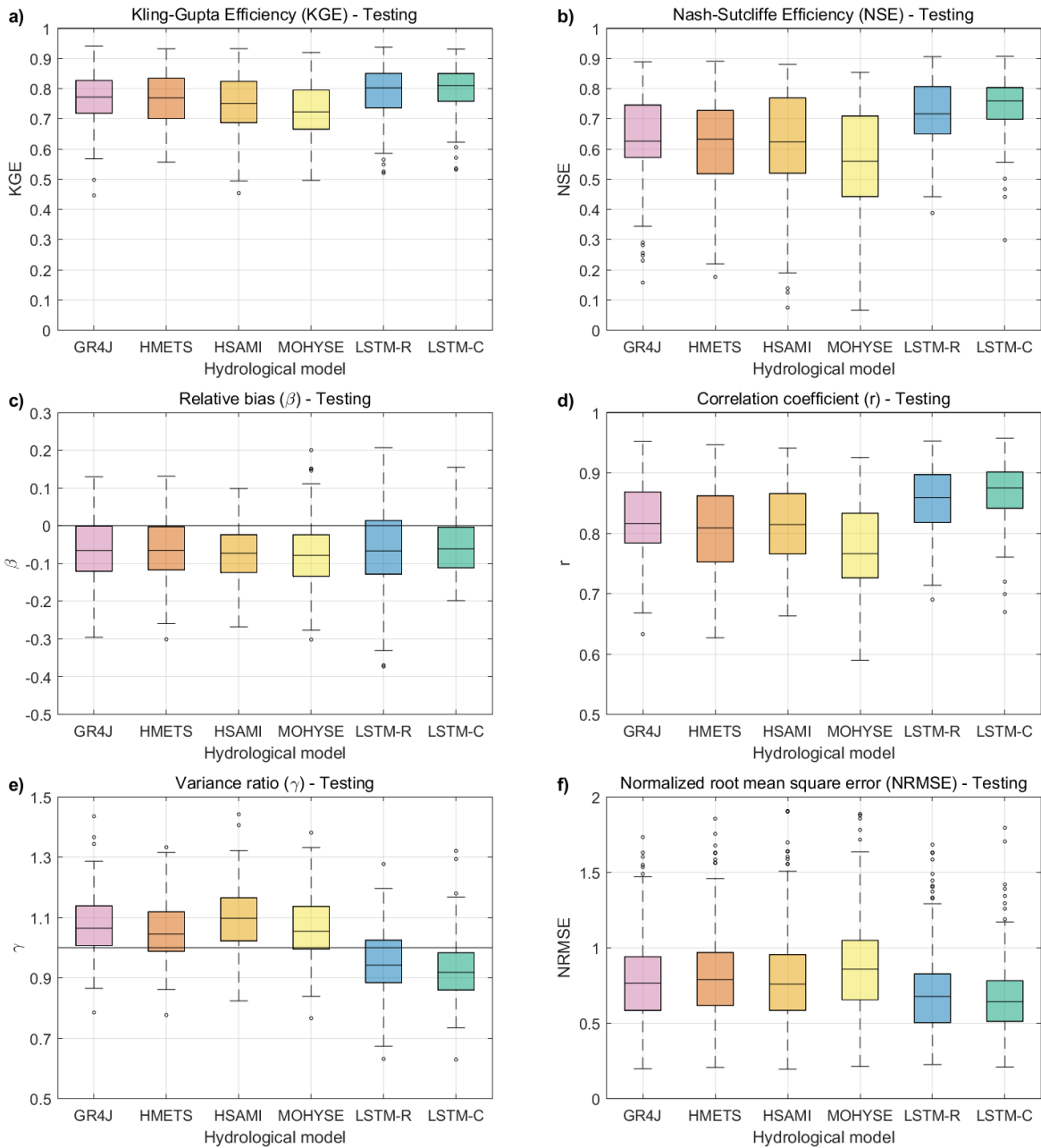
465 Figure 3: Kling-Gupta Efficiency (KGE; a), Nash-Sutcliffe Efficiency (NSE; b), relative bias ( \beta ; c), correlation coefficient ( r ; d), 470 variance ratio ( \gamma ; e), and normalized root mean square error (NRSME; f) metrics over the independent 5-year testing period (2008- 2012).
