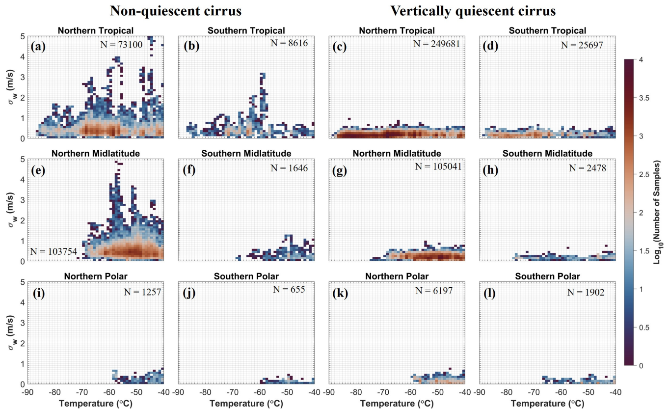
990 Figure 3. Distributions of standard deviations of vertical velocity ( \sigma_w calculated for 10 km spatial scales) at various temperatures, separated by non-quietescent cirrus (two left columns) and vertically quietescent cirrus (two right columns).
