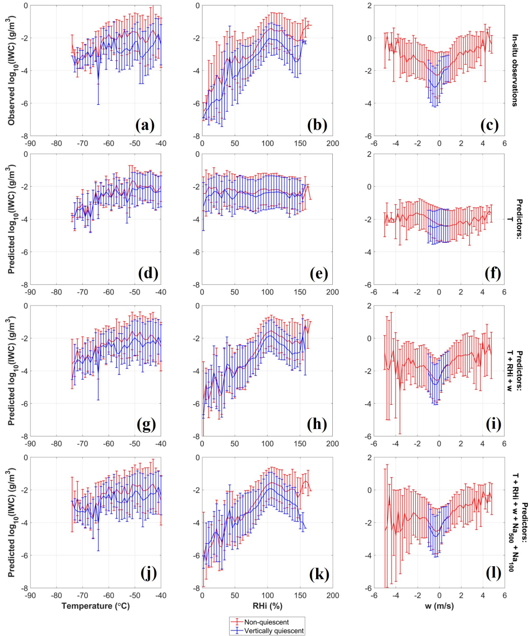
1010 Figure 9. Distributions of \log_{10}\text{IWC} in relation to temperature, RH i , and w in columns 1 – 3, respectively. Various sets of predictors are used in different rows. The solid horizontal lines and the vertical bars represent the geometric means and standard deviations of (a-c) observed and (d-l) predicted \log_{10}\text{IWC} . Red and blue represent results for non-quietest and vertically quietest cirrus, respectively.
