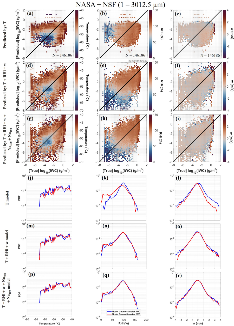
Figure 10. (a-i) Distributions of predicted versus observed \log_{10}\text{IWC} colored coded by the average temperature, RHi, and w in each bin for columns 1 – 3, respectively. (j-r) PDFs of T, RHi, and w , separated by when IWC is underestimated or overestimated by the ML model. Rows 1 and 4 are predicted by T only. Rows 2 and 5 are predicted by T+RHi+w. Rows 3 and 6 are predicted by T+RHi+w+Na 500 +Na 100 .
