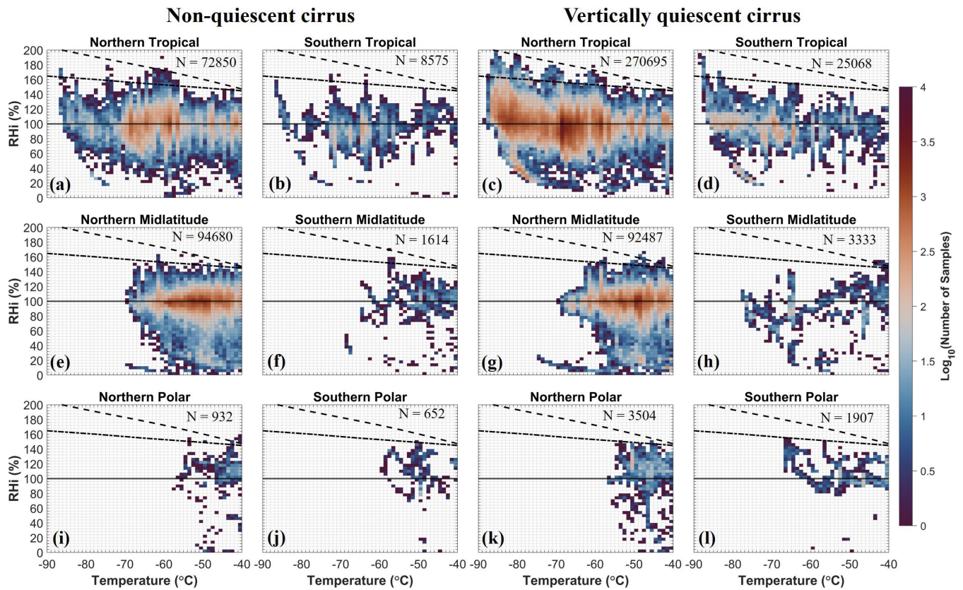
Figure 2. Distributions of RHi at various temperatures in 6 latitudinal bands using the combined NASA and NSF dataset, 925 separated by non-quiescent cirrus (two left columns) and vertically quiescent cirrus (two right columns). Solid black line indicates ice saturation. The dashed black line denotes the liquid saturation threshold. Dash-dotted line represents the homogeneous freezing line based on Koop et al. (2000). Color bars denote logarithmic-scale number of samples.
