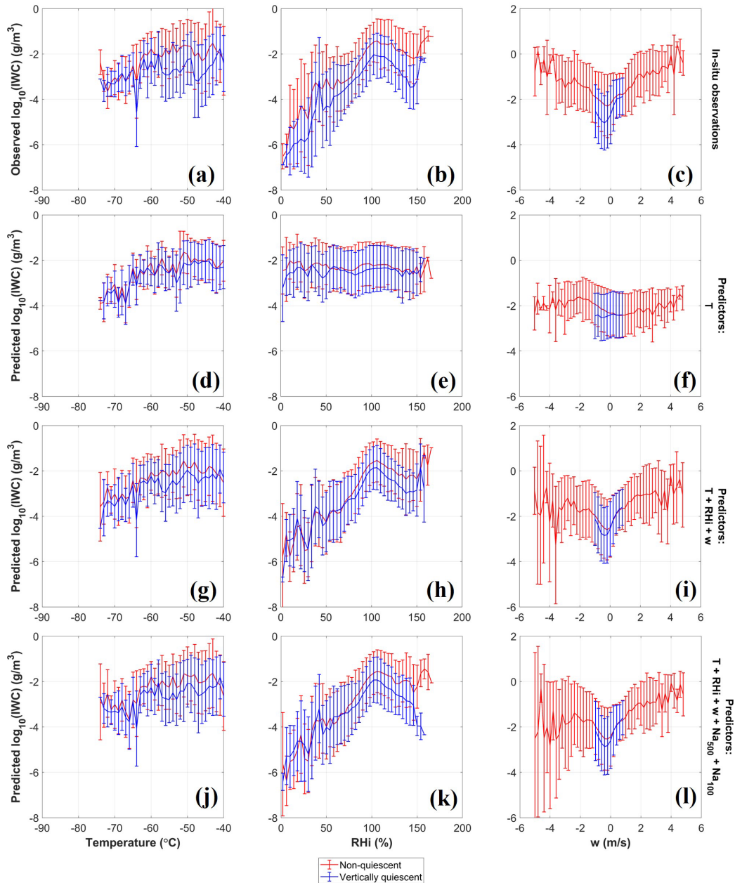
960 Figure 9. Distributions of \log_{10}\text{IWC} in relation to temperature, RH i , and w in columns 1 – 3, respectively. Various sets of predictors are used in different rows. The solid horizontal lines and the vertical bars represent the geometric means and standard deviations of (a-c) observed and (d-l) predicted \log_{10}\text{IWC} . Red and blue represent results for non-quietest and vertically quietest cirrus, respectively.
