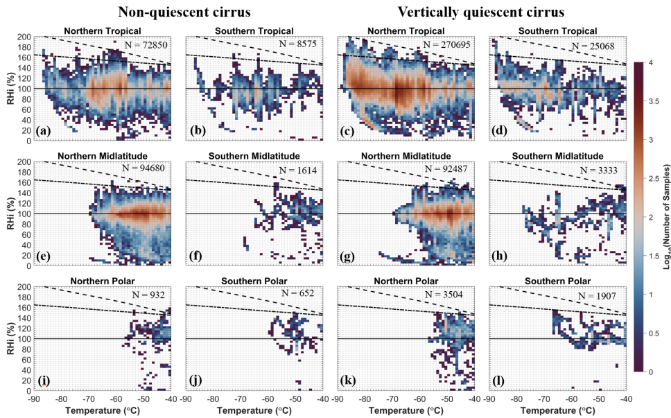
Figure 2. Distributions of RH i at various temperatures in 6 latitudinal bands using the combined NASA and NSF dataset, separated by non-quiescent cirrus (two left columns) and vertically quiescent cirrus (two right columns). Solid black line indicates ice saturation. The dashed black line denotes the liquid saturation threshold. Dash-dotted line represents the homogeneous freezing line based on Koop et al. (2000). Color bars denote logarithmic-scale number of samples.
