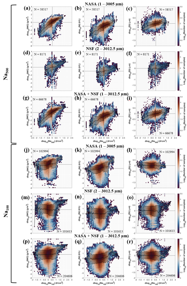
Figure 5. Similar to Figure 4, but for relationships of fluctuations of cirrus properties (i.e., d\log_{10}IWC , d\log_{10}Ni , and d\log_{10}Di ) with respect to d\log_{10}(Na_{500}) in top 3 rows and d\log_{10}(Na_{100}) in bottom 3 rows. Rows 1 and 4 are based on NASA campaigns, rows 2 and 5 are NSF campaigns, and rows 3 and 6 are the combined NASA+NSF campaigns.
