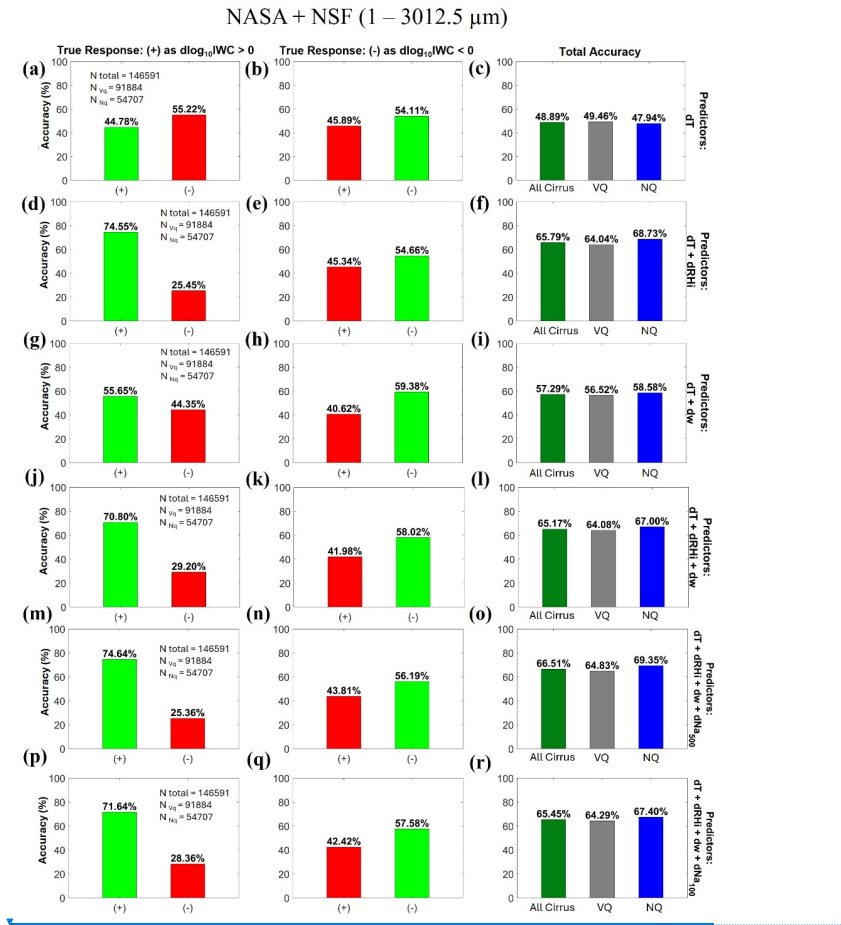
1455 Figure 8. Similar to Figure 7 but predicting whether d\log_{10}IWC is positive (+) or negative (-) for in-cloud conditions. d\log_{10}IWC is calculated relative to the geometric mean of IWC in each 1-degree temperature bin inside cirrus clouds. 1-Hz observations are used in this analysis compared with coarser scales used in Table 2. Columns 1 and 2 represent the scenarios when the real observations show d\log_{10}IWC > 0 and < 0 , respectively. Column 3 shows the overall accuracies for predicting the sign of d\log_{10}IWC in three types of cirrus.
