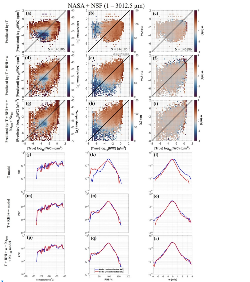
Figure 10. (a-i) Distributions of predicted versus observed \log_{10} IWC colored coded by the average temperature, RH i , and w in each bin for columns 1 – 3, respectively. (j-r) PDFs of T, RH i , and w , separated by when IWC is underestimated or overestimated by the ML model. Rows 1 and 4 are predicted by T only, Rows 2 and 5 are predicted by T+RH i + w . Rows 3 and 6 are predicted by T+RH i + w +Na 500 +Na 100 .
