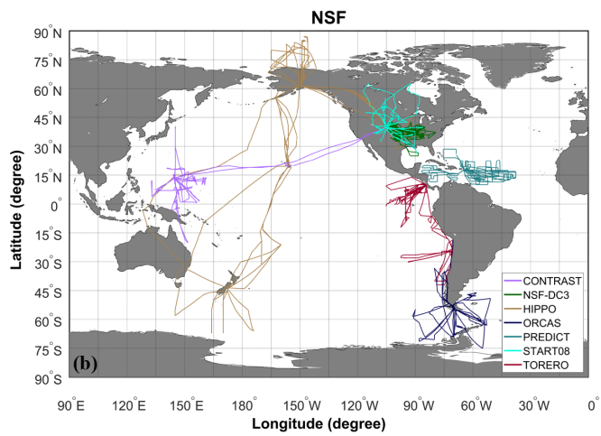
1415 Figure 1. Global maps of research aircraft flight tracks from (a) five NASA campaigns and (b) seven NSF flight campaigns used in this observational study. The entire flight tracks at all temperatures as shown.
