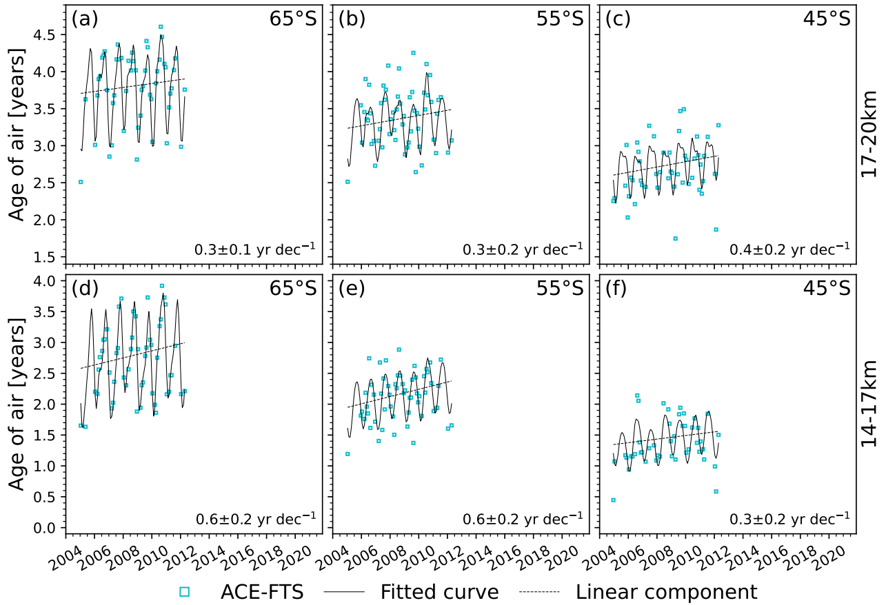
Figure 17. Same as Fig. 14 but for only January 2005 to April 2012.
