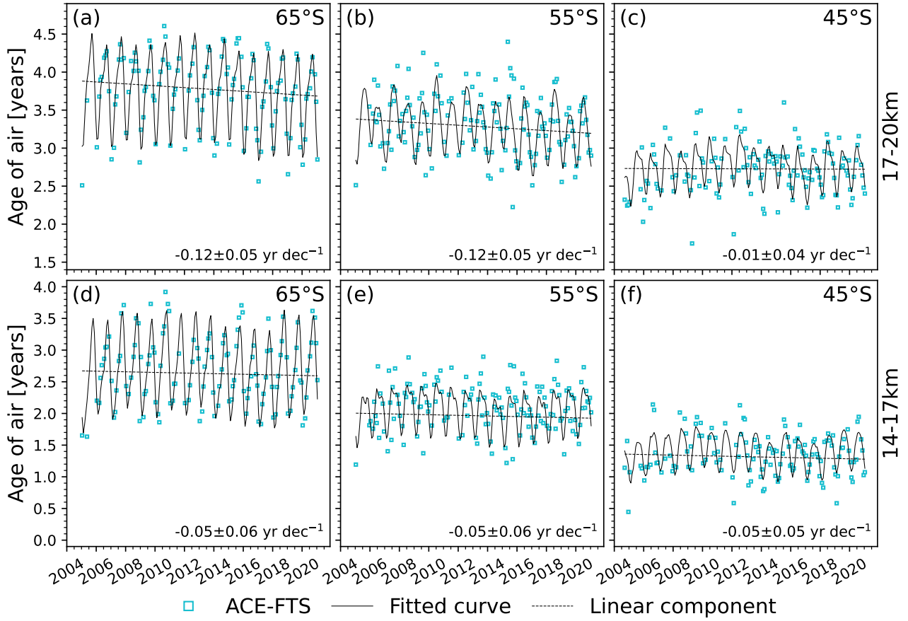
Figure 14. Same as Fig. 13 but for the Southern Hemisphere.
