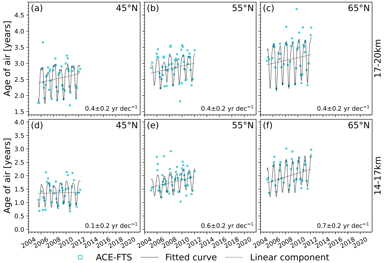
Figure 16. Same as Fig. 13 but for only January 2005 to April 2012.
