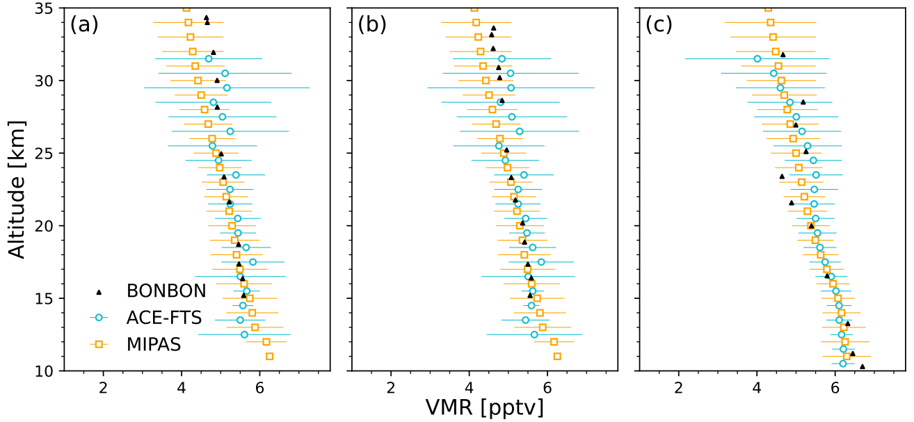
Figure 2. \text{SF}_6 profiles from three BONBON balloon flights (black triangles) on (a) 8 June 2005 (B42) and (b) 25 June 2005 (B43), both over Brazil near 5^\circ S, and on (c) 10 October 2009 over Sweden near 68^\circ N (B45). Also shown are means of \text{SF}_6 profiles from ACE-FTS (blue circles) and MIPAS (orange squares) that are within 90 days and 5^\circ latitude of each BONBON profile. The error bars represent one standard deviation.
