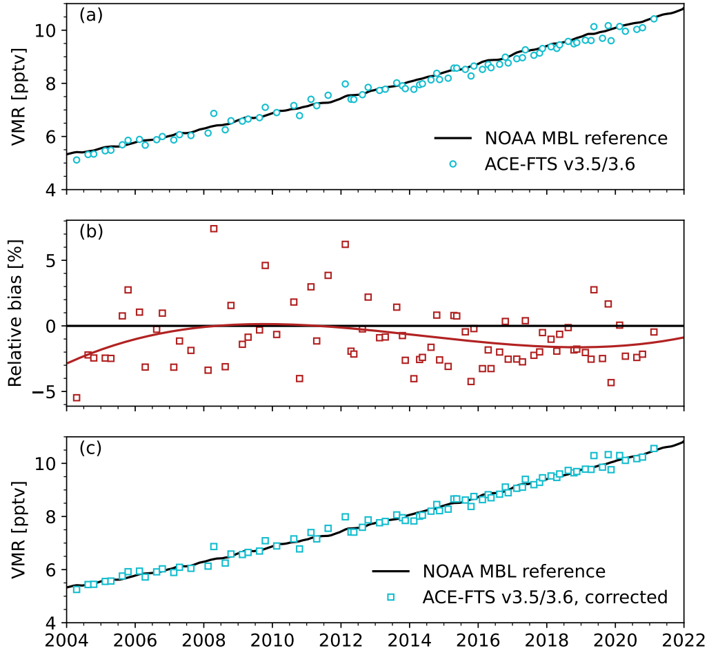
Figure 3. (a) Monthly tropical tropospheric \text{SF}_6 time series from the NOAA MBL reference data (black line) and ACE-FTS (blue circles, see text for definition of tropics and troposphere). (b) Relative difference between the monthly ACE-FTS \text{SF}_6 values and the reference time series (red squares), with a cubic fit to the data (red line). (c) Same as (a) but with the surface correction applied to the ACE-FTS values (blue squares).
