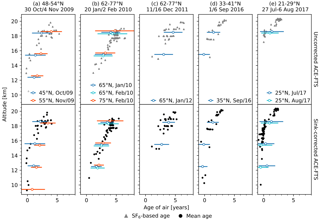
Figure 9. Comparisons between the ACE-FTS age of air dataset and ages based on aircraft in situ measurements taken during the ACE-FTS mission. Each column corresponds to one campaign (a) OB09, (b) K2010, (c) K2011, (d) AMO-16, and (e) AMO-17. See Table 1 for further details. Black dots: mean age of air based on all clock tracers included in the campaign. Grey triangles: age of air based on \text{SF}_6 . Open coloured circles: mean age of air for one bin in the ACE-FTS dataset (top: uncorrected, bottom: sink-corrected). Points for ACE-FTS bins centred on the same altitude are separated vertically for visibility. Error bars show the standard deviation of the age in each bin.
