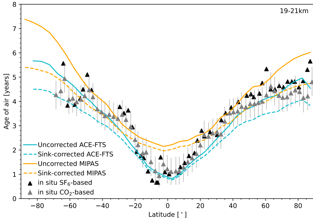
Figure 11. Age of air as a function of latitude, based on in situ measurements of \text{SF}_6 (black triangles), in situ measurements of \text{CO}_2 (grey triangles with 1\sigma error bars), ACE-FTS (blue lines), and MIPAS (orange lines). The dashed lines represent the sink-corrected ages from ACE-FTS and MIPAS. The in situ measurements are aircraft measurements taken between 1992 and 1997 at 19–21 km. The ACE-FTS and MIPAS ages are based on the full datasets, with all measurements taken between 19 and 21 km averaged into 5^\circ latitude bins.
