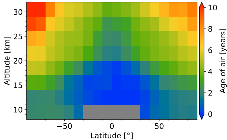
Figure 4. Multi-year zonal mean apparent age of air based on the ACE-FTS \text{SF}_6 dataset (February 2004–February 2021).
