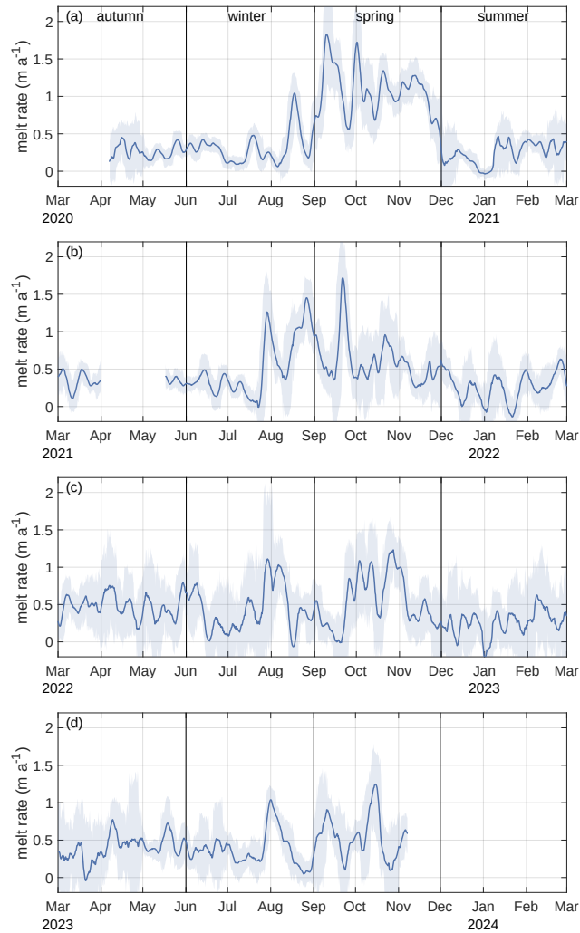
Figure 2. Time series of 7-day average basal melt rate from autumn 2020 to spring 2023 (blue line) with sub-weekly variability represented by the standard deviation (shaded area).
