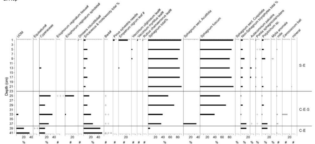
Figure A2. Macrofossil data for peat profiles in transect 1. Unrecognized organic matter (UOM), and plant species or species group are presented as well as remains of mites, Cenococcum , and mineral content.
