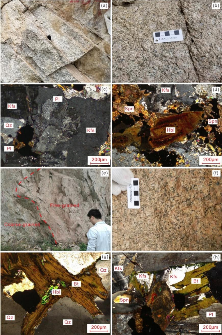
125 Figure 3: Representative field photographs and photomicrographs of the LP (a-d) and XP (e-h) in the western section of North Qinling Orogen. Kfs = K-feldspar, Pl = Plagioclase, Bt = biotite, Qz = Quartz, Hbl = Hornblende, Spn = Sphene.
