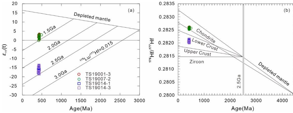
Figure 9: Age versus \varepsilon_{\text{Hf}}(t) diagram (a) and Age versus ^{176}\text{Hf}/^{177}\text{Hf} diagram (b) of the LP and XP in the western section of North Qinling Orogen.
