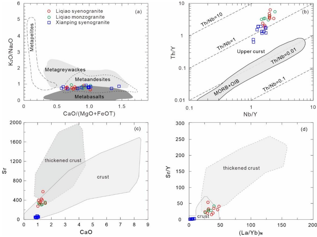
Figure 10: The source region diagrams of the LP and XP in the western section of North Qinling Orogen: (a) molar \text{K}_2\text{O}/\text{Na}_2\text{O} versus molar \text{CaO}/(\text{MgO}+\text{FeO}^T) (Altherr and Siebel 2002); (b) \text{Nb}/\text{Y} versus \text{Th}/\text{Y} (Boztuğ et al. 2007); (c) \text{CaO} versus \text{Sr} (He et al. 2011); (d) (\text{La}/\text{Yb})_N versus \text{Sr}/\text{Y} (He et al. 2011).
