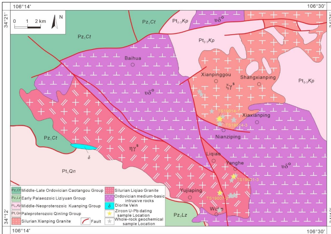
105 Figure 2: Geological map showing the LP and XP in the western section of North Qinling Orogen (Pei et al. 2004; Xu et al. 2012).
