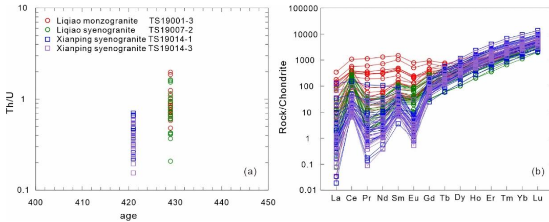
200 Figure 5: Zircons U-Pb age-Th/U (a) and Chondrite-normalized REE patterns (b) diagram of the LP and XP in the western 205 section of North Qinling Orogen. The chondrite and Primitive Mantle values are from Sun and McDonough (1989).
