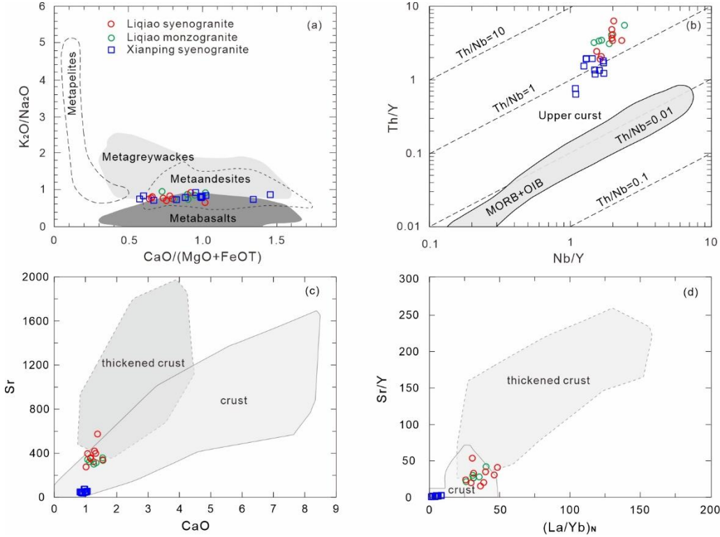
Figure 10: The source region diagrams of the LP and XP in the western section of North Qinling Orogen: (a) molar \text{K}_2\text{O}/\text{Na}_2\text{O} versus molar \text{CaO}/(\text{MgO}+\text{FeO}^{\text{T}}) (Altherr and Siebel 2002); (b) Nb/Y versus Th/Y (Boztuğ et al. 2007); (c) CaO versus Sr (He et al. 2011); (d) (\text{La}/\text{Yb})_{\text{N}} versus Sr/Y (He et al. 2011).
