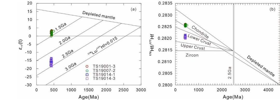
Figure 9: Age versus ε Hf (t) diagram (a) and Age versus 176 Hf/ 177 Hf diagram (b) of the LP and XP in the western section of North Qinling Orogen.
