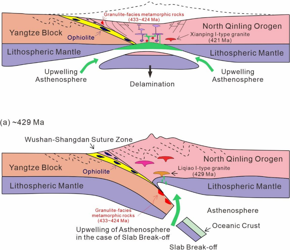
Figure 13: Schematics geodynamic and petrogenetic model illustrating the evolution of the western section of the North Qinling Orogen at ca. 429 Ma and 421Ma, and the generation of the LP (a) and XP (b) during Late Silurian.
