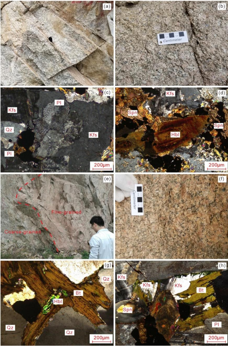
125 Figure 3: Representative field photographs and photomicrographs of the LP and XP in the western section of North Qinling Orogen. Kfs = K-feldspar, Pl = Plagioclase, Bt = biotite, Qz = Quartz, Hbl = Hornblende, Spn = Sphene.
